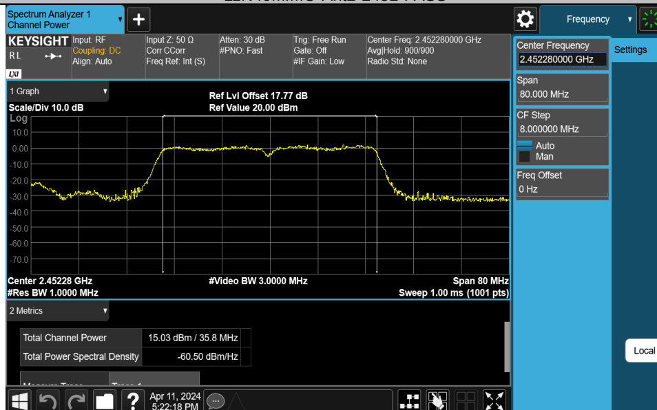
11N40MIMO-Ant2-2452-PASS
