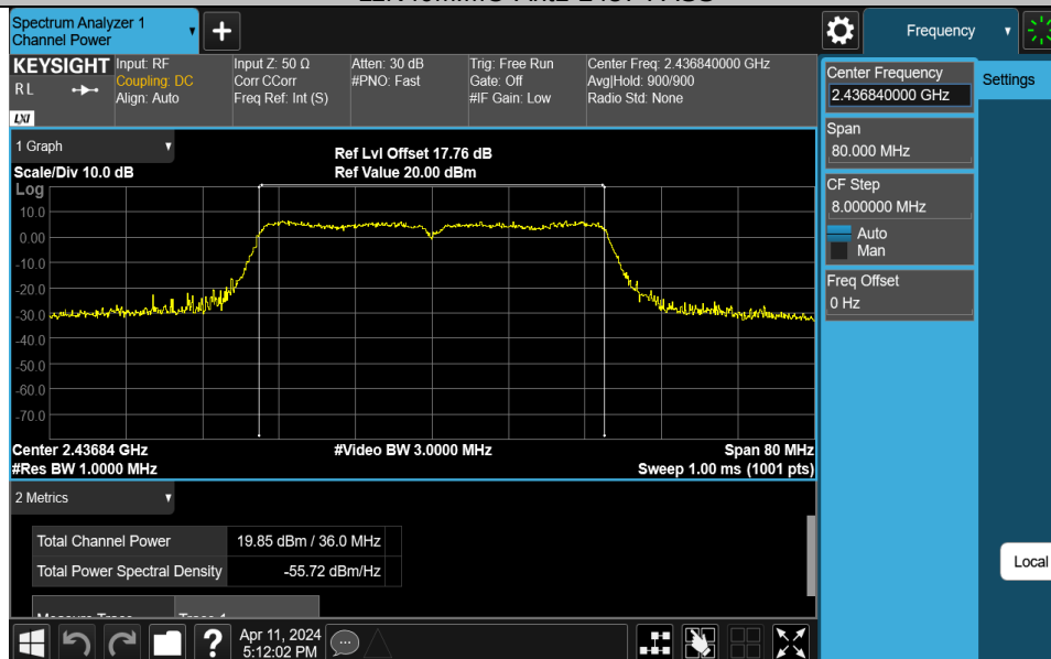
11N40MIMO-Ant2-2437-PASS
