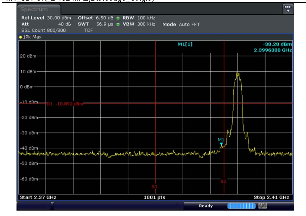
M1 8DPSK 2 402 MHz(Bandedge_Single)
