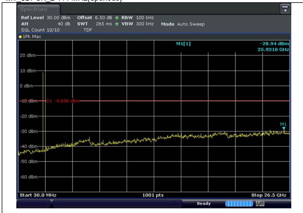
M1 8DPSK 2 441 MHz(Spurious)
