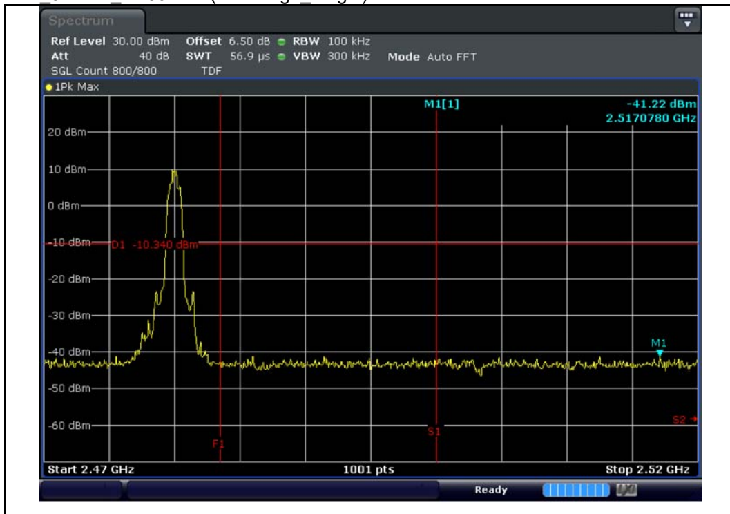
M1 8DPSK 2 480 MHz(Bandedge_Single)
