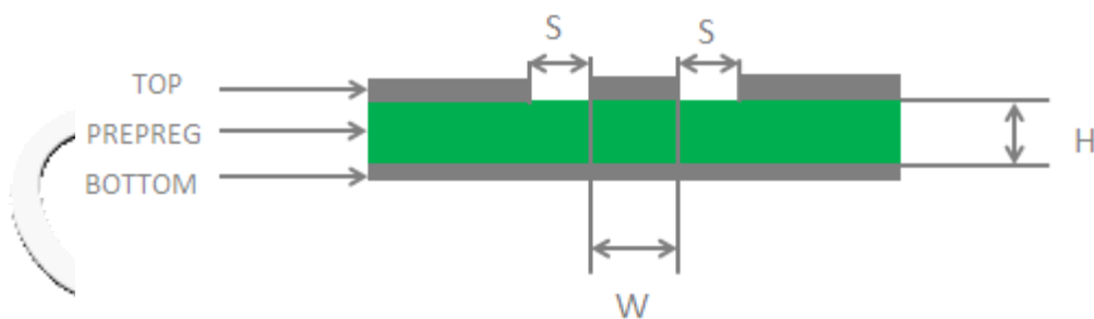
Figure 4-2 Coplanar waveguide structure of two-layer PCB
