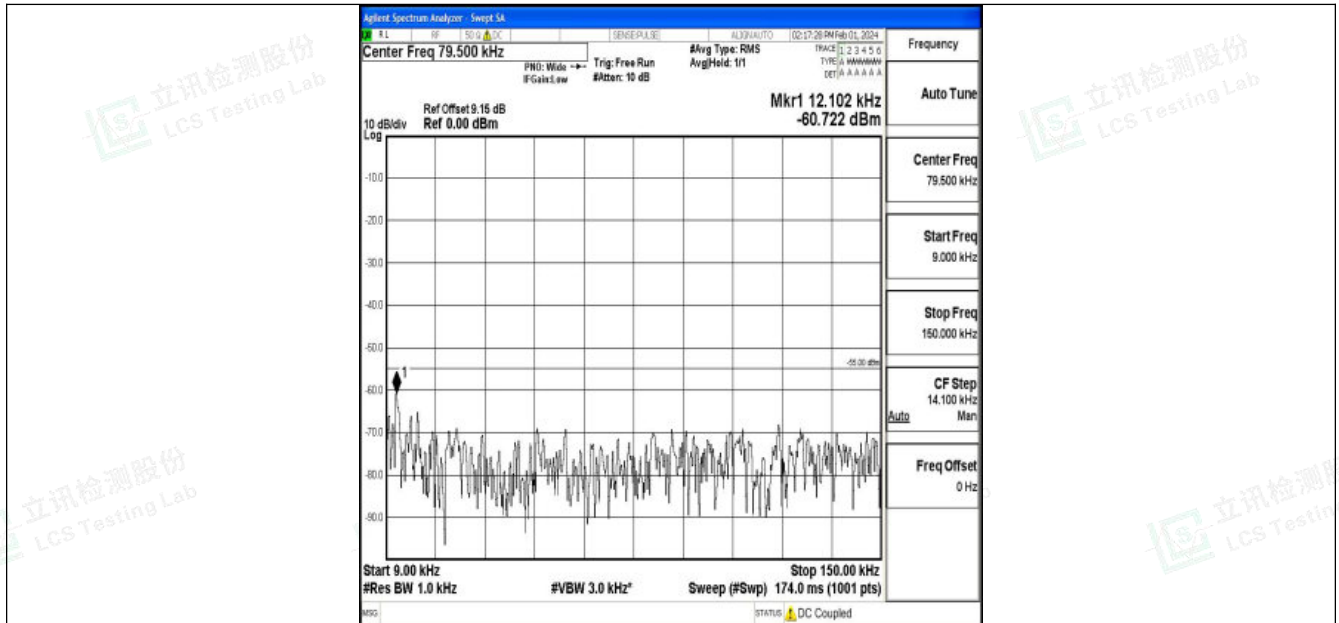
Band7_5MHz_QPSK_20775_1RB#0_0.009~0.15_0.009~0.15
