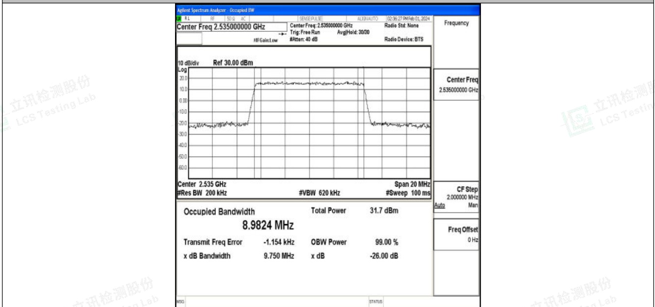
Band7-10MHz-16QAM-21100-50RB#0-PASS
