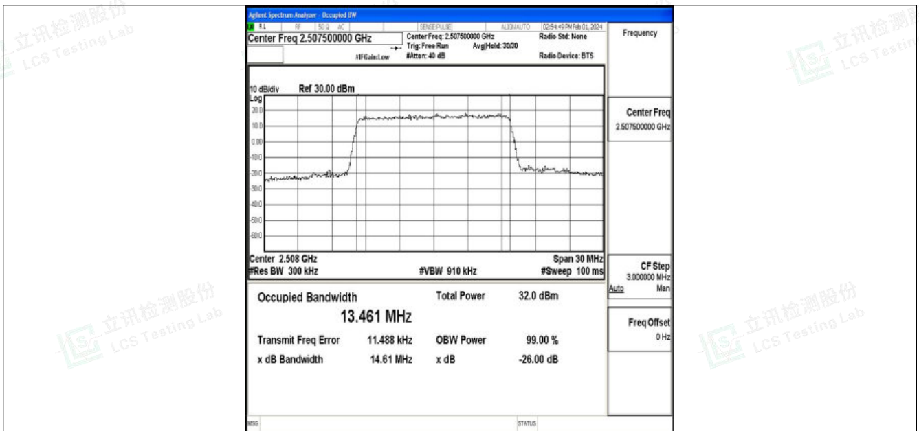
Band7-15MHz-QPSK-20825-75RB#0-PASS
