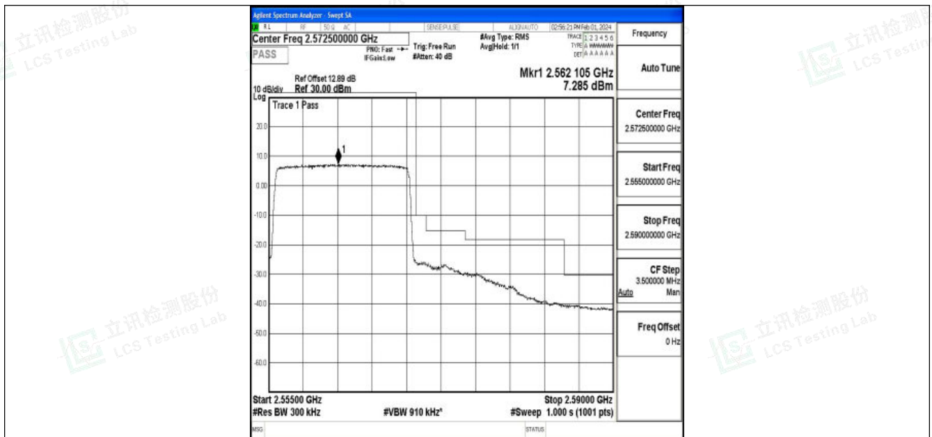
Band7_15MHz_16QAM_21375_75RB#0
