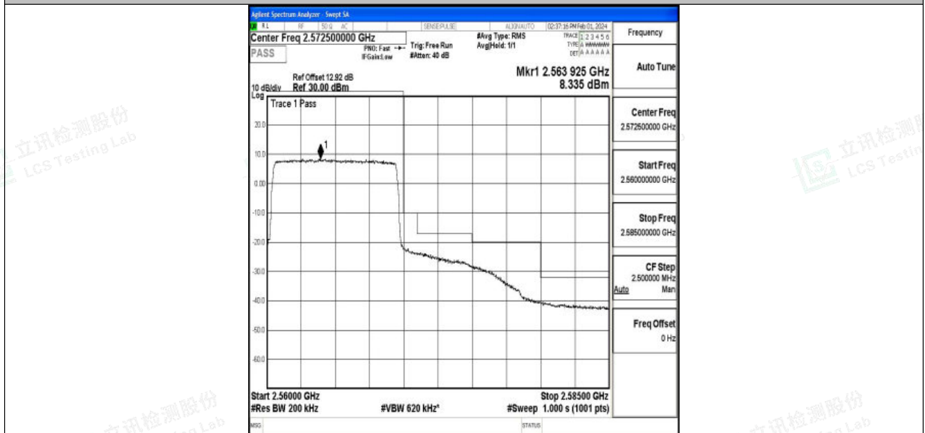
Band7_10MHz_QPSK_21400_50RB#0
