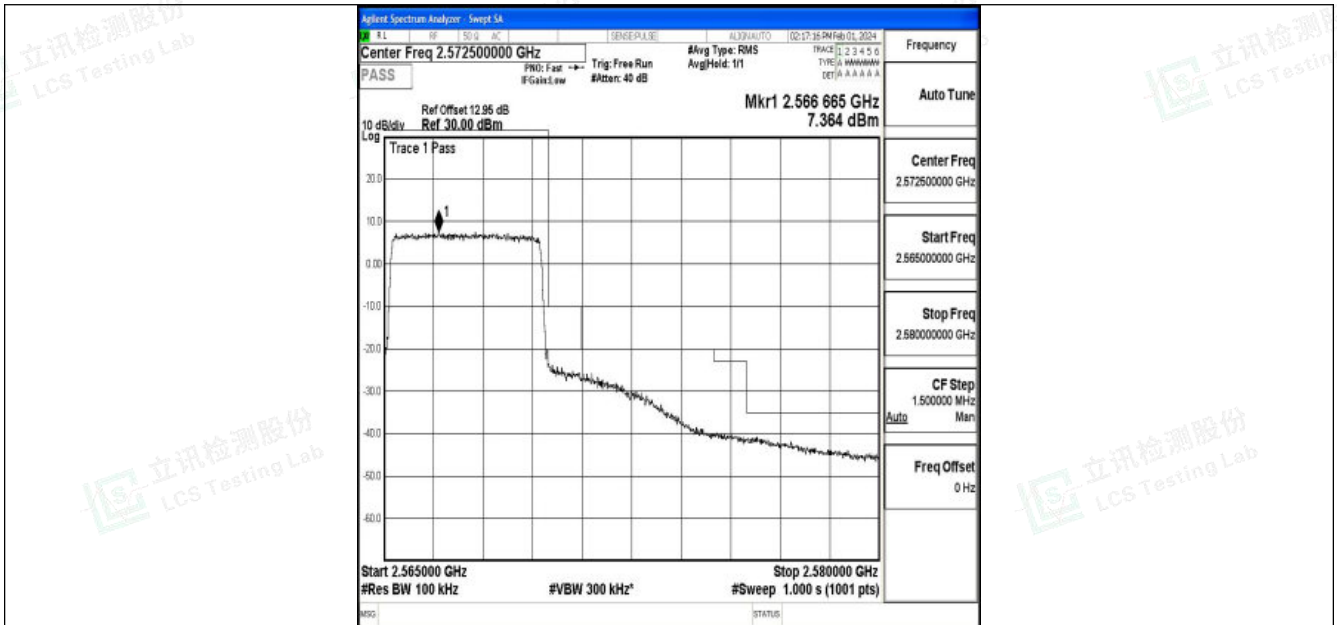
Band7_5MHz_16QAM_21425_25RB#0
