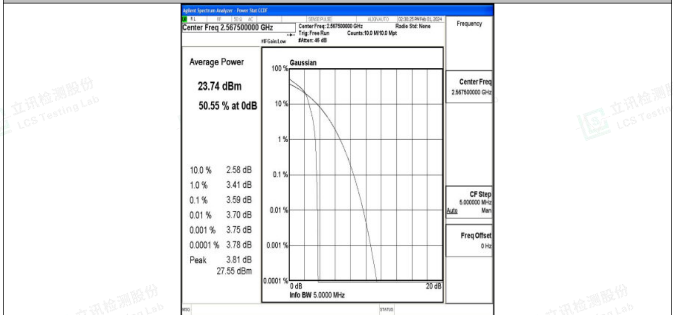
Band7-5MHz-16QAM-21425-1RB#0-PASS
