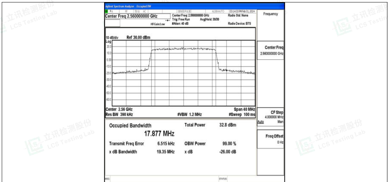
Band7-20MHz-QPSK-21350-100RB#0-PASS
