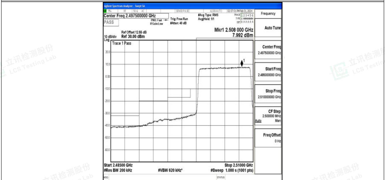
Band7_10MHz_QPSK_20800_50RB#0
