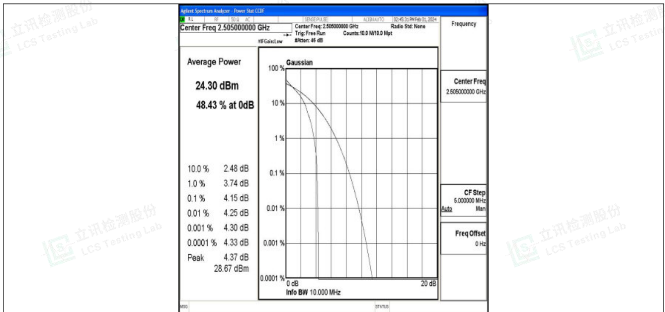
Band7-10MHz-QPSK-20800-1RB#0-PASS
