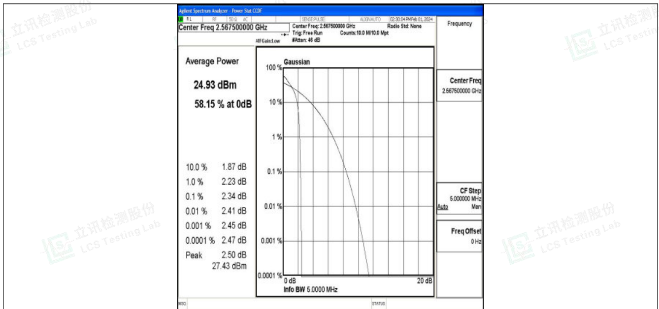
Band7-5MHz-QPSK-21425-1RB#0-PASS
