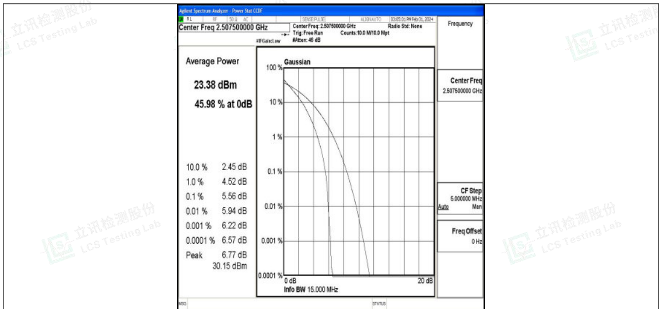
Band7-15MHz-QPSK-20825-75RB#0-PASS
