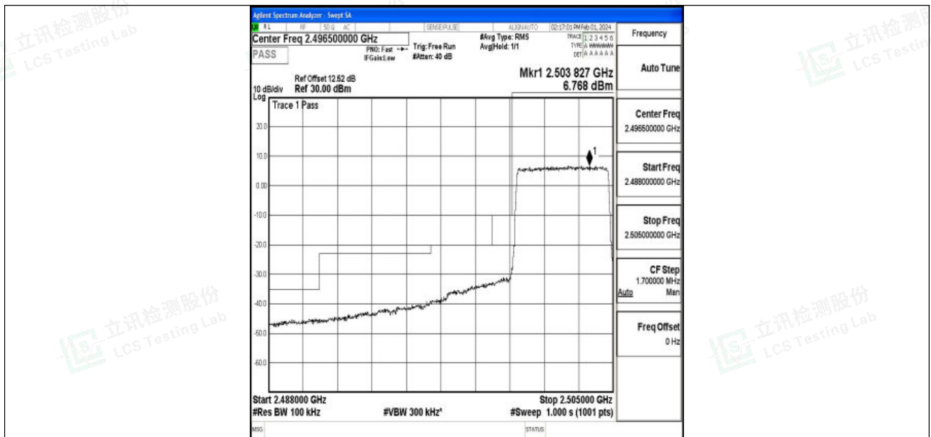
Band7_5MHz_16QAM_20775_25RB#0
