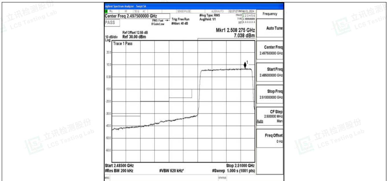
Band7_10MHz_16QAM_20800_50RB#0
