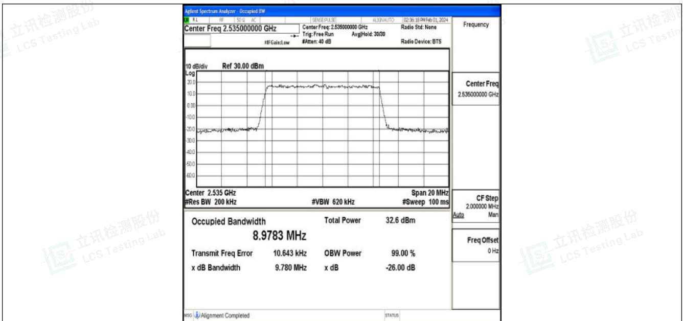
Band7-10MHz-QPSK-21100-50RB#0-PASS
