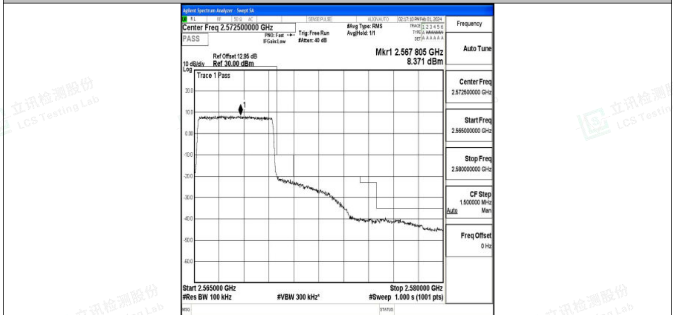
Band7_5MHz_QPSK_21425_25RB#0
