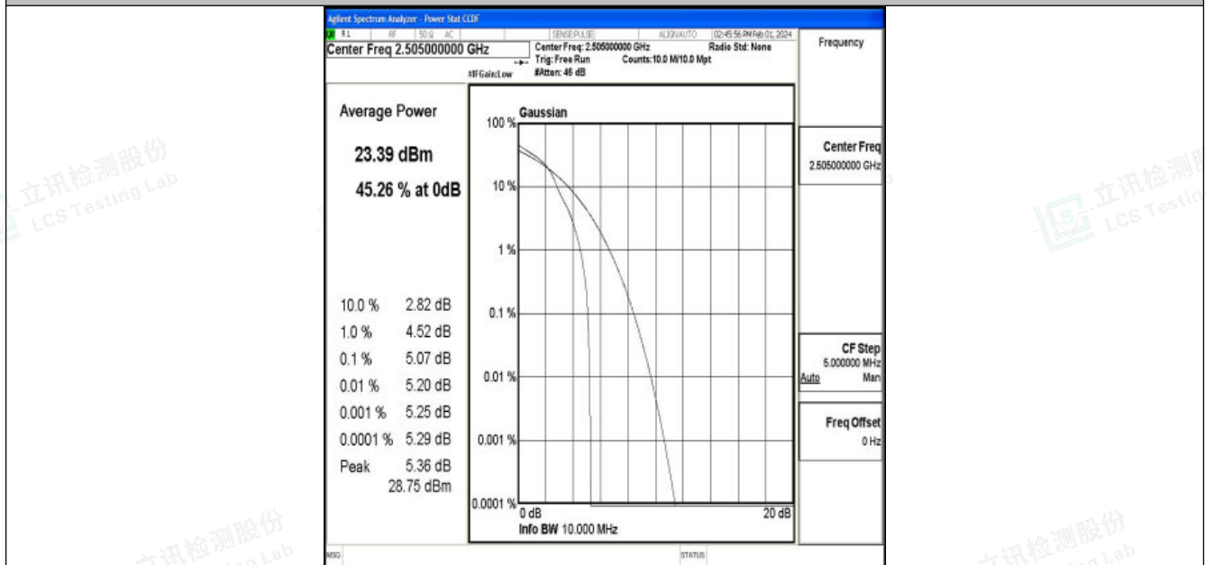
Band7-10MHz-16QAM-20800-1RB#0-PASS
