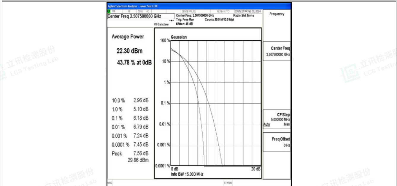
Band7-15MHz-16QAM-20825-75RB#0-PASS
