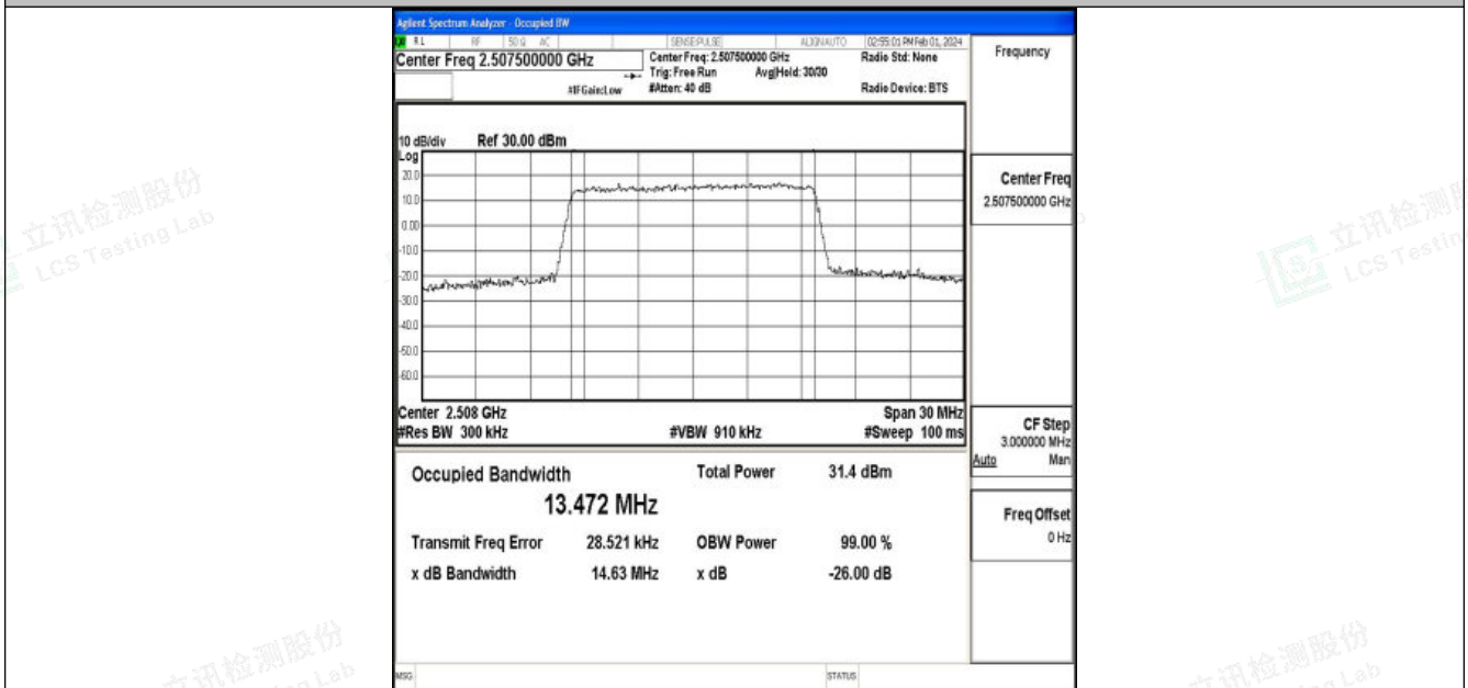
Band7-15MHz-16QAM-20825-75RB#0-PASS
