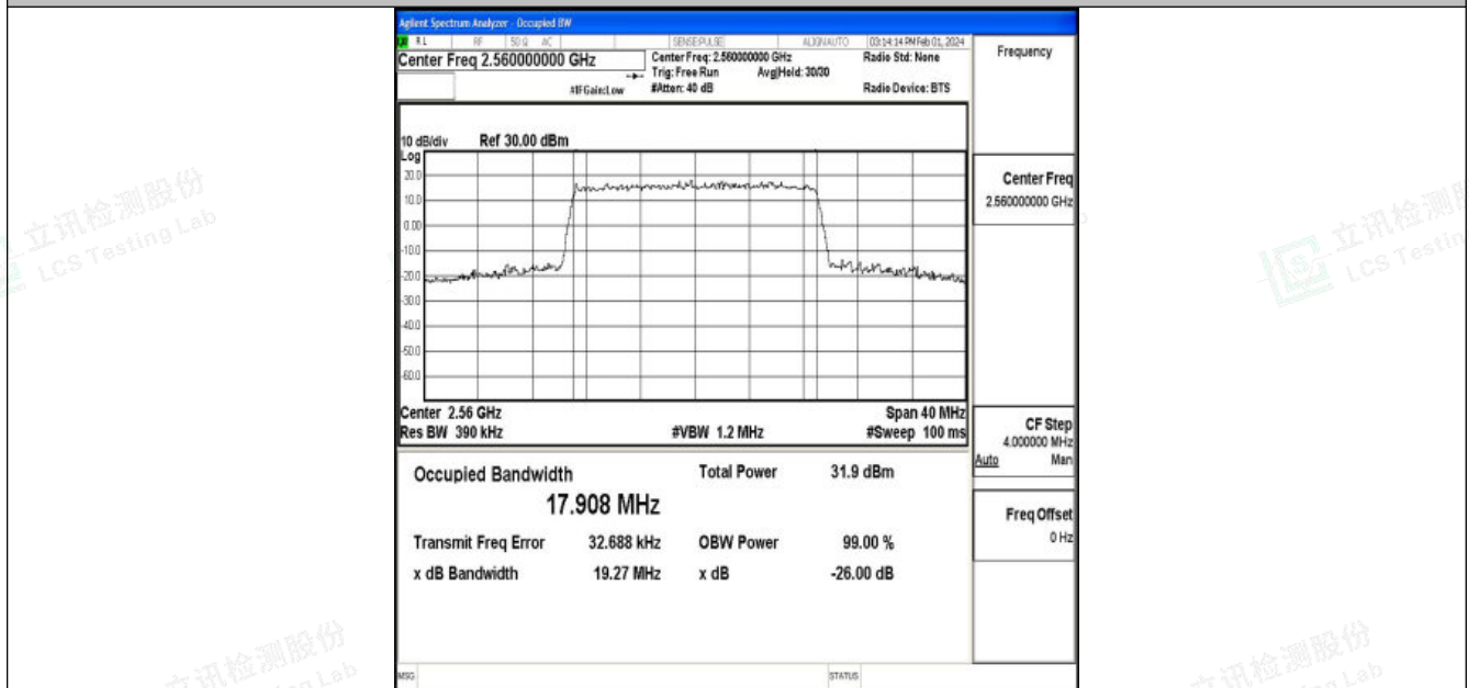
Band7-20MHz-16QAM-21350-100RB#0-PASS
