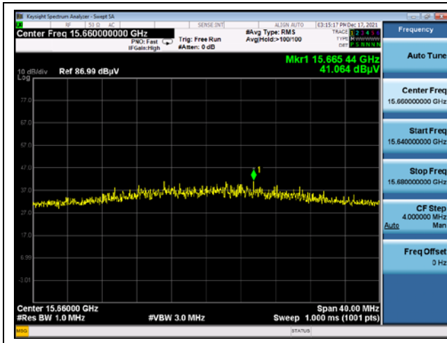
Middle channel 3 rd harmonic (Peak) - Band 1
