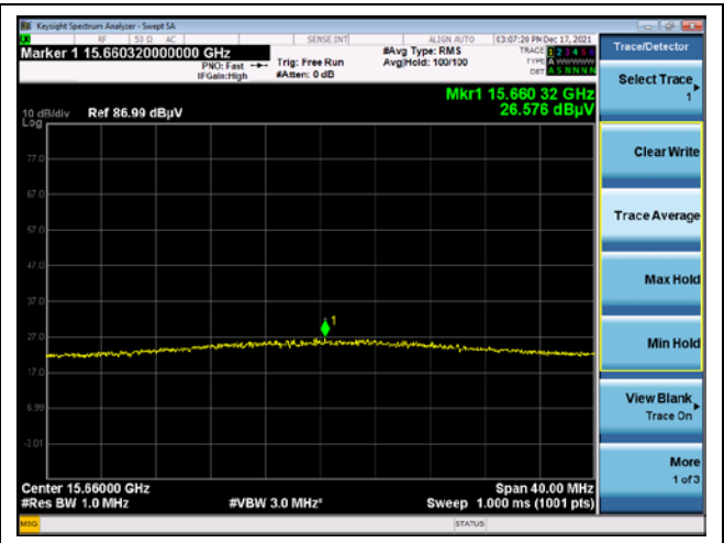
Middle channel 3 rd harmonic (Average) - Band 1
