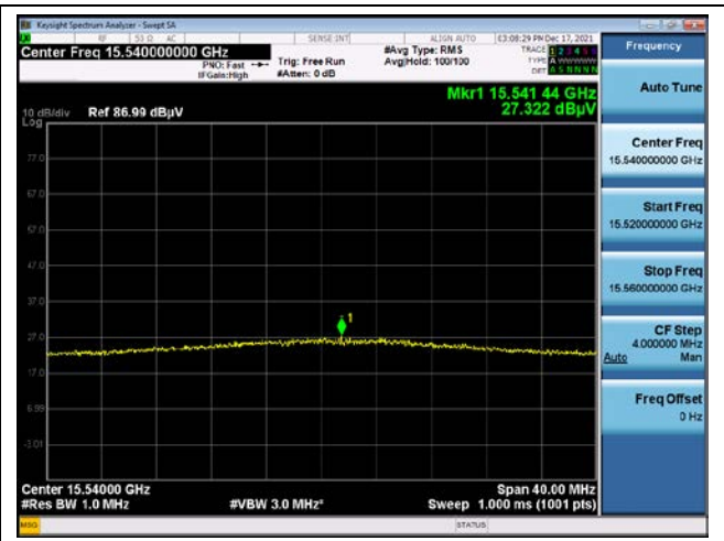
Low channel 3 rd harmonic (Average) - Band 1
