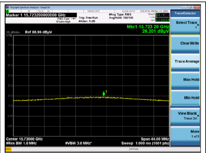
High channel 3 rd harmonic (Average) - Band 1
