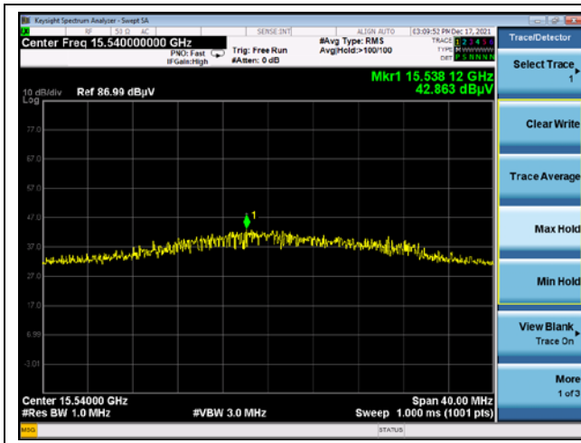
Low channel 3 rd harmonic (Peak) - Band 1
