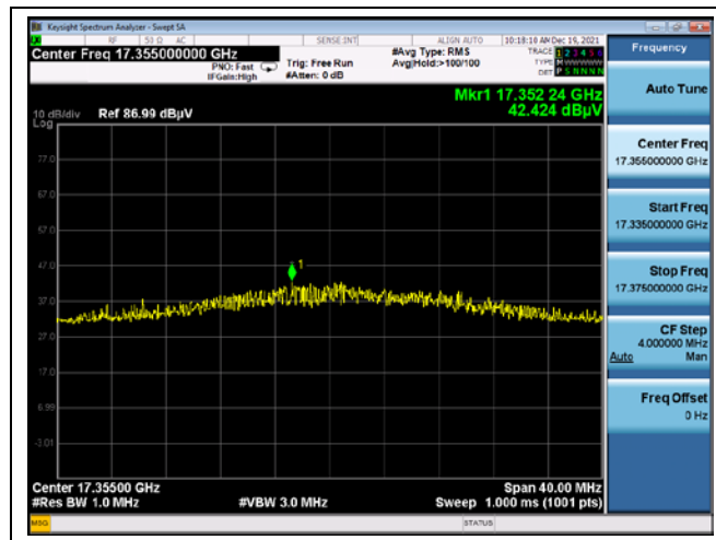
Middle channel 3 rd harmonic (Peak) - Band 3
