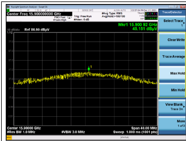
Middle channel 3 rd harmonic (Peak) - Band 2A
