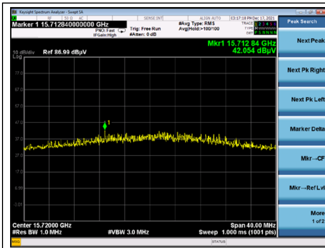
High channel 3 rd harmonic (Peak) - Band 1
