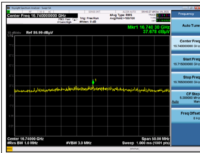
Middle channel 3 rd harmonic (Peak) - Band 2C
