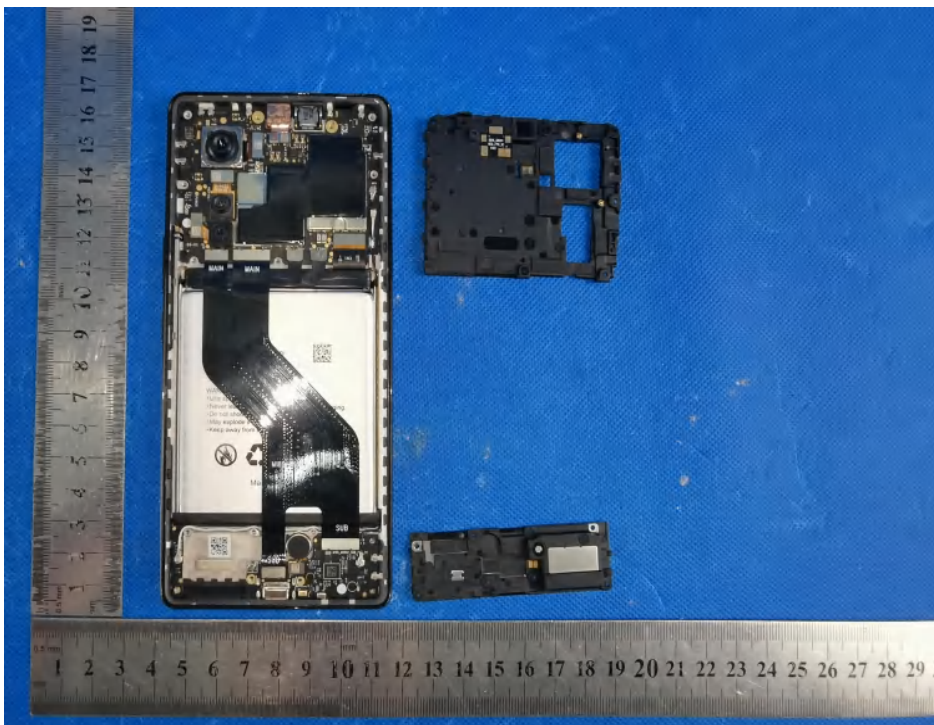
OPEN VIEW OF EUT(FIGURE 2)
