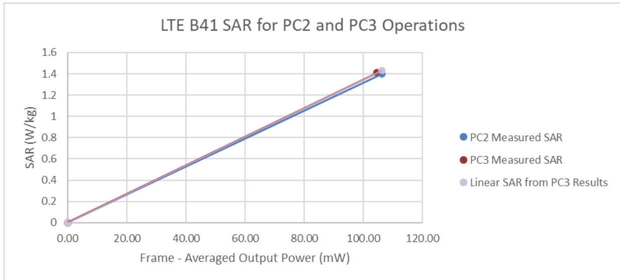
Figure 13-12 LTE Band 41 Antenna I ULCA Phablet Linearity
