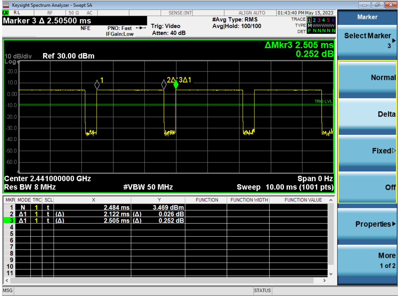
Figure 9-8 Bluetooth Low Energy Antenna 1 Transmission Plot
