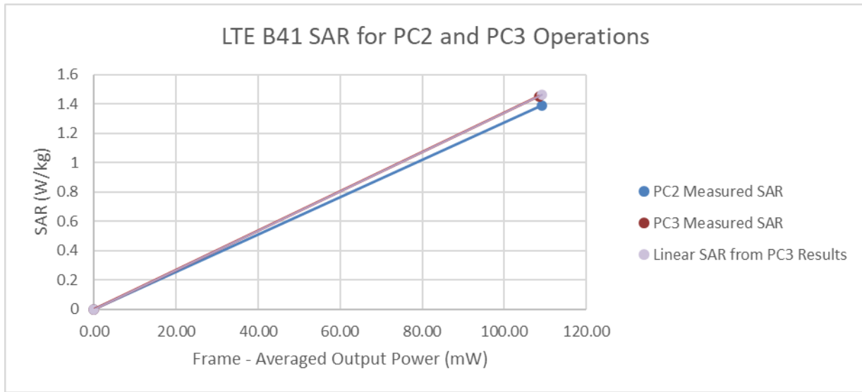
Figure 13-11 LTE Band 41 Antenna I Phablet Linearity
