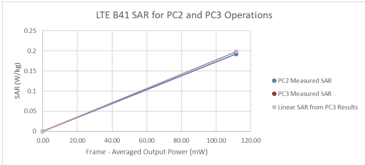
Figure 13-5 LTE Band 41 Antenna I Body-Worn Linearity
