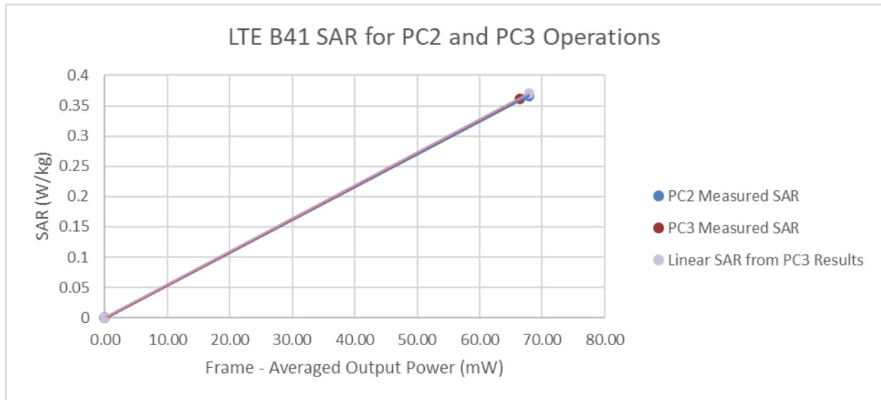
Figure 13-8 LTE Band 41 Antenna B ULCA Hotspot Linearity
