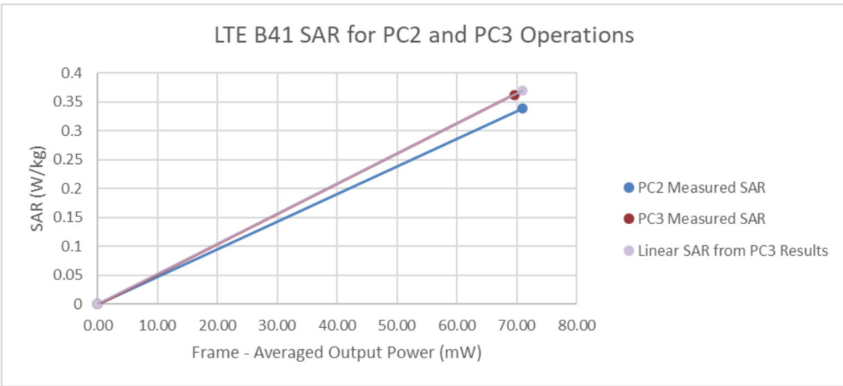
Figure 13-7 LTE Band 41 Antenna B Hotspot Linearity
