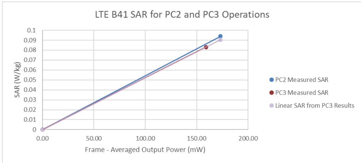
Figure 13-3 LTE Band 41 Antenna B Body-Worn Linearity
