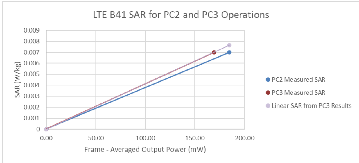
Figure 13-2 LTE Band 41 Antenna B ULCA Head Linearity
