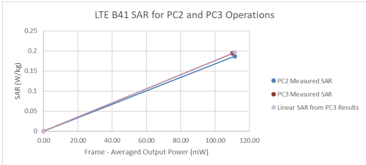
Figure 13-6 LTE Band 41 Antenna I ULCA Body-Worn Linearity
