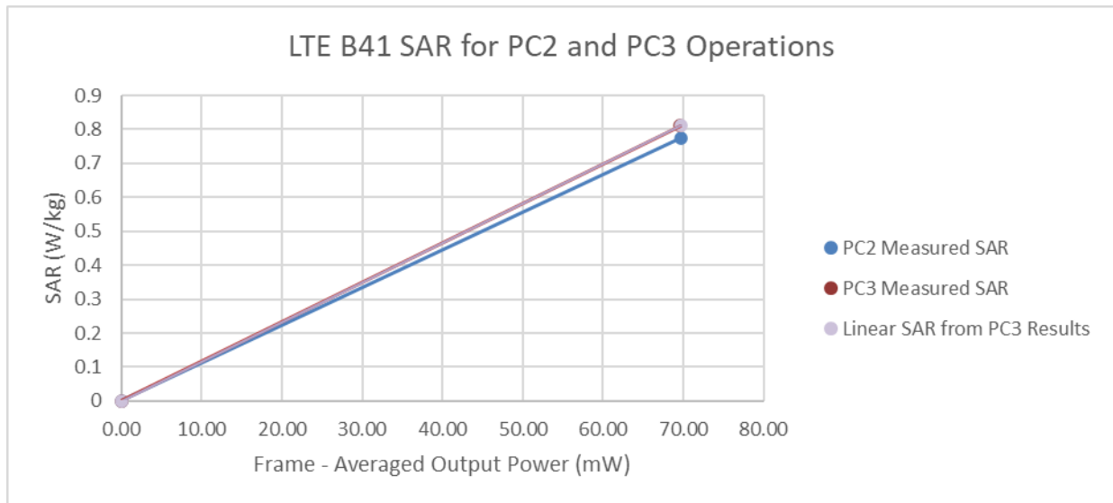
Figure 13-9 LTE Band 41 Antenna I Hotspot Linearity
