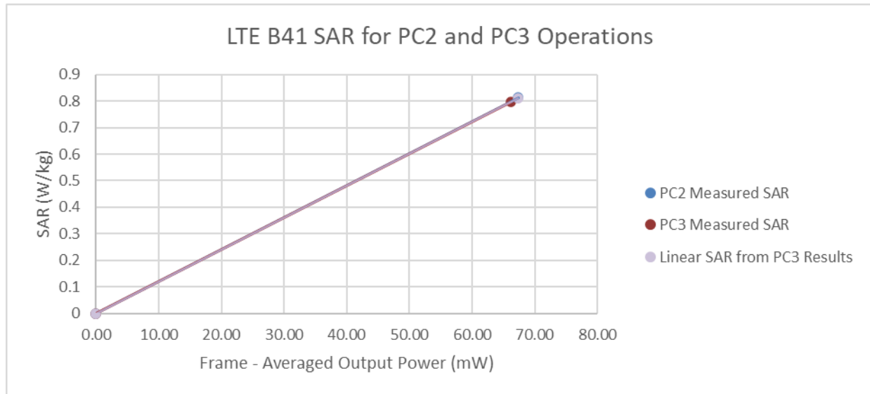
Figure 13-10 LTE Band 41 Antenna I ULCA Hotspot Linearity
