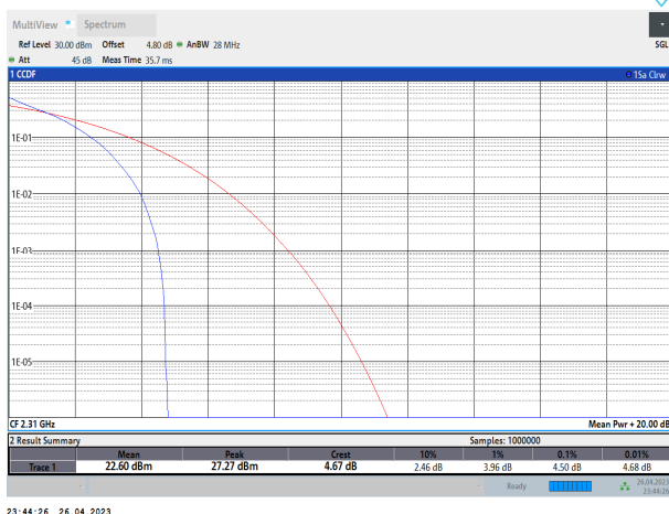
Band30-10MHz-QPSK-27710-50RB#0
