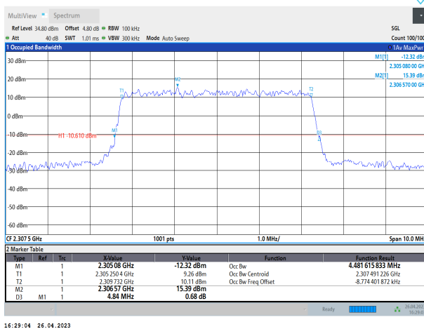
Band30-5MHz-QPSK-27710-25RB#0
