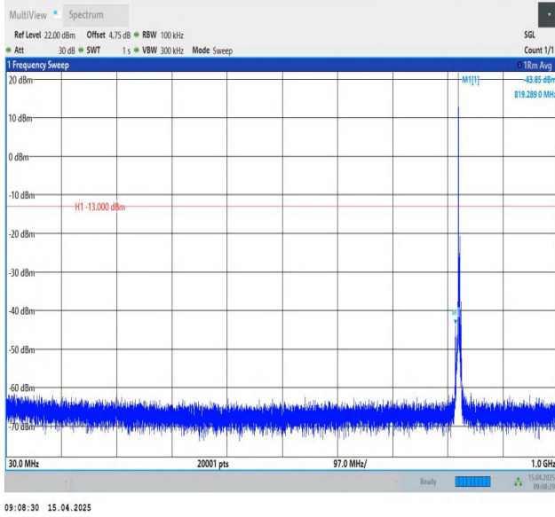
Band26(824-849)-3MHz-QPSK-26805-1RB#0-30~1000-PASS
