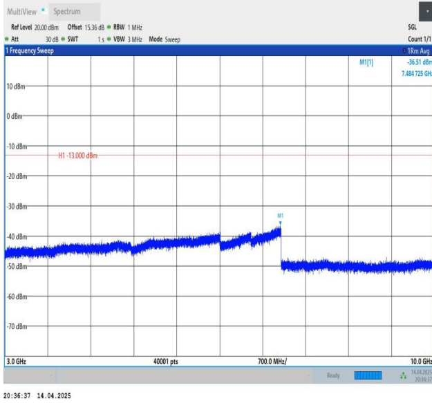
Band26(824-849)-3MHz-QPSK-26915-1RB#0-3000~10000-PASS
