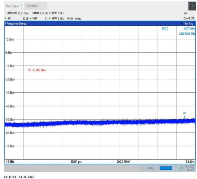
Band26(824-849)-5MHz-QPSK-27015-1RB#0-1000~3000-PASS
