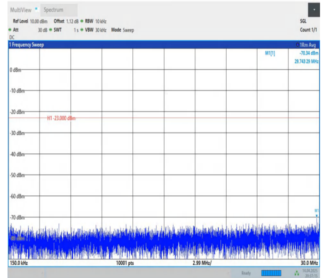
Band26(824-849)-3MHz-QPSK-27025-1RB#0-0.15~30-PASS
