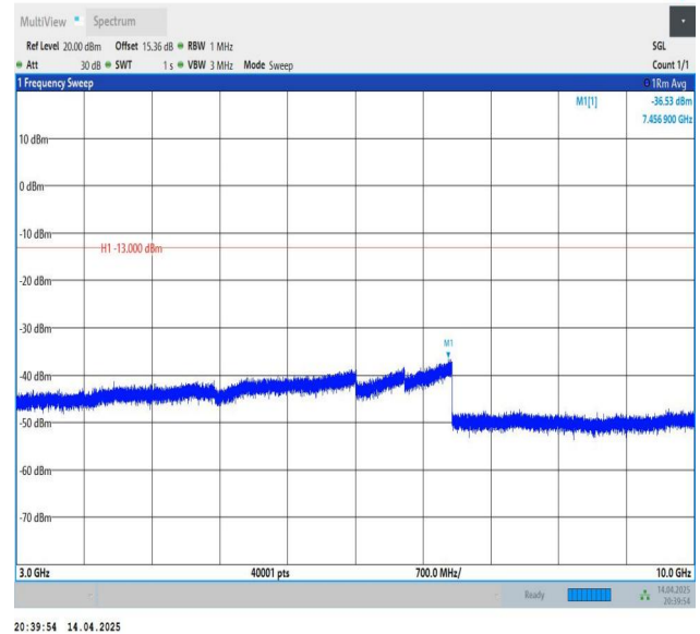
Band26(824-849)-5MHz-QPSK-26915-1RB#24-3000~10000-PASS
