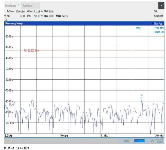
Band26(824-849)-3MHz-QPSK-26805-1RB#14-0.009~0.15-PASS
