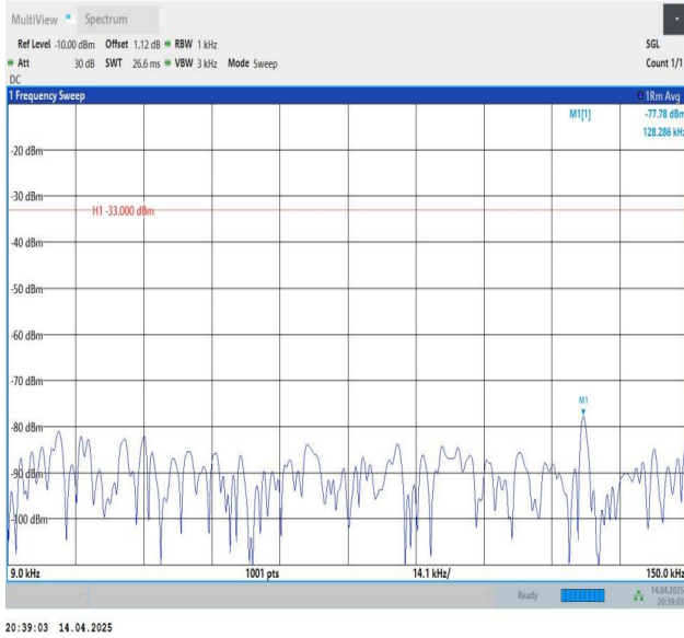
Band26(824-849)-5MHz-QPSK-26915-1RB#0-0.009~0.15-PASS
