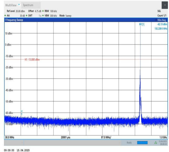
Band26(824-849)-3MHz-QPSK-26915-1RB#14-30~1000-PASS
