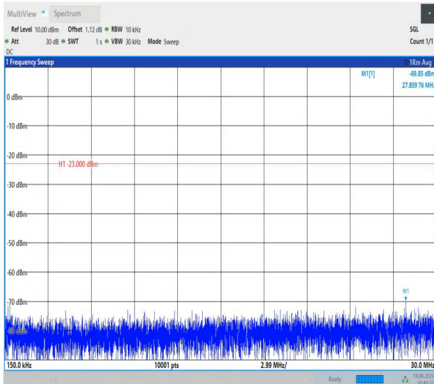
Band26(824-849)-5MHz-QPSK-27015-1RB#24-0.15~30-PASS
