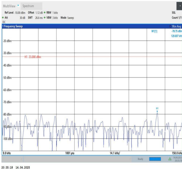
Band26(824-849)-3MHz-QPSK-26805-1RB#0-0.009~0.15-PASS
