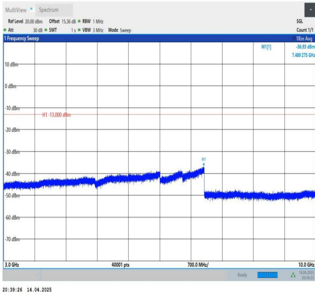
Band26(824-849)-5MHz-QPSK-26915-1RB#0-3000~10000-PASS
