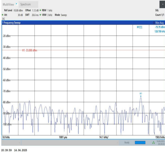
Band26(824-849)-5MHz-QPSK-27015-1RB#0-0.009~0.15-PASS
