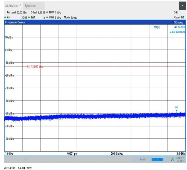
Band26(824-849)-1.4MHz-QPSK-27033-1RB#0-1000~3000-PASS
