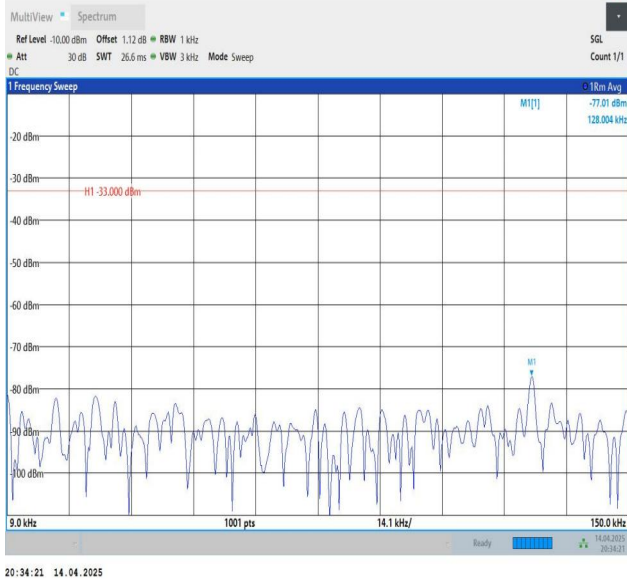
Band26(824-849)-1.4MHz-QPSK-27033-1RB#0-0.009~0.15-PASS
