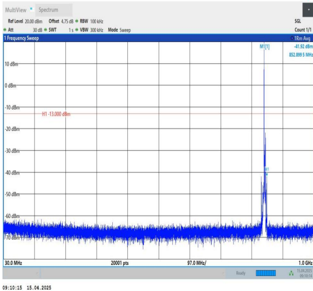
Band26(824-849)-5MHz-QPSK-27015-1RB#0-30~1000-PASS
