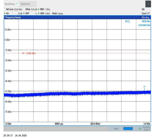
Band26(824-849)-5MHz-QPSK-26915-1RB#0-1000~3000-PASS
