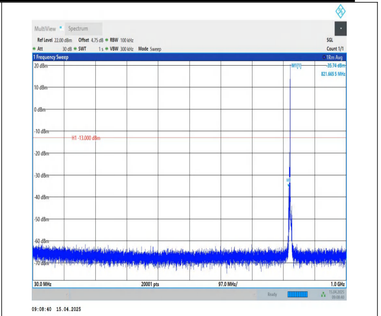
Band26(824-849)-3MHz-QPSK-26805-1RB#14-30~1000-PASS
