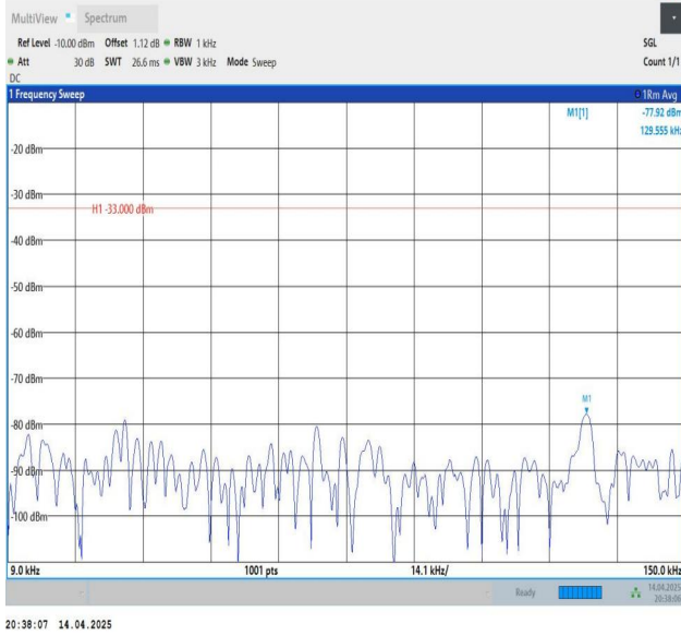
Band26(824-849)-5MHz-QPSK-26815-1RB#0-0.009~0.15-PASS
