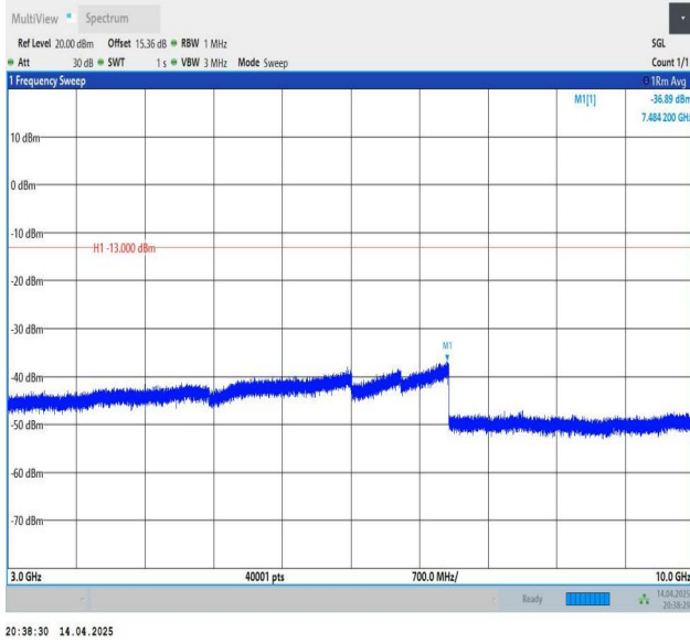
Band26(824-849)-5MHz-QPSK-26815-1RB#0-3000~10000-PASS
