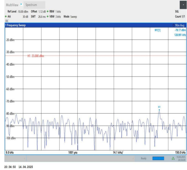
Band26(824-849)-1.4MHz-QPSK-27033-1RB#5-0.009~0.15-PASS
