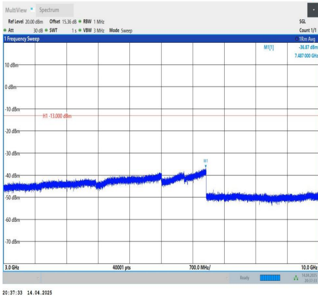
Band26(824-849)-3MHz-QPSK-27025-1RB#0-3000~10000-PASS
