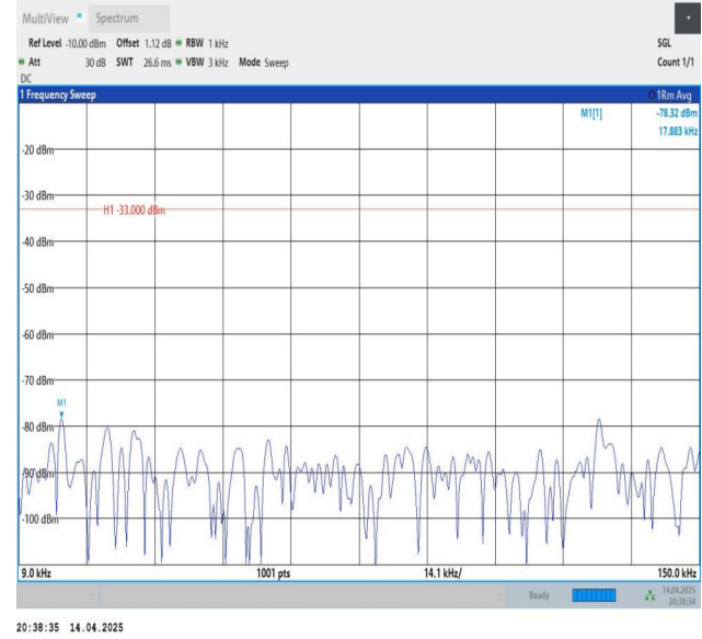
Band26(824-849)-5MHz-QPSK-26815-1RB#24-0.009~0.15-PASS
