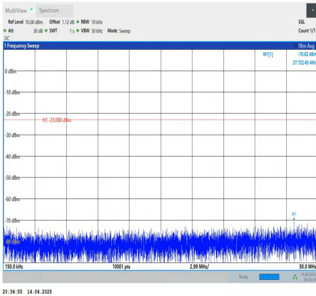
Band26(824-849)-1.4MHz-QPSK-27033-1RB#5-0.15~30-PASS
