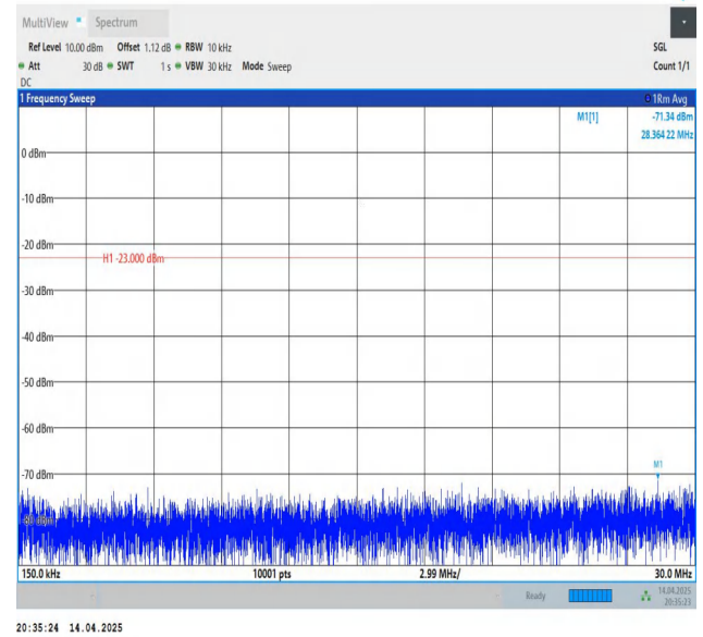
Band26(824-849)-3MHz-QPSK-26805-1RB#0-0.15~30-PASS
