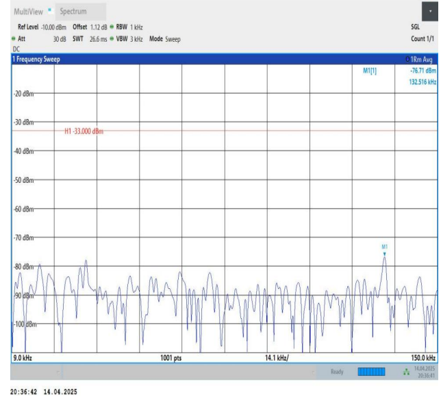
Band26(824-849)-3MHz-QPSK-26915-1RB#14-0.009~0.15-PASS
