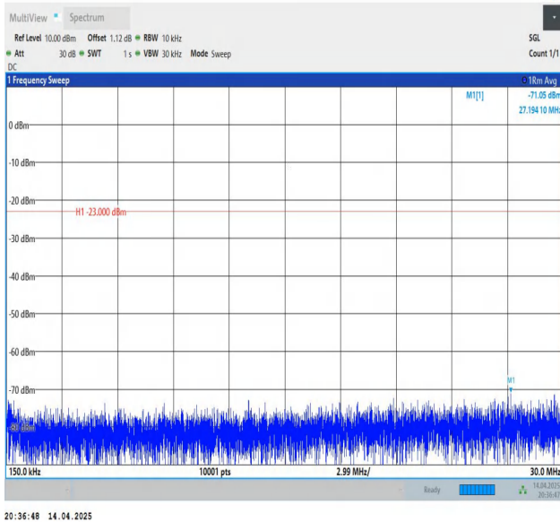
Band26(824-849)-3MHz-QPSK-26915-1RB#14-0.15~30-PASS
