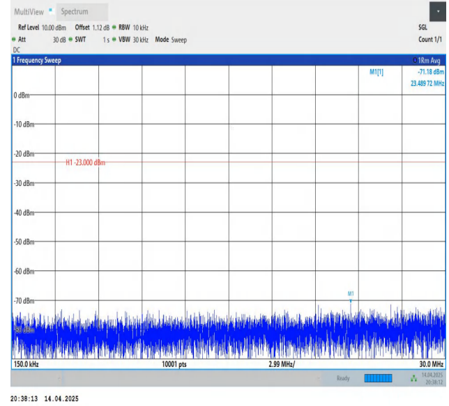
Band26(824-849)-5MHz-QPSK-26815-1RB#0-0.15~30-PASS
