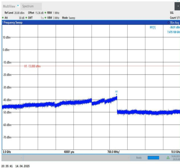
Band26(824-849)-3MHz-QPSK-26805-1RB#0-3000~10000-PASS
