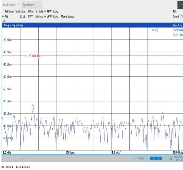
Band26(824-849)-3MHz-QPSK-26915-1RB#0-0.009~0.15-PASS
