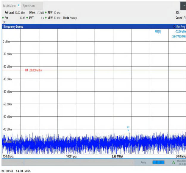
Band26(824-849)-5MHz-QPSK-26815-1RB#24-0.15~30-PASS
