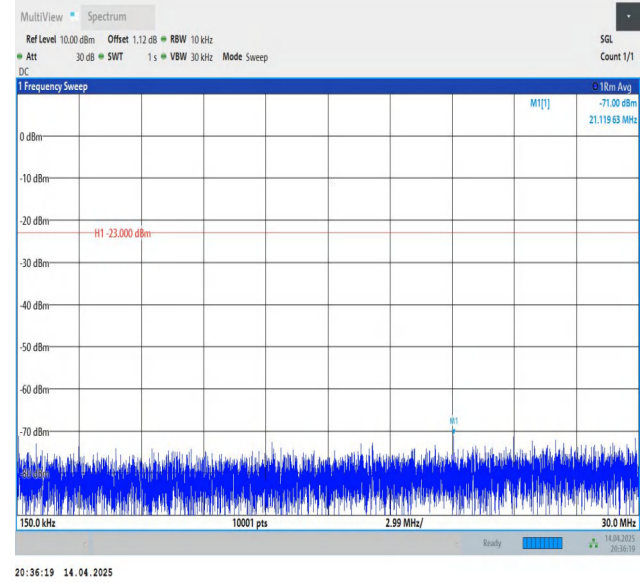
Band26(824-849)-3MHz-QPSK-26915-1RB#0-0.15~30-PASS
