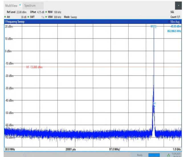
Band26(824-849)-5MHz-QPSK-27015-1RB#24-30~1000-PASS
