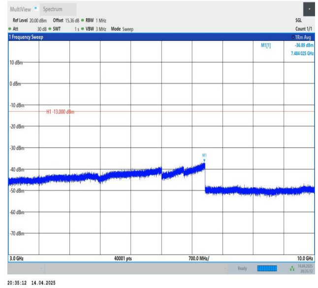
Band26(824-849)-1.4MHz-QPSK-27033-1RB#5-3000~10000-PASS S
