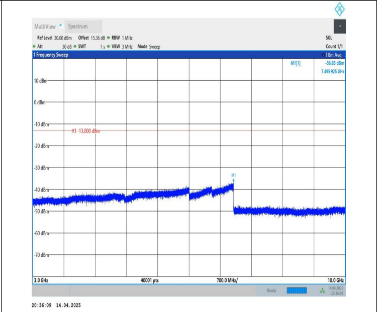
Band26(824-849)-3MHz-QPSK-26805-1RB#14-3000~10000-PASS
