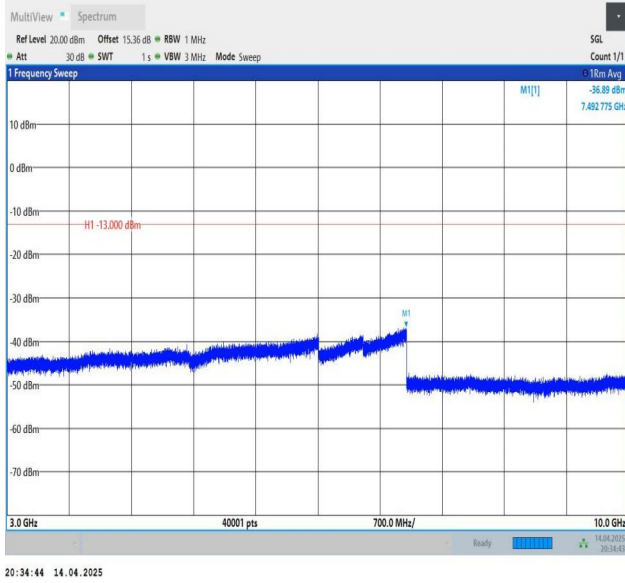
Band26(824-849)-1.4MHz-QPSK-27033-1RB#0-3000~10000-PASS S
