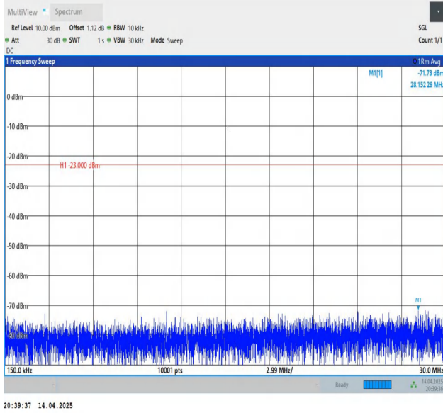
Band26(824-849)-5MHz-QPSK-26915-1RB#24-0.15~30-PASS
