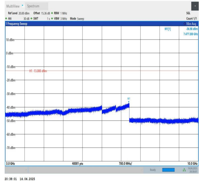
Band26(824-849)-3MHz-QPSK-27025-1RB#14-3000~10000-PASS
