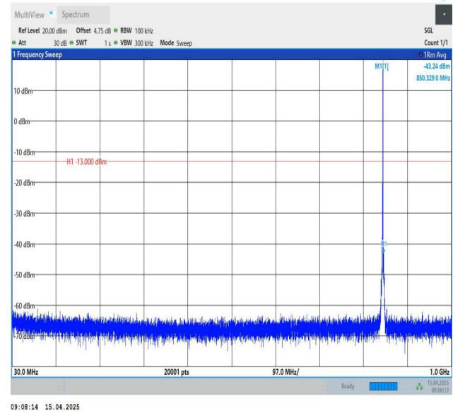
Band26(824-849)-1.4MHz-QPSK-27033-1RB#5-30~1000-PASS
