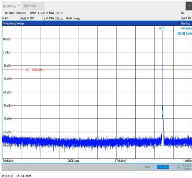
Band26(824-849)-1.4MHz-QPSK-27033-1RB#0-30~1000-PASS
