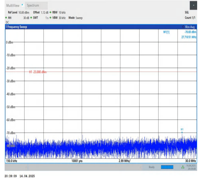
Band26(824-849)-5MHz-QPSK-26915-1RB#0-0.15~30-PASS
