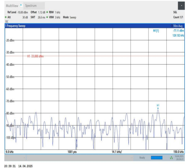
Band26(824-849)-5MHz-QPSK-26915-1RB#24-0.009~0.15-PASS
