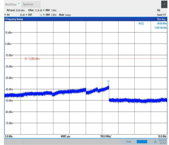
Band26(824-849)-3MHz-QPSK-26915-1RB#14-3000~10000-PASS
