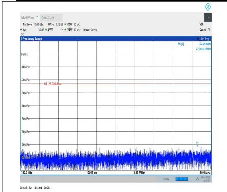
Band26(824-849)-3MHz-QPSK-26805-1RB#14-0.15~30-PASS
