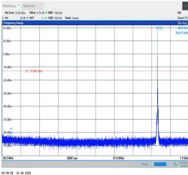
Band26(824-849)-3MHz-QPSK-26915-1RB#0-30~1000-PASS
