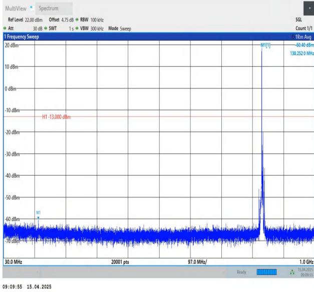
Band26(824-849)-5MHz-QPSK-26915-1RB#0-30~1000-PASS
