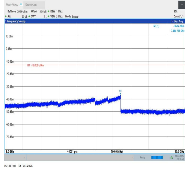
Band26(824-849)-5MHz-QPSK-26815-1RB#24-3000~10000-PASS
