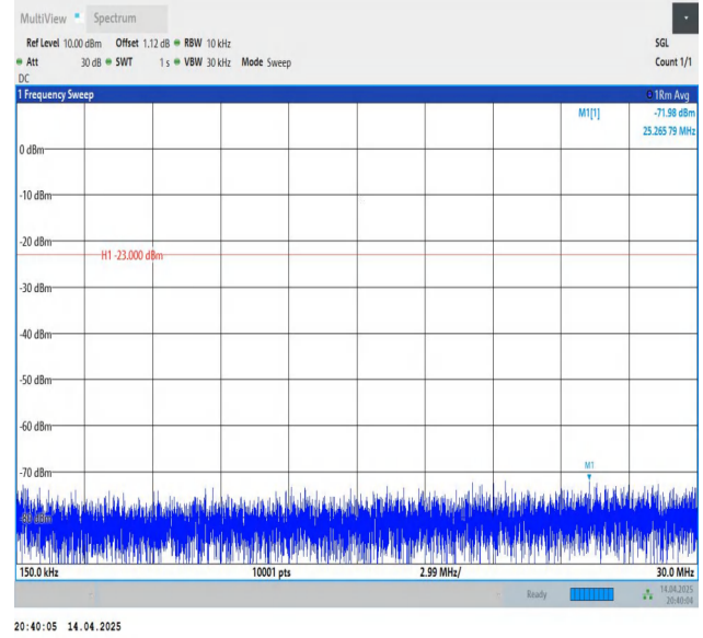
Band26(824-849)-5MHz-QPSK-27015-1RB#0-0.15~30-PASS
