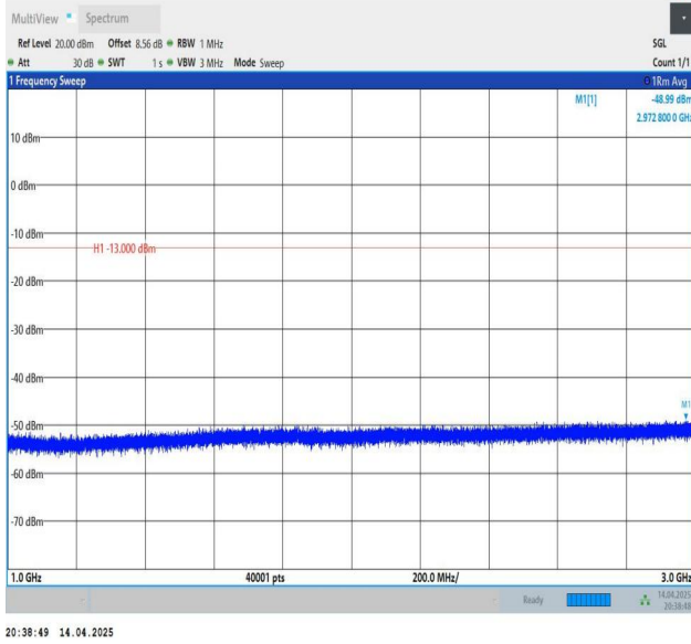
Band26(824-849)-5MHz-QPSK-26815-1RB#24-1000~3000-PASS
