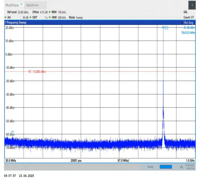
Band26(824-849)-1.4MHz-QPSK-26915-1RB#5-30~1000-PASS
