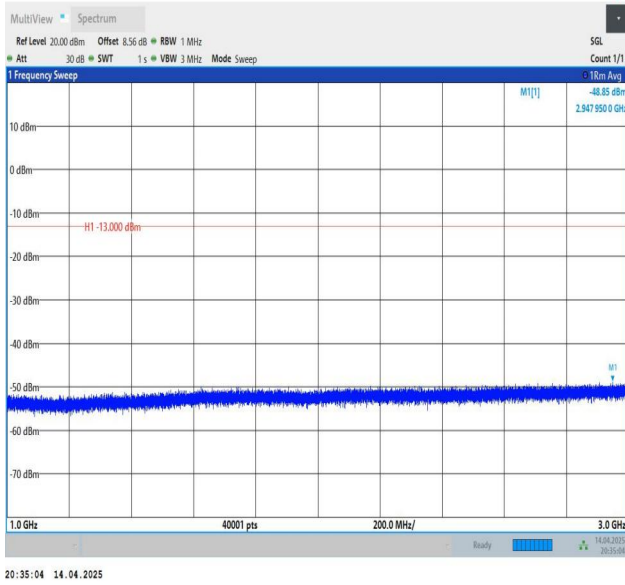
Band26(824-849)-1.4MHz-QPSK-27033-1RB#5-1000~3000-PASS
