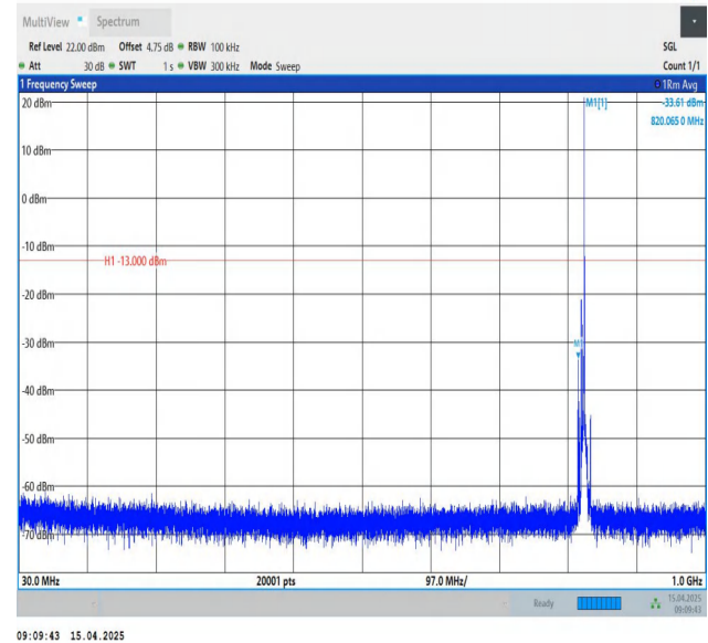
Band26(824-849)-5MHz-QPSK-26815-1RB#24-30~1000-PASS
