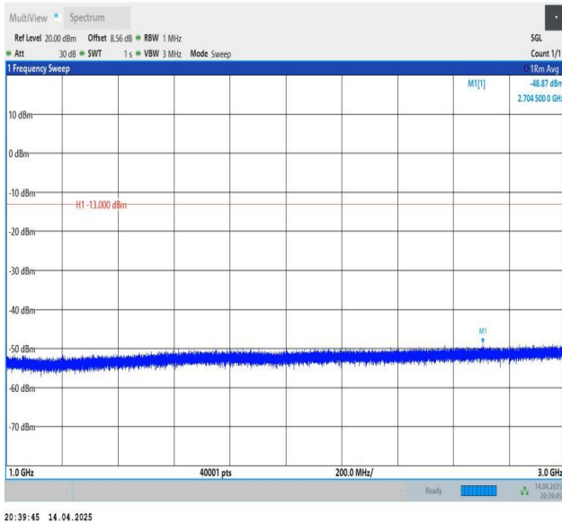
Band26(824-849)-5MHz-QPSK-26915-1RB#24-1000~3000-PASS
