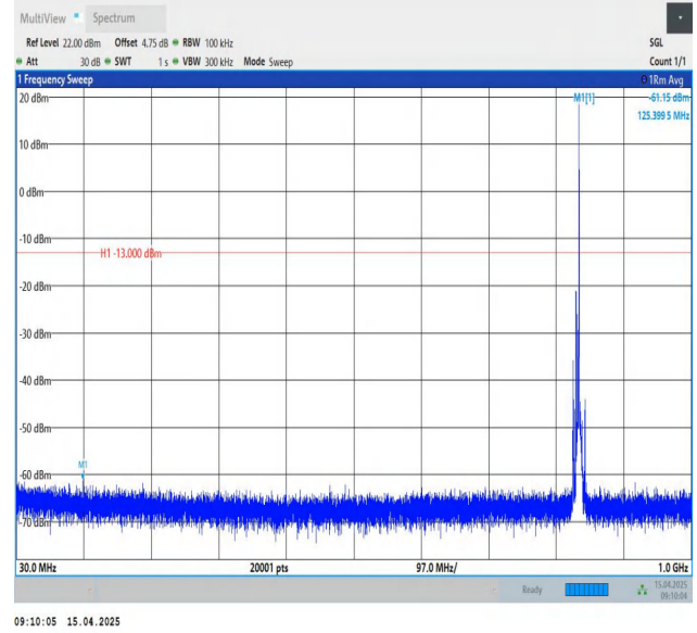
Band26(824-849)-5MHz-QPSK-26915-1RB#24-30~1000-PASS
