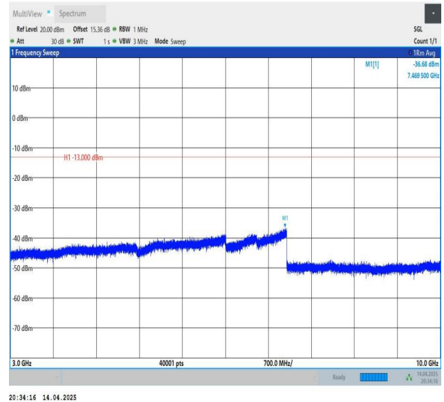
Band26(824-849)-1.4MHz-QPSK-26915-1RB#5-3000~10000-PAS
