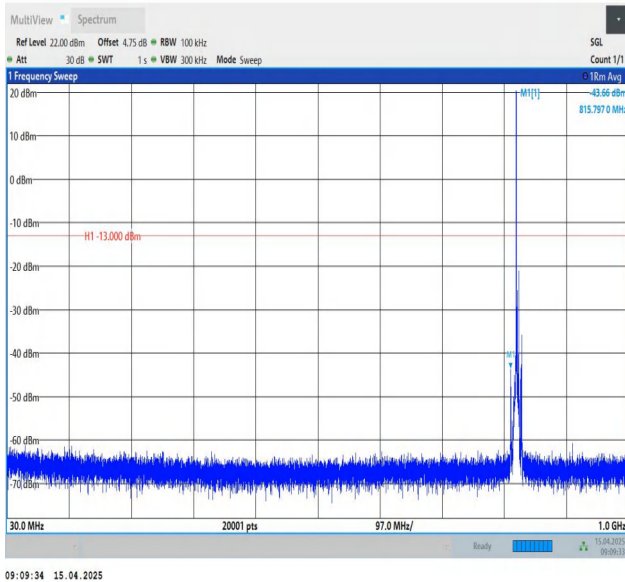
Band26(824-849)-5MHz-QPSK-26815-1RB#0-30~1000-PASS
