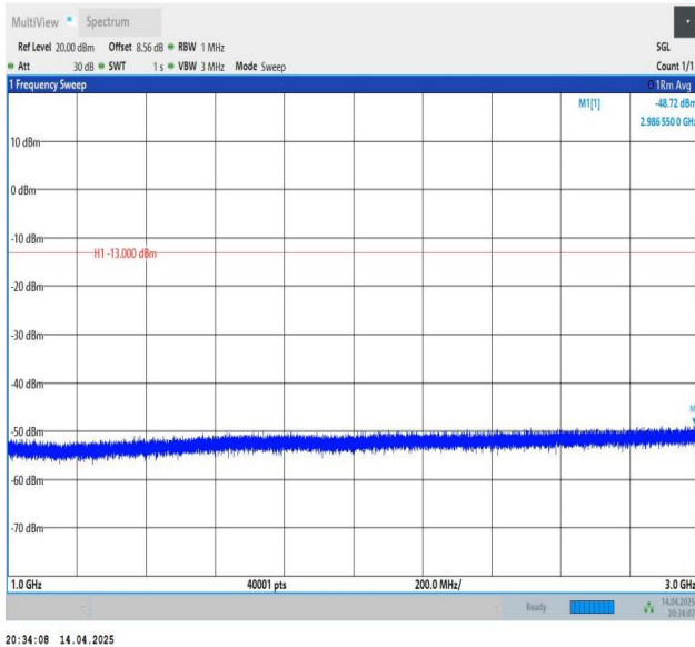
Band26(824-849)-1.4MHz-QPSK-26915-1RB#5-1000~3000-PASS
