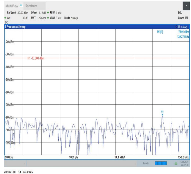
Band26(824-849)-3MHz-QPSK-27025-1RB#14-0.009~0.15-PASS
