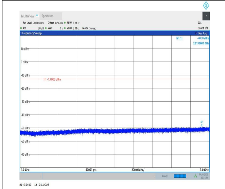
Band26(824-849)-3MHz-QPSK-26805-1RB#14-1000~3000-PASS
