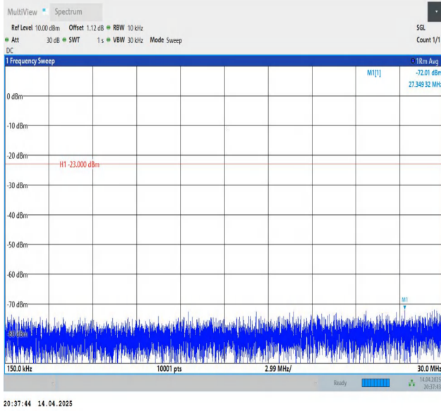
Band26(824-849)-3MHz-QPSK-27025-1RB#14-0.15~30-PASS
