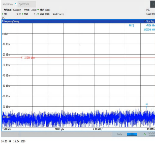
Band26(824-849)-1.4MHz-QPSK-26915-1RB#5-0.15~30-PASS
