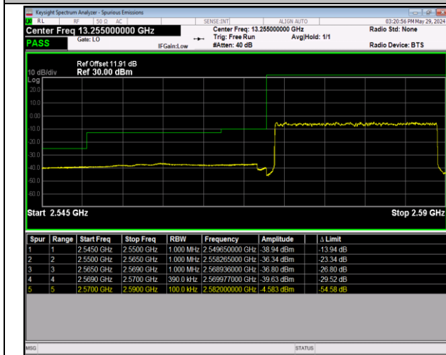
Band38_20MHz_64QAM_37850_100RB#0
