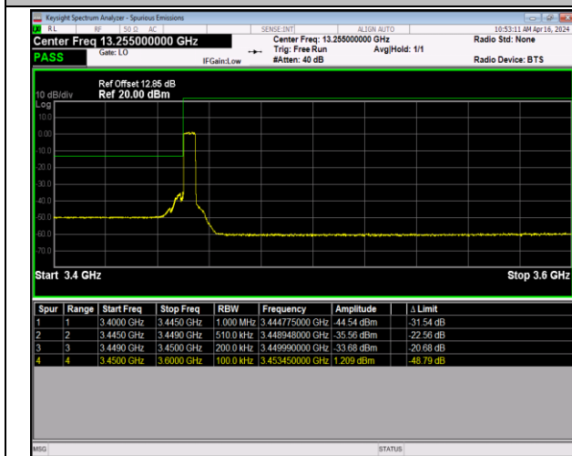
Band42_5MHz_16QAM_42115_25RB#0
