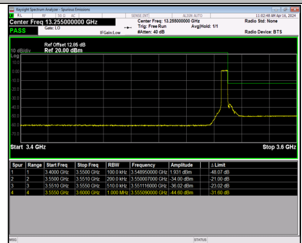
Band42_5MHz_QPSK_43065_25RB#0
