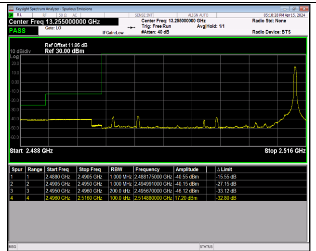
Band41_20MHz_64QAM_39750_1RB#99
