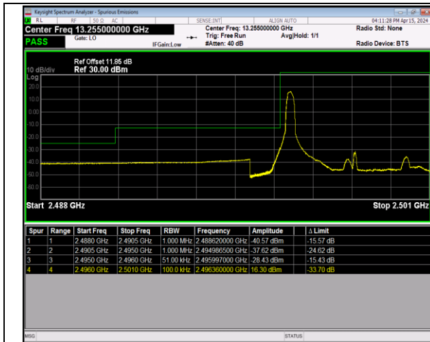
Band41_5MHz_64QAM_39675_1RB#0
