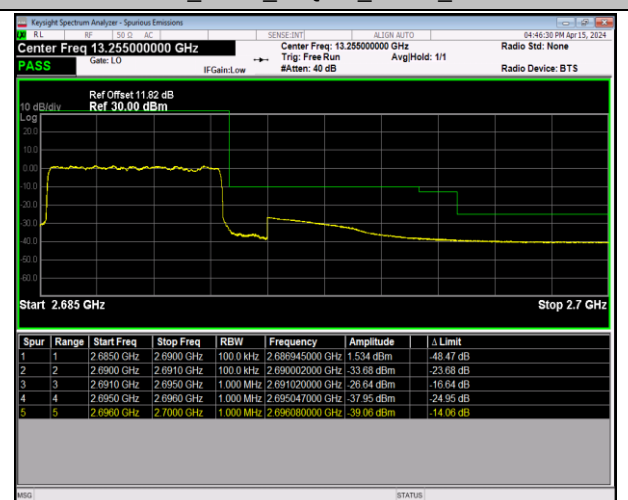
Band41_5MHz_16QAM_41565_25RB#0
