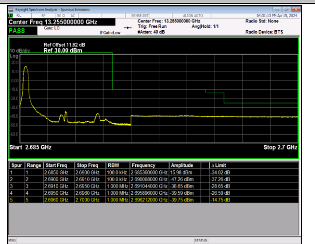
Band41_5MHz_64QAM_41565_1RB#0
