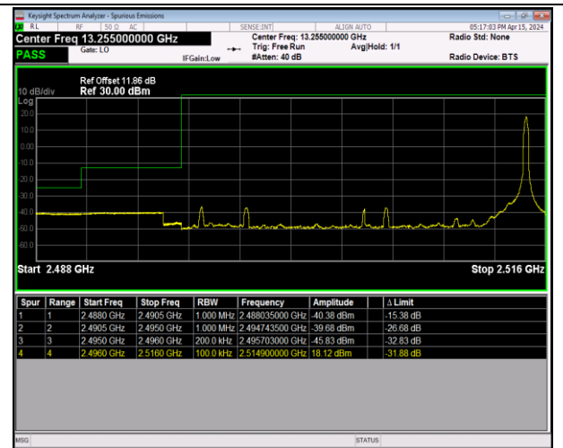
Band41_20MHz_16QAM_39750_1RB#99
