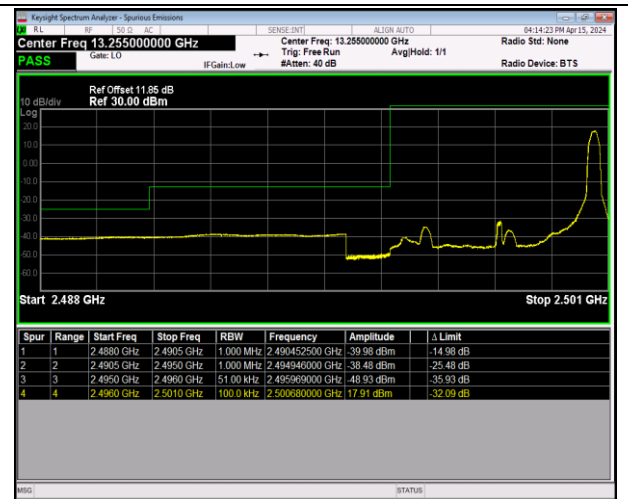
Band41_5MHz_16QAM_39675_1RB#24
