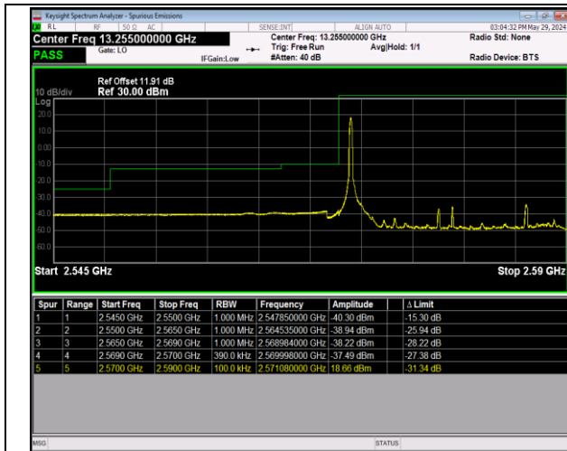
Band38_20MHz_16QAM_37850_1RB#0
