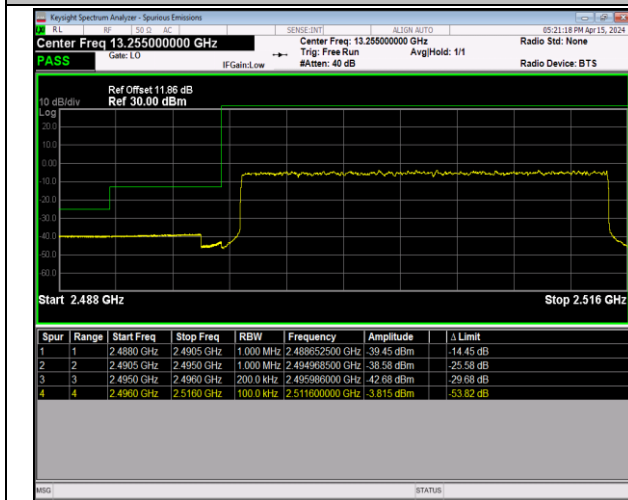
Band41_20MHz_16QAM_39750_100RB#0
