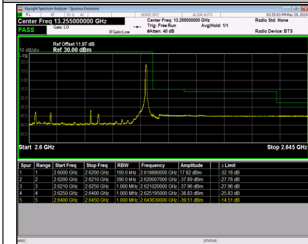
Band38_20MHz_64QAM_38150_1RB#99
