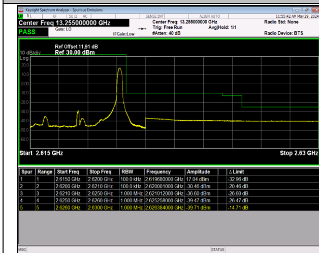
Band38_5MHz_64QAM_38225_1RB#0
