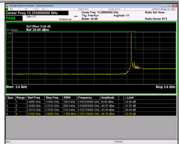
Band42_5MHz_QPSK_43065_1RB#0
