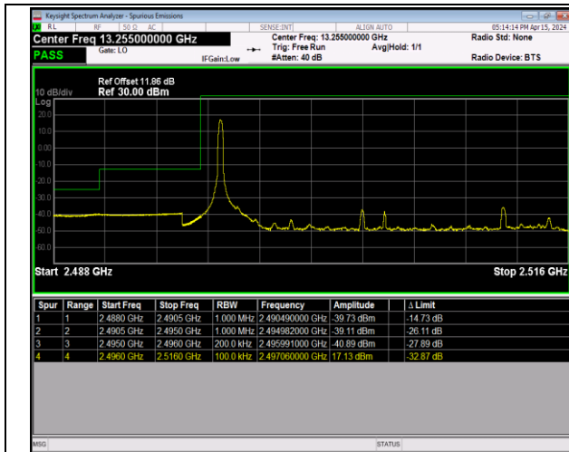
Band41_20MHz_64QAM_39750_1RB#0
