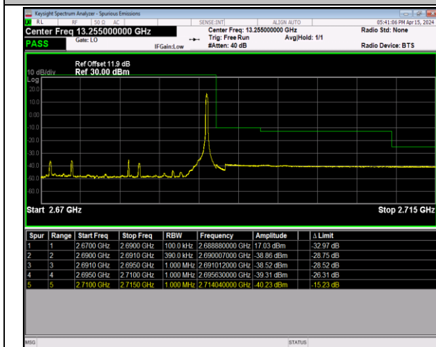
Band41_20MHz_64QAM_41490_1RB#99
