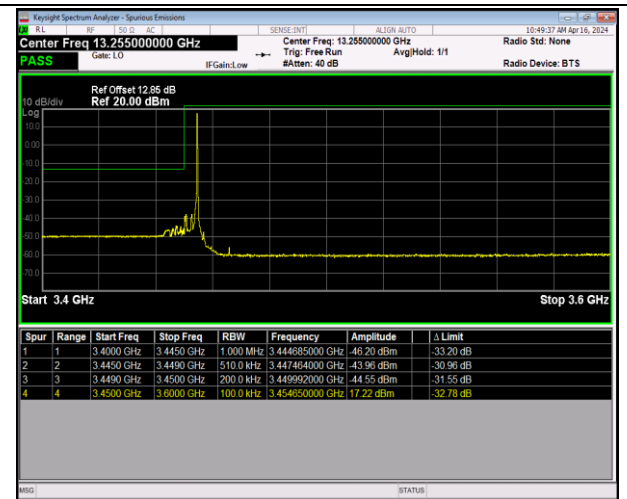
Band42_5MHz_16QAM_42115_1RB#24
