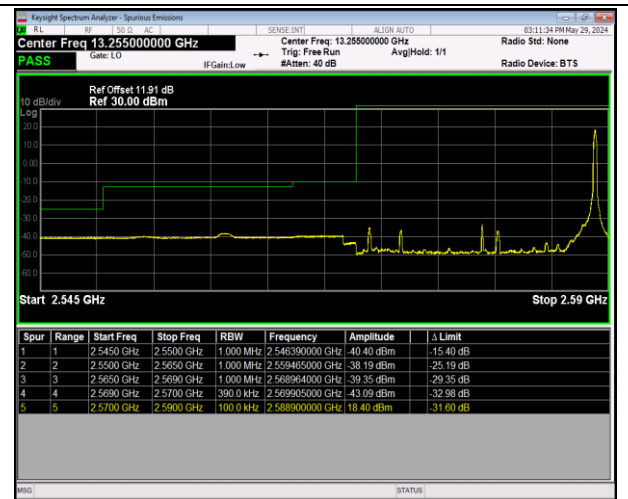
Band38_20MHz_16QAM_37850_1RB#99
