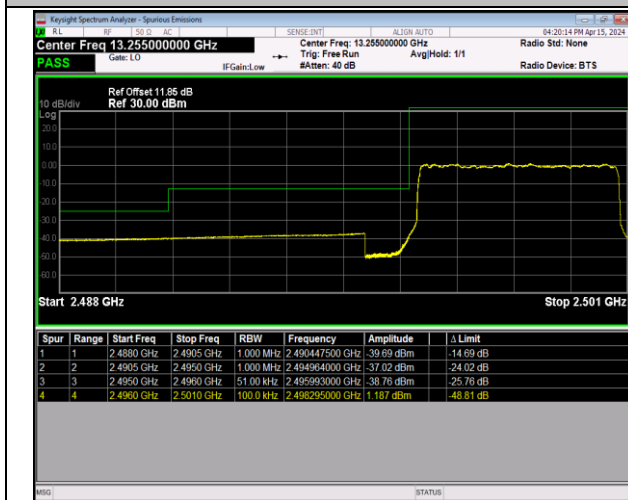
Band41_5MHz_64QAM_39675_25RB#0
