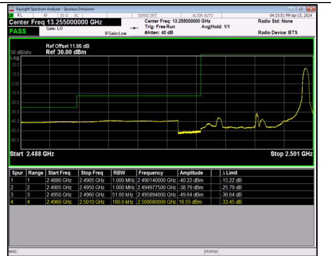
Band41_5MHz_64QAM_39675_1RB#24
