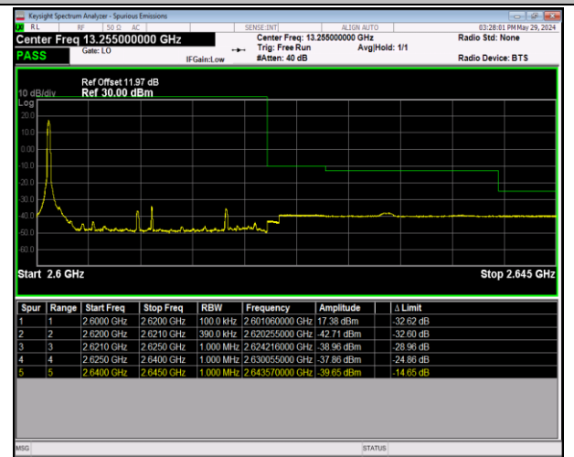
Band38_20MHz_64QAM_38150_1RB#0
