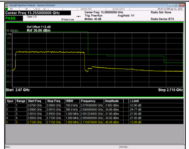
Band41_20MHz_16QAM_41490_100RB#0
