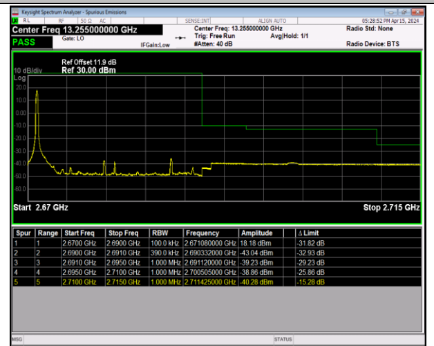
Band41_20MHz_16QAM_41490_1RB#0
