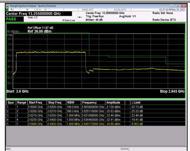
Band38_20MHz_QPSK_38150_100RB#0
