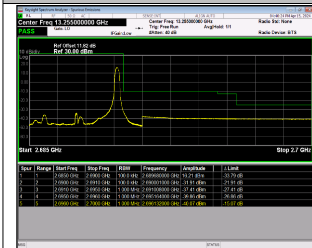
Band41_5MHz_64QAM_41565_1RB#24
