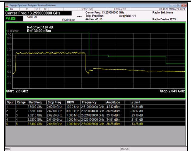
Band38_20MHz_64QAM_38150_100RB#0
