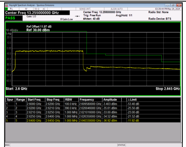
Band38_20MHz_16QAM_38150_100RB#0
