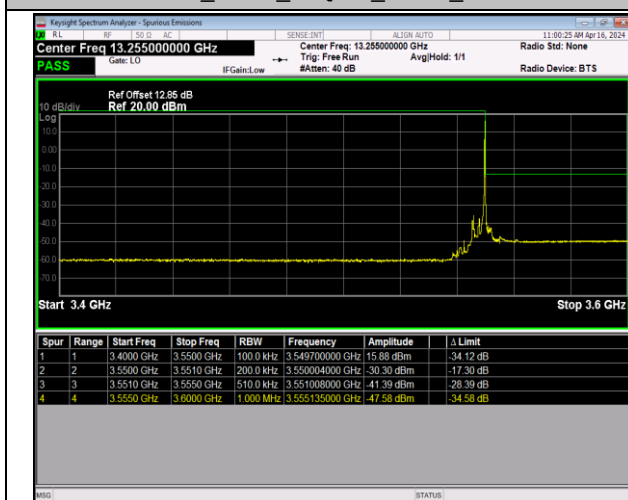
Band42_5MHz_16QAM_43065_1RB#24
