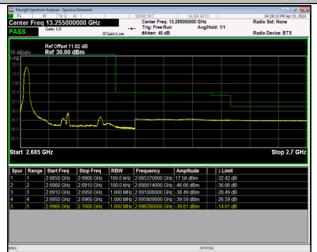
Band41_5MHz_16QAM_41565_1RB#0
