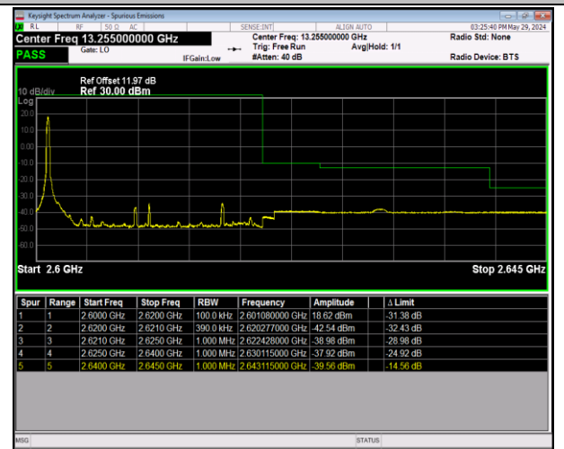
Band38_20MHz_16QAM_38150_1RB#0
