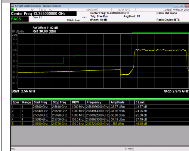
Band38_5MHz_64QAM_37775_25RB#0
