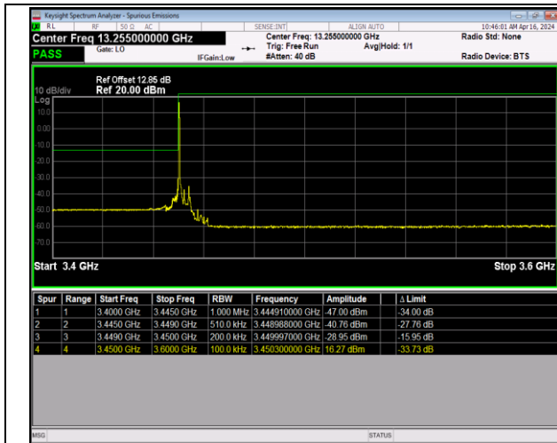
Band42_5MHz_16QAM_42115_1RB#0
