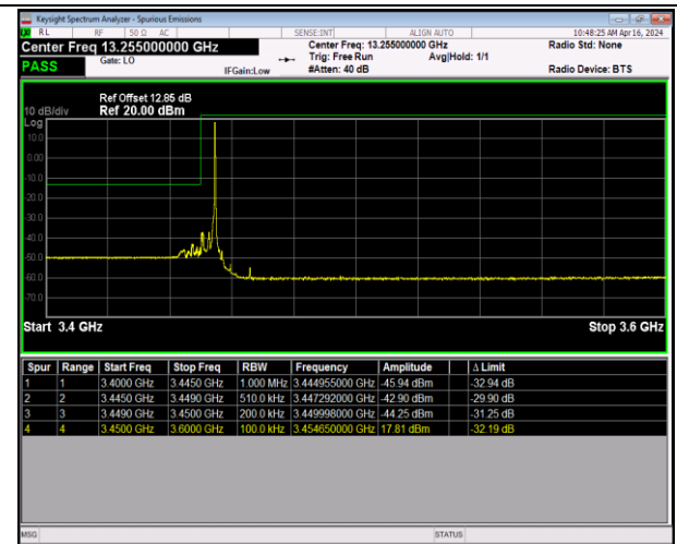
Band42_5MHz_QPSK_42115_1RB#24
