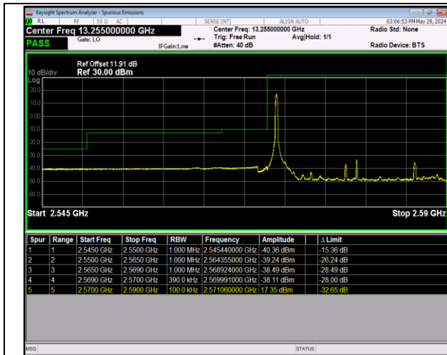
Band38_20MHz_64QAM_37850_1RB#0
