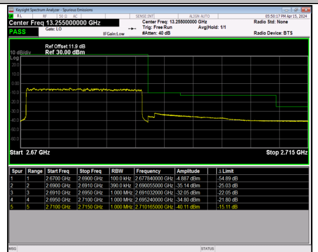
Band41_20MHz_64QAM_41490_100RB#0
