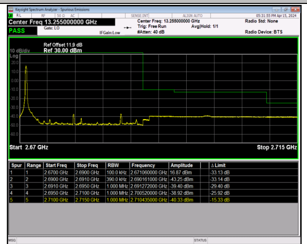
Band41_20MHz_64QAM_41490_1RB#0
