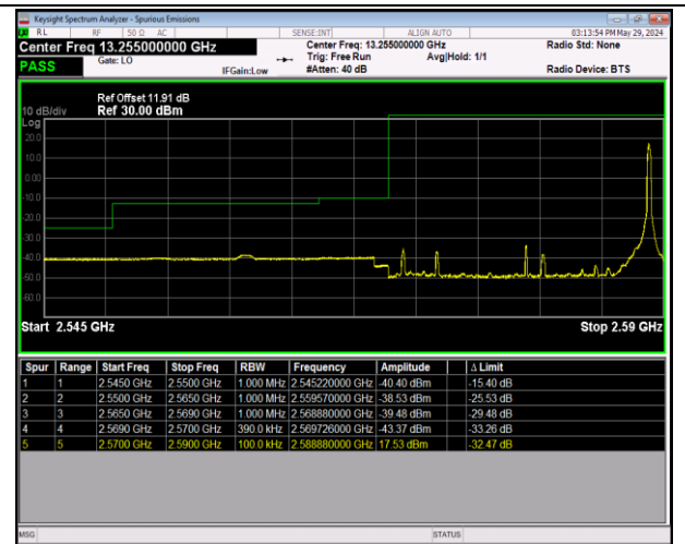
Band38_20MHz_64QAM_37850_1RB#99
