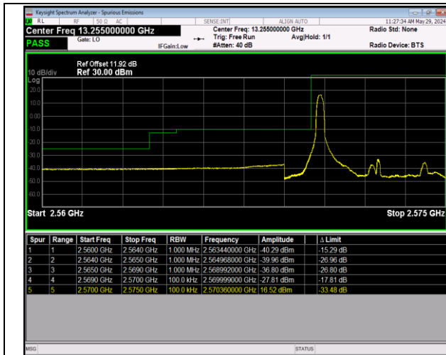
Band38_5MHz_64QAM_37775_1RB#0
