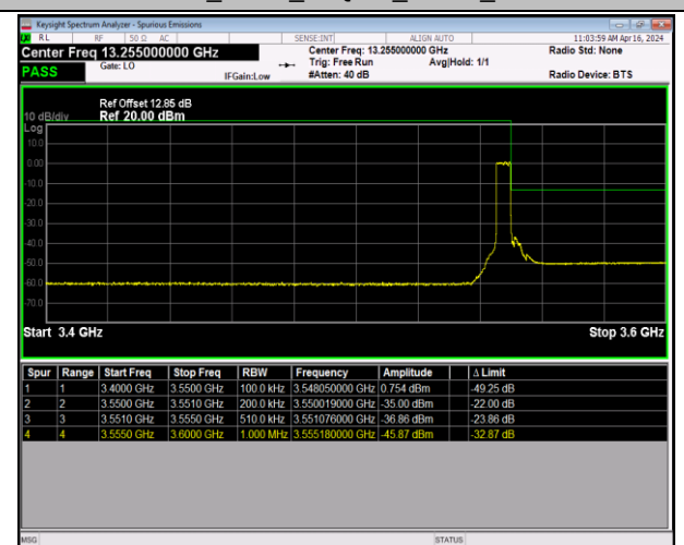
Band42_5MHz_16QAM_43065_25RB#0
