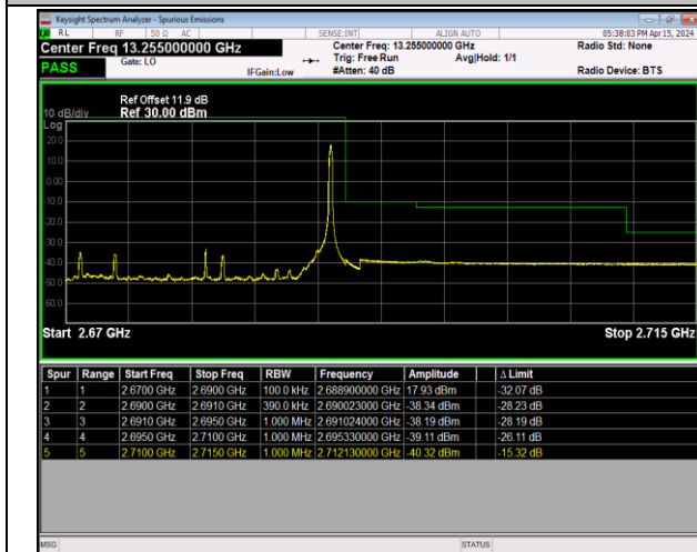
Band41_20MHz_16QAM_41490_1RB#99
