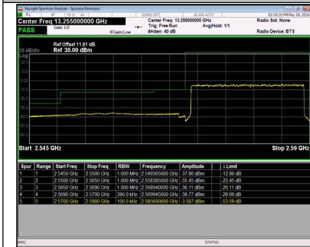
Band38_20MHz_16QAM_37850_100RB#0
