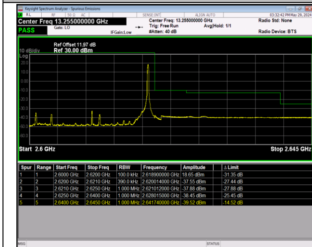
Band38_20MHz_16QAM_38150_1RB#99
