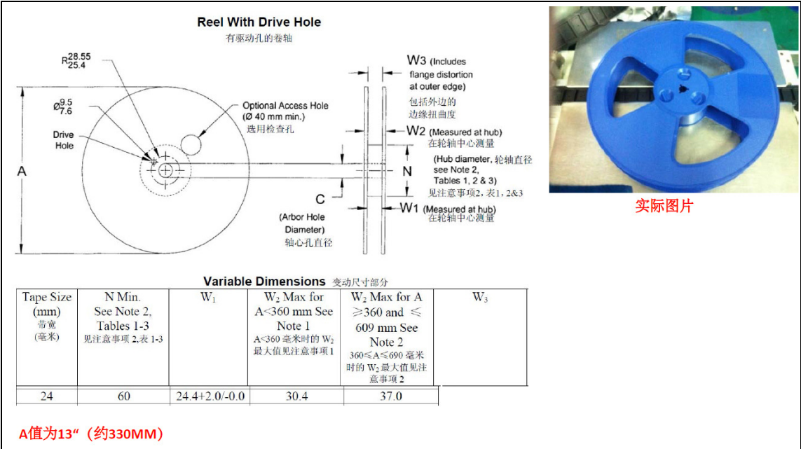
Figure 18: Reel specifications
