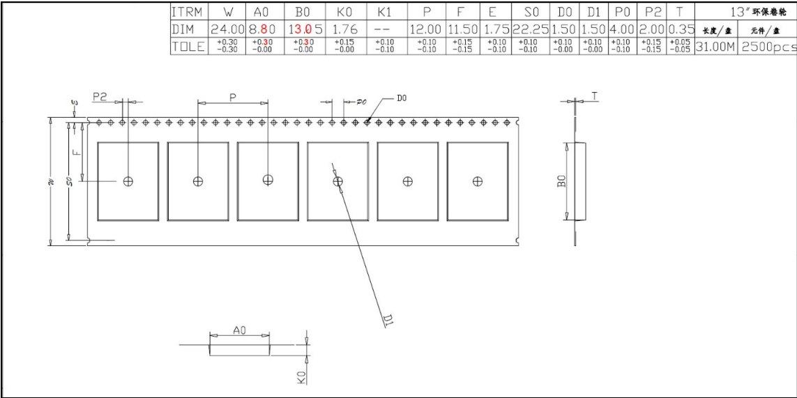
Figure 19: Tape specifications
