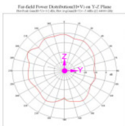
Figure 13: Antenna patterns
