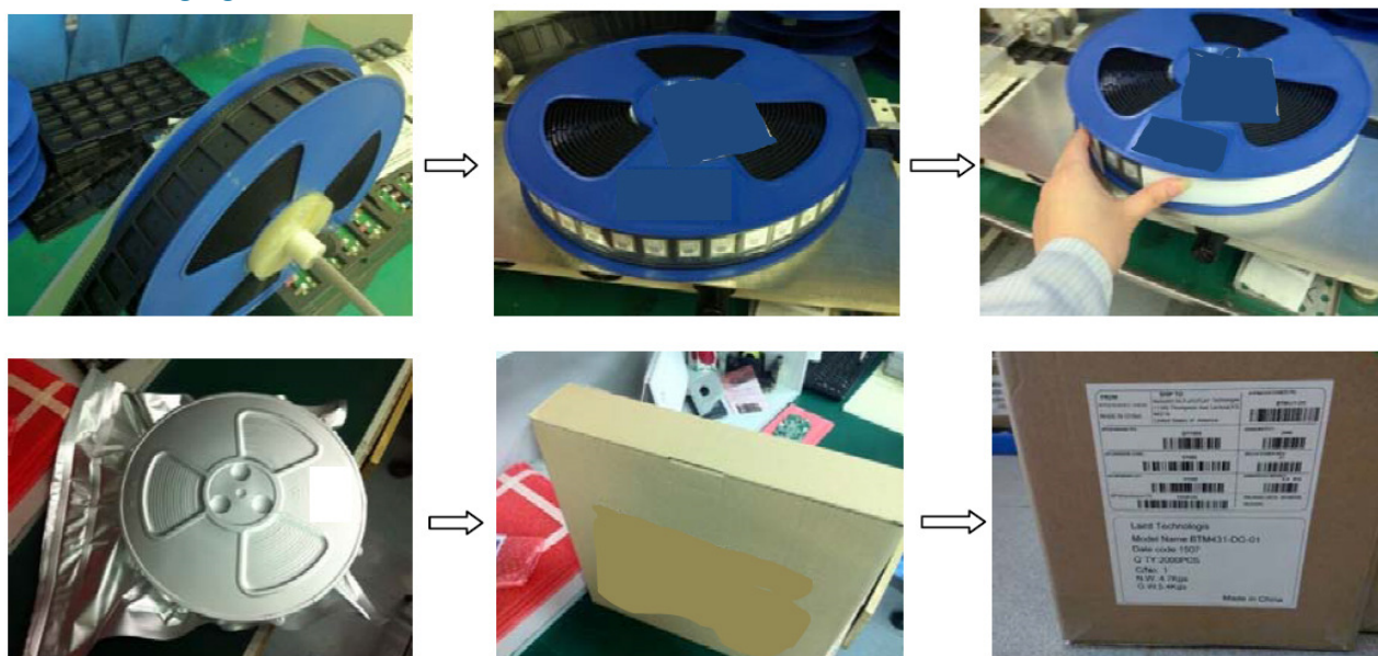
Figure 20: Packaging process
