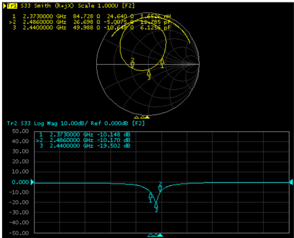
Figure 12: Antenna return loss
