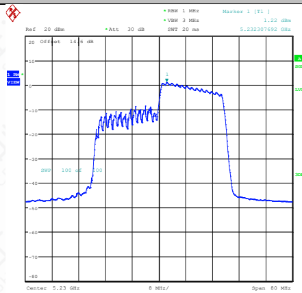
11AX40MIMO-Ant1-5230-242Tone-RU62-PASS
