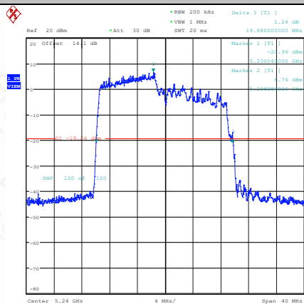
11AX20SISO-Ant1-5240-106Tone-RU53
