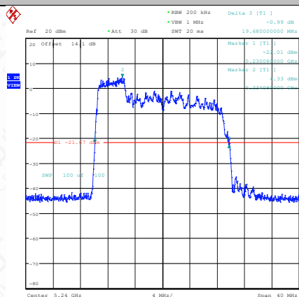
11AX20SISO-Ant1-5240-52Tone-RU37
