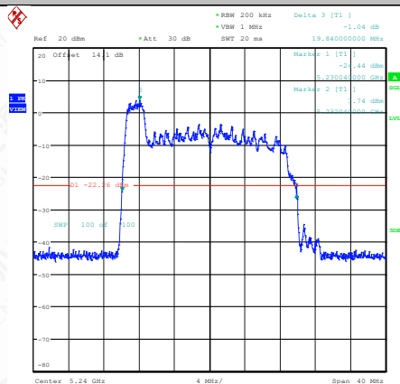
11AX20SISO-Ant1-5240-26Tone-RU0
