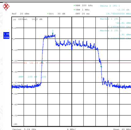
11AX20SISO-Ant2-5240-52Tone-RU37
