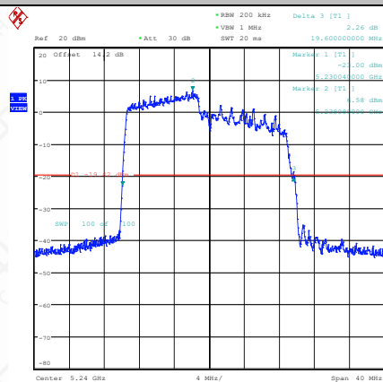
11AX20SISO-Ant2-5240-106Tone-RU53
