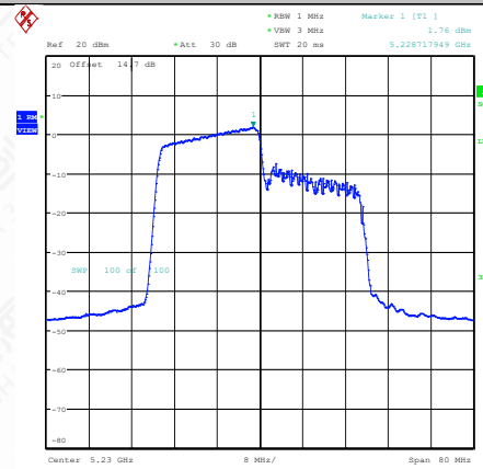
11AX40MIMO-Ant2-5230-242Tone-RU61-PASS
