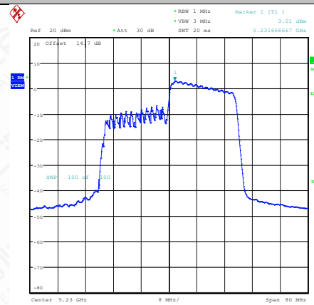
11AX40MIMO-Ant2-5230-242Tone-RU62-PASS
