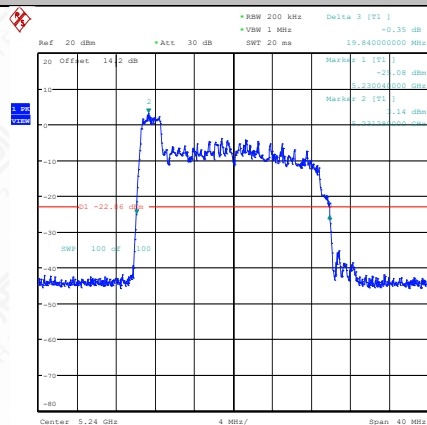
11AX20SISO-Ant2-5240-26Tone-RU0
