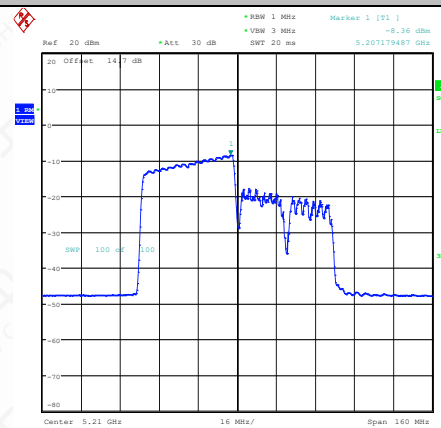
11AX80SISO-Ant2-5210-484Tone-RU65-PASS
