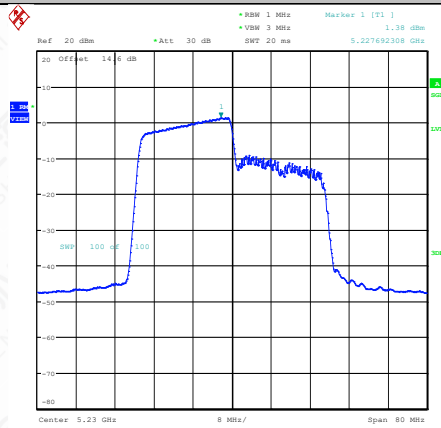
11AX40MIMO-Ant1-5230-242Tone-RU61-PASS
