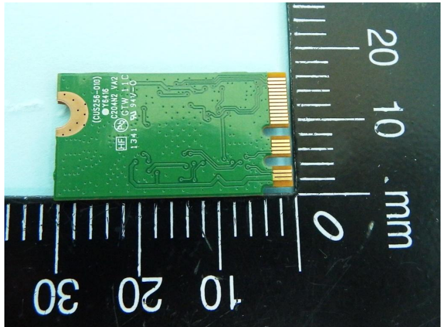
Antenna No.: 3 Brand Name: ACON Antenna Type: PIFA
