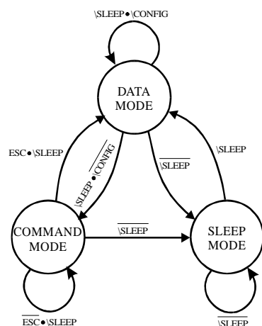
Figure 5a - Menu Interface State Diagram
