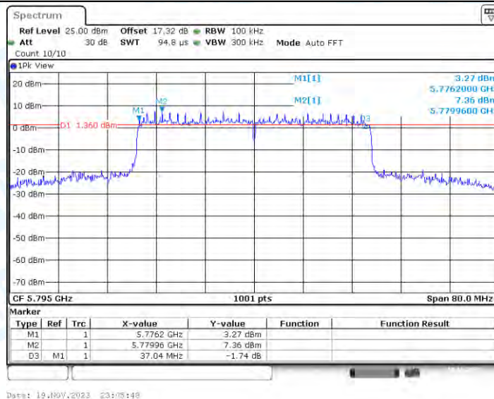
11AX40-CDD_Ant4_5795
