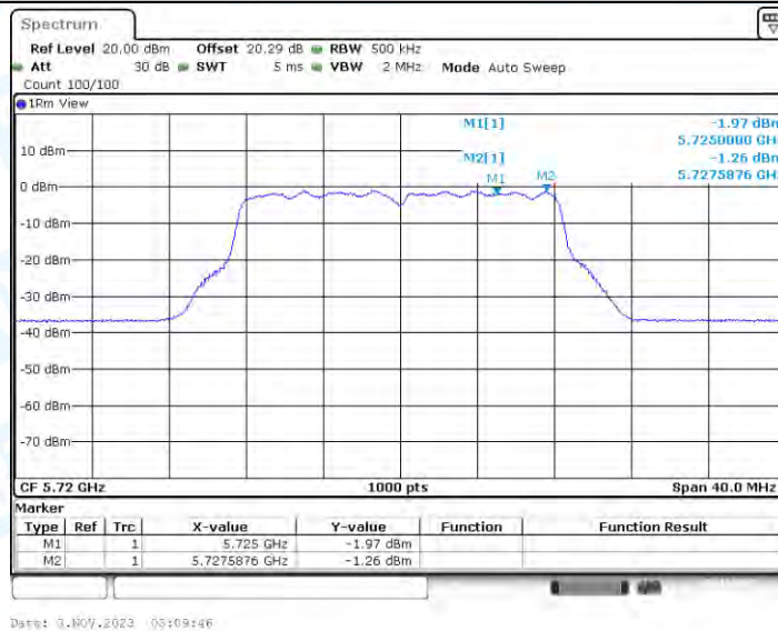
11A-CDD_Ant4_5720_UNII-3
