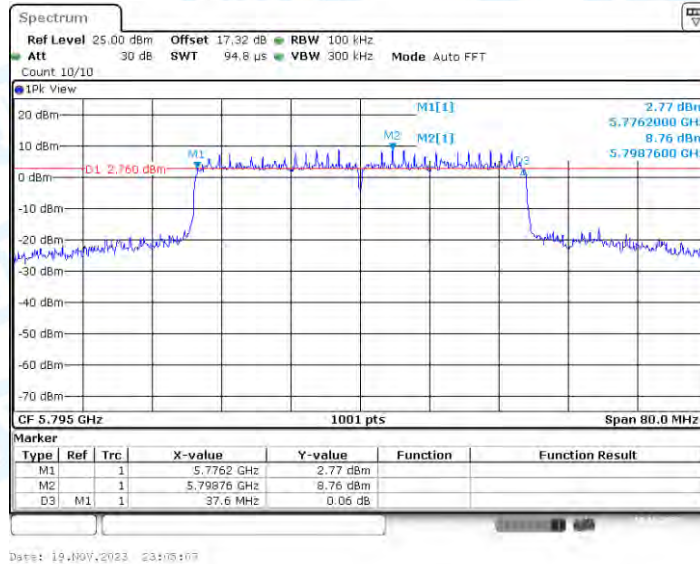
11AX40-CDD_Ant3_5795
