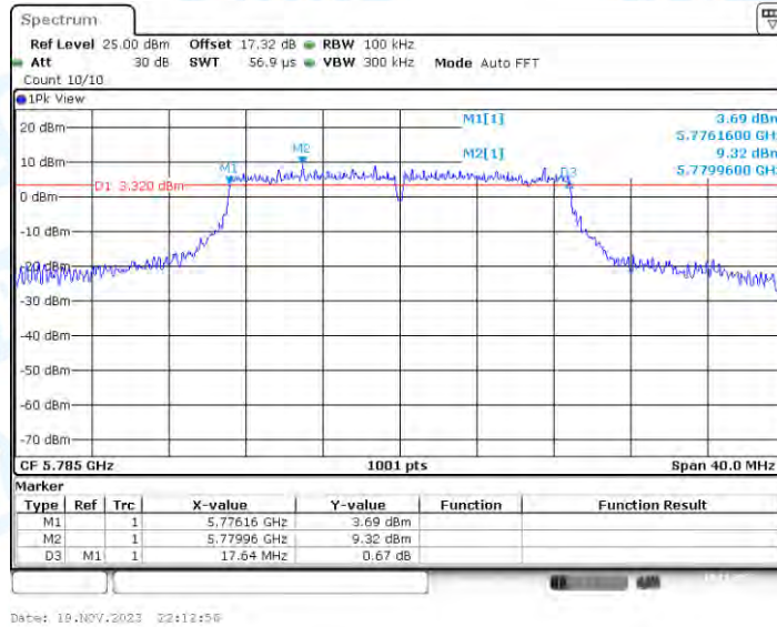
11N20-CDD_Ant4_5785
