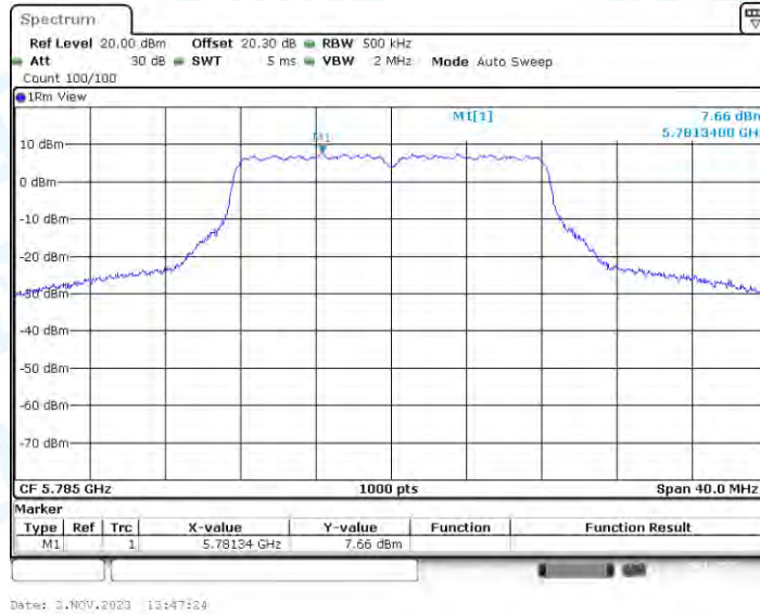
11A-CDD_Ant3_5785
