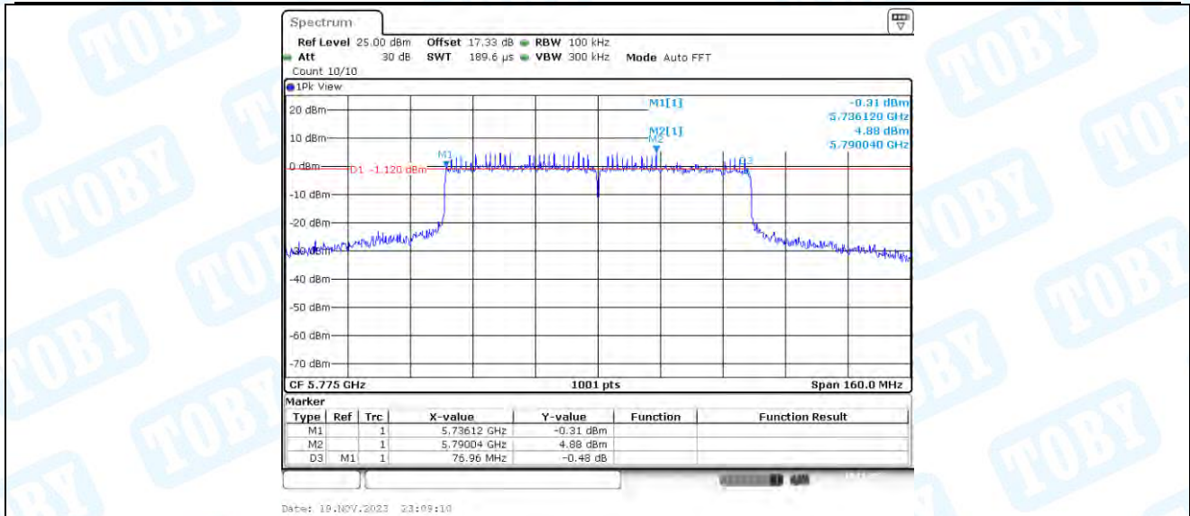
11AX80-CDD_Ant4_5775
