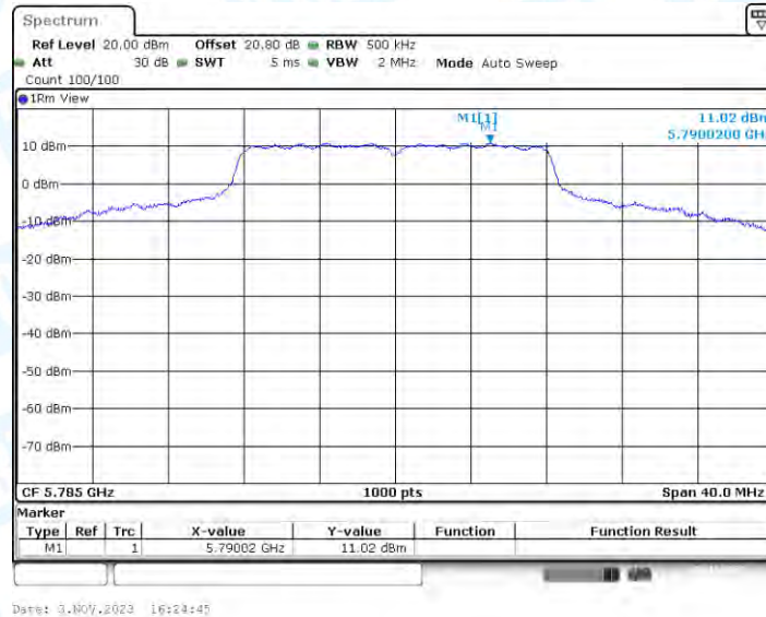
11A_Ant4_5785
