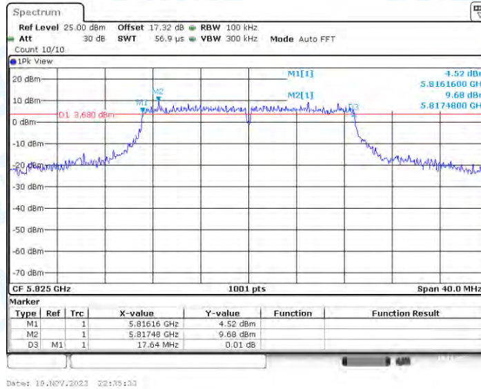
11AC20-CDD_Ant4_5825
