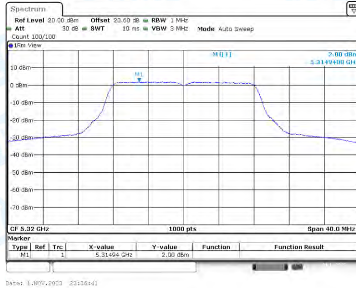
11A-CDD_Ant4_5320
