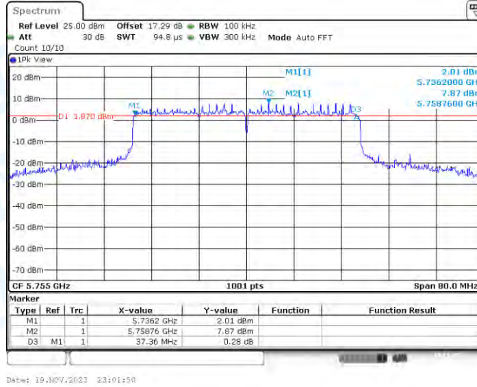
11AX40-CDD_Ant3_5755
