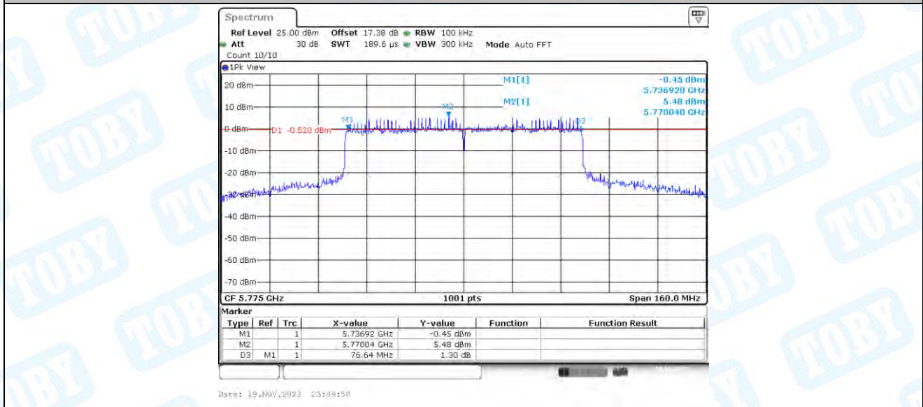
11AX80-CDD_Ant4_5775
