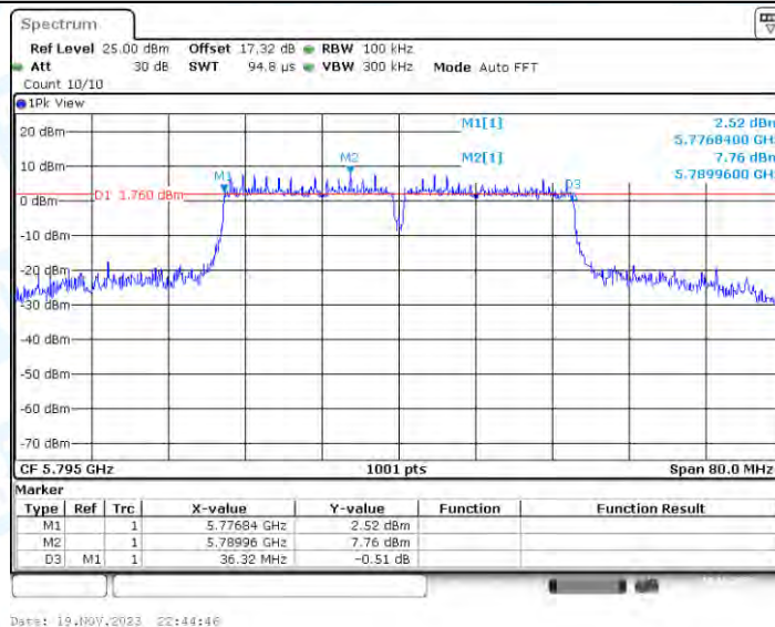
11AC40-CDD_Ant4_5795
