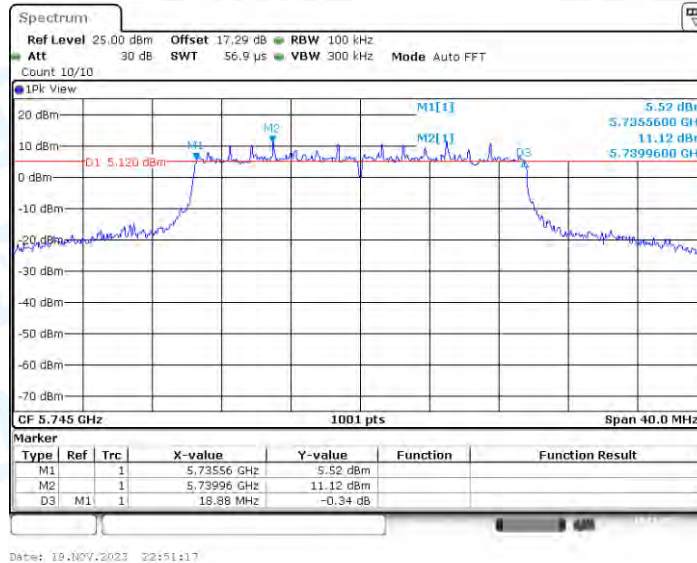
11AX20-CDD_Ant3_5745
