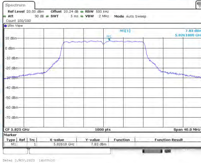
11A-CDD_Ant3_5825
