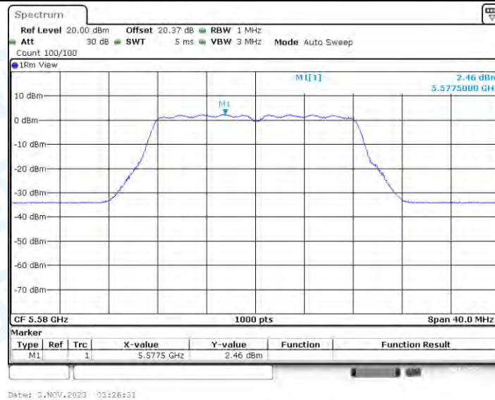
11A-CDD_Ant3_5580
