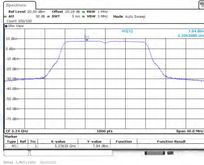
11A-CDD_Ant4_5240
