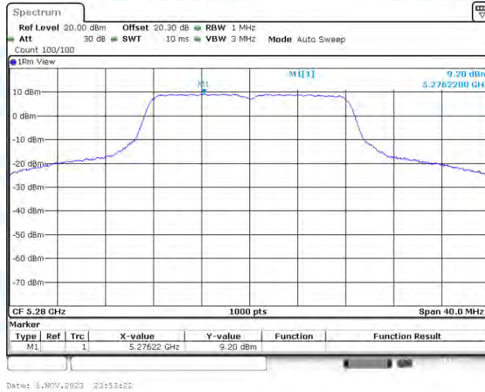
11A_Ant4_5280
