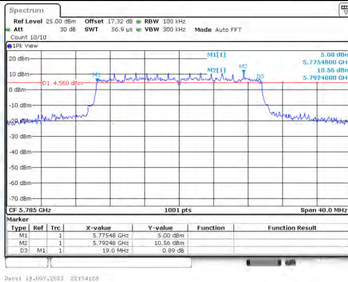
11AX20-CDD_Ant3_5785
