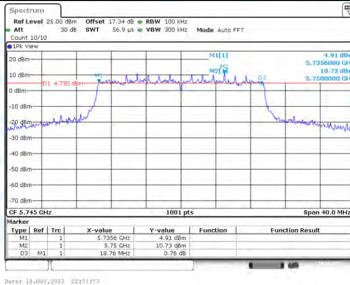
11AX20-CDD_Ant4_5745
