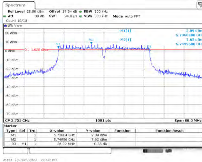
11AC40-CDD_Ant4_5755
