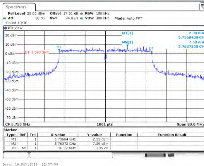
11AC40-CDD_Ant2_5755
