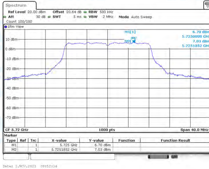
11A_Ant4_5720_UNII-3
