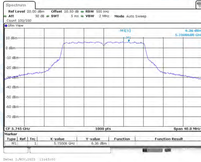
11A-CDD_Ant4_5745
