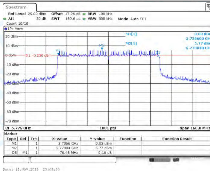
11AX80-CDD_Ant3_5775
