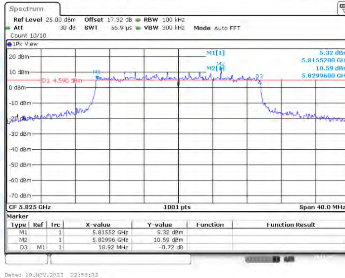
11AX20-CDD_Ant4_5825
