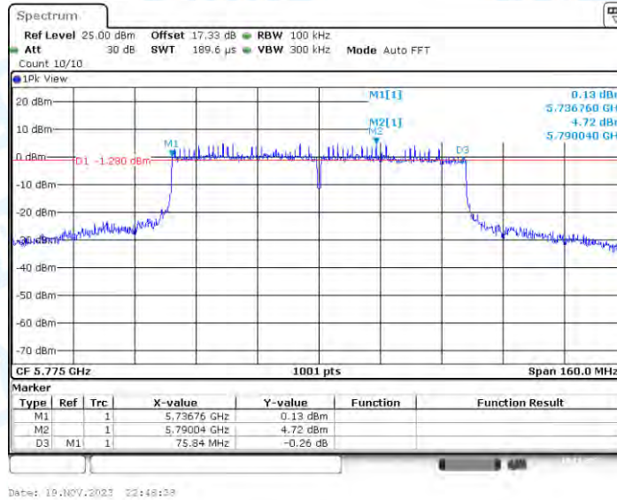
11AC80-CDD_Ant4_5775
