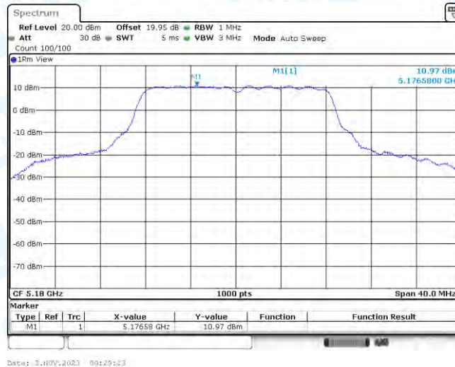
11A_Ant3_5180
