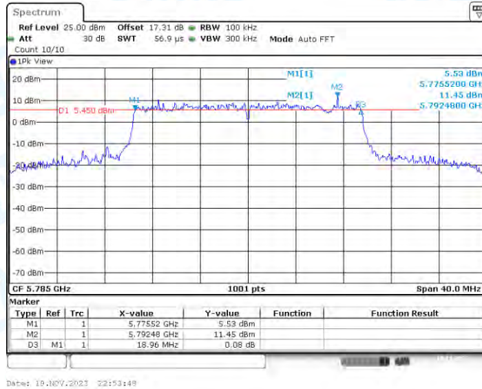
11AX20-CDD_Ant2_5785
