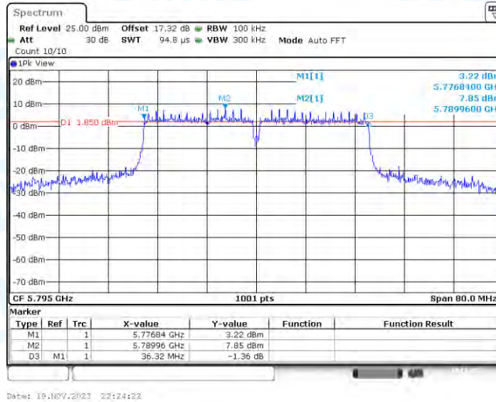
11N40-CDD_Ant4_5795
