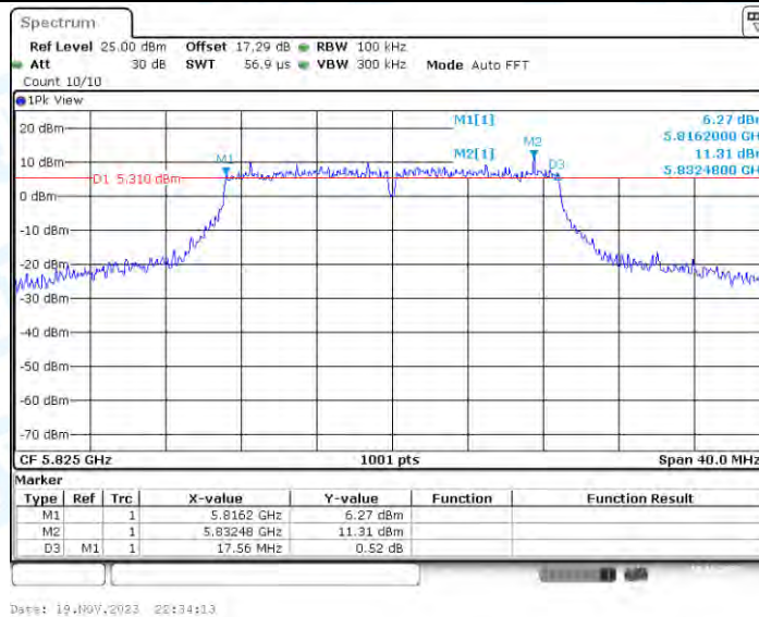
11AC20-CDD_Ant2_5825
