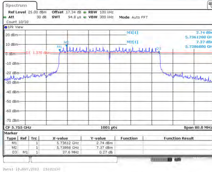
11AX40-CDD_Ant4_5755
