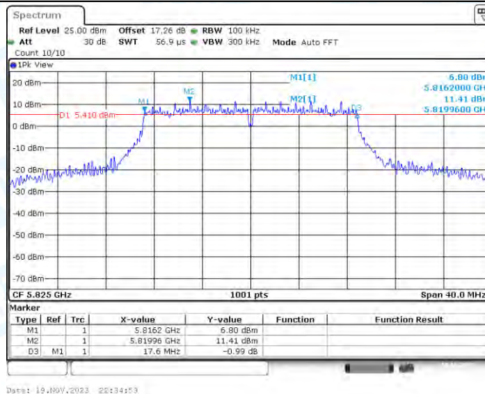
11AC20-CDD_Ant3_5825
