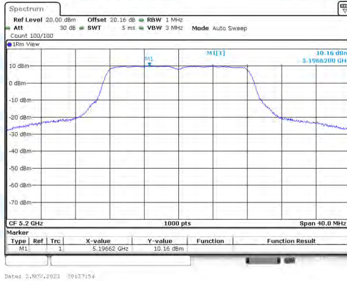
11A_Ant4_5200
