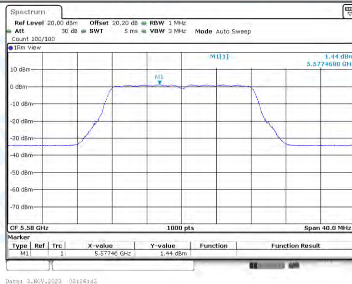
11A-CDD_Ant4_5580
