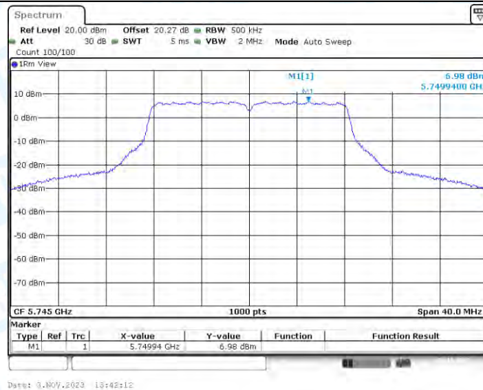
11A-CDD_Ant3_5745
