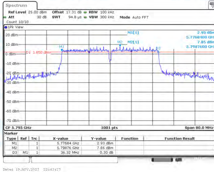
11AC40-CDD_Ant2_5795
