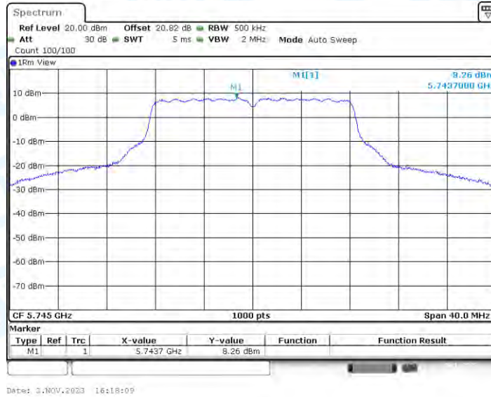
11A_Ant4_5745
