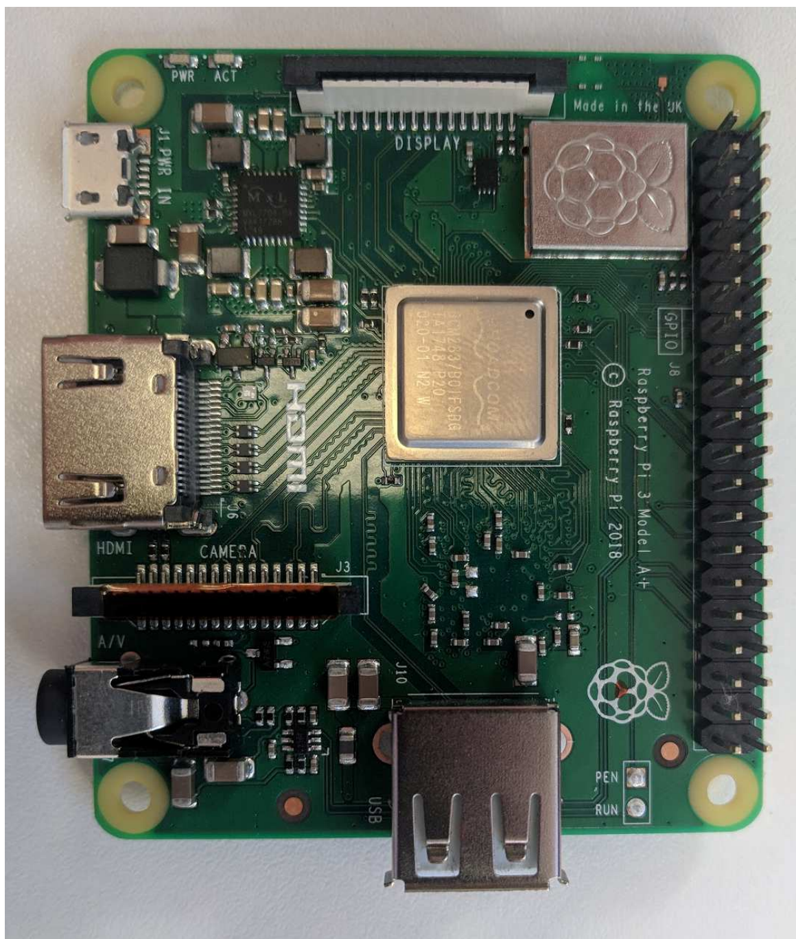
R-Pi 3A+ [Front Photo]
