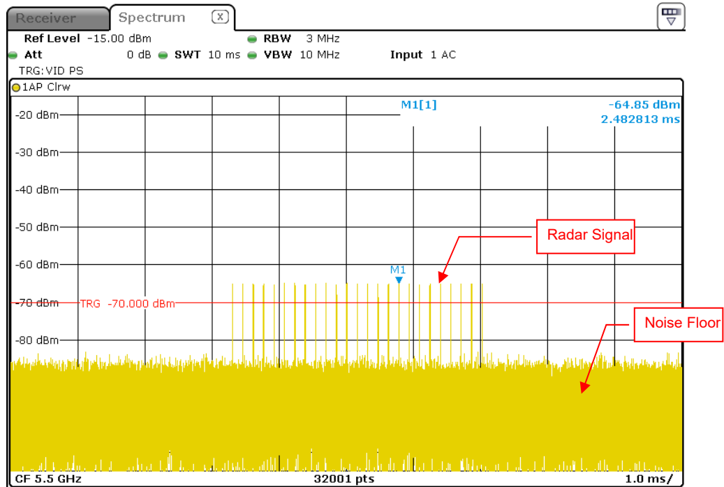
Radar Signal 2
