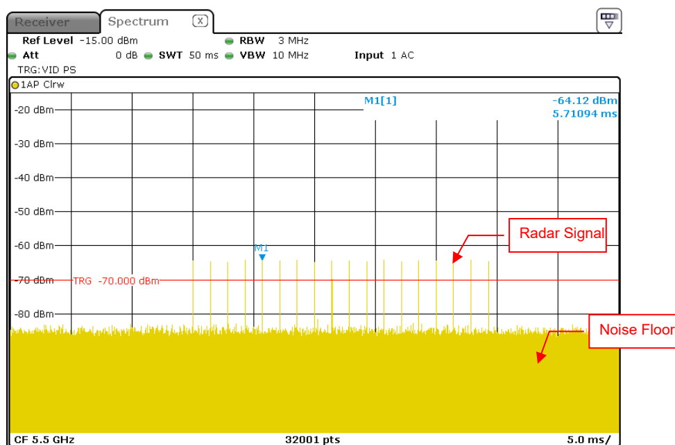
Radar Signal 0
