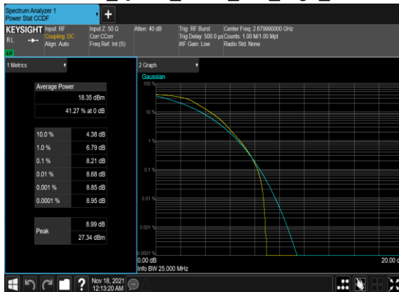
B4_N41(20M)_DFT-s- OFDM_QPSK_Outer_Full_High_CH
