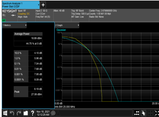
B4_N41(20M)_DFT-s-OFDM_PI_2- BPSK_Outer_Full_High_CH
