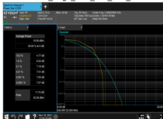
B4_N41(20M)_DFT-s-OFDM_PI_2- BPSK_Edge_1RB_Left_Low_CH
