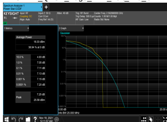
B4_N41(20M)_DFT-s- OFDM_QPSK_Edge_1RB_Left_Mid_CH
