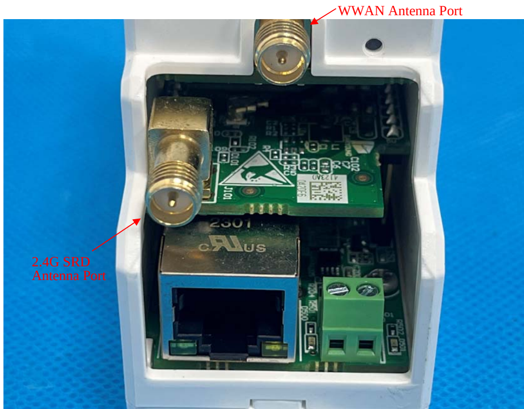
WWAN Antenna(The 2.4G SRD has the same antenna as the WWAN)
