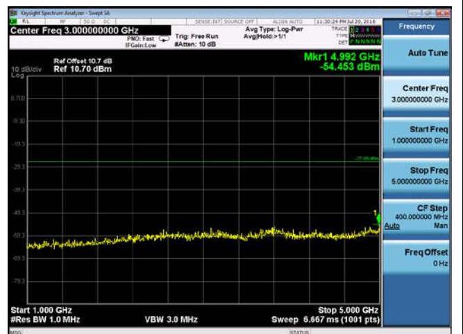
CUE-802.11a-5280M-chain1(1GHz-5GHz)
