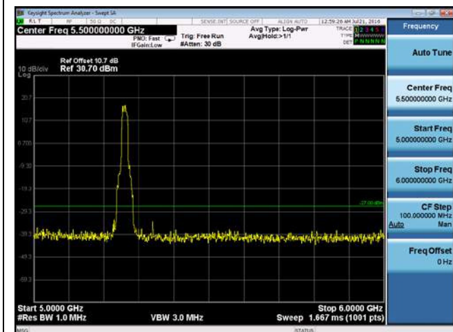
CUE-802.11a-5260M-chain3(5GHz-6GHz)
