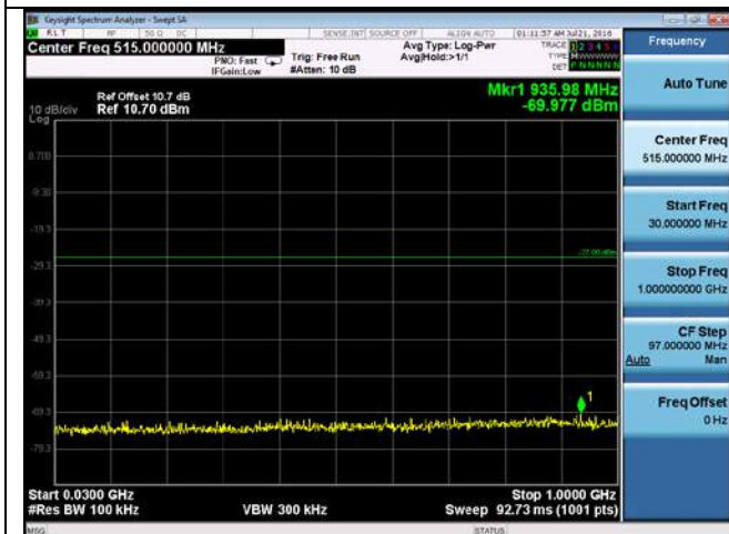
CUE-802.11n-20-5260M -chain3(30MHz-1GHz)
