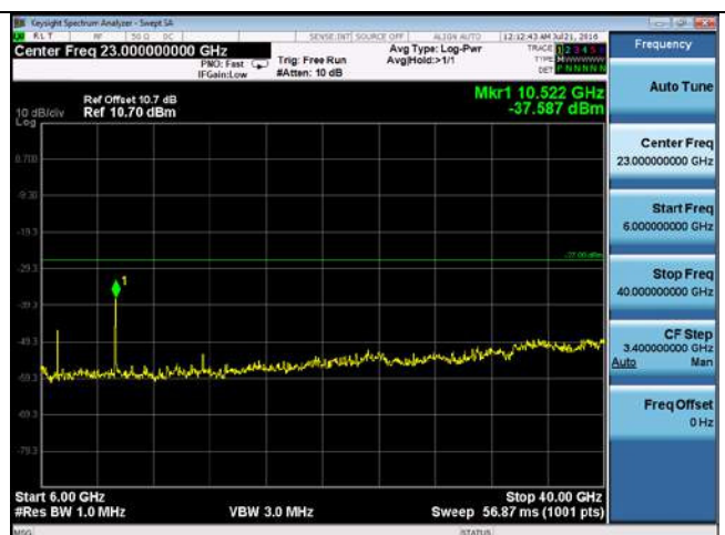
CUE-802.11a-5260M -chain2(6GHz-40GHz)
