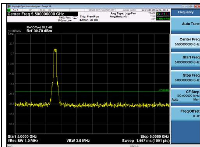
CUE-802.11n-20-5260M chain2(5GHz-6GHz)
