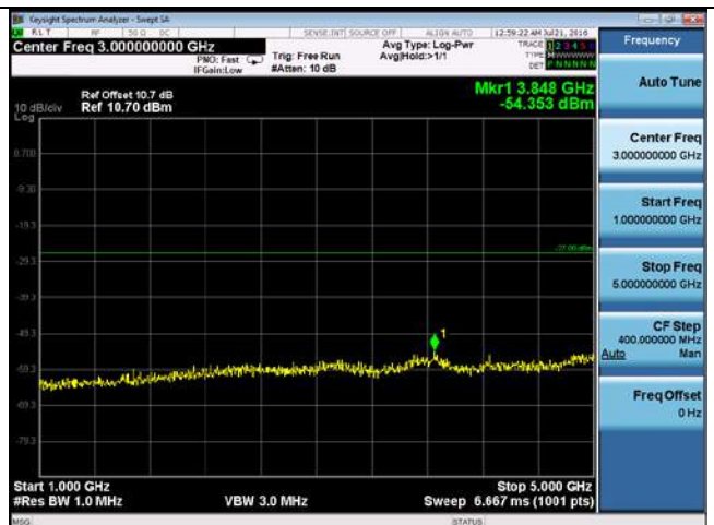
CUE-802.11a-5260M -chain3(1GHz-5GHz)
