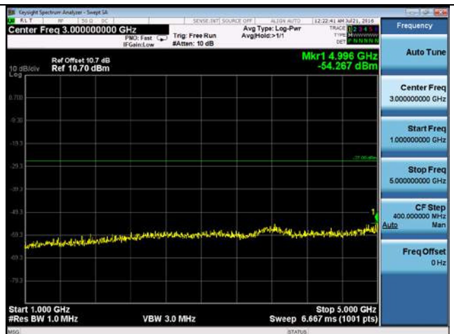
CUE-802.11n-20-5280M -chain2(1GHz-5GHz)
