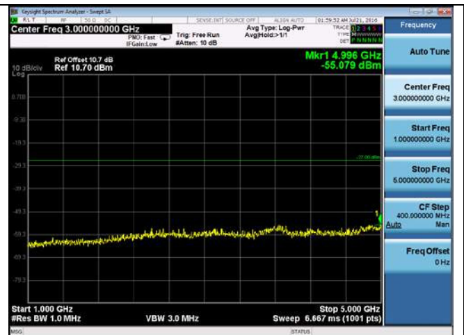
CUE-802.11n-20-5260M-chain4(1GHz-5GHz)
