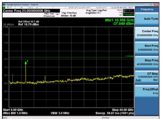
CUE-802.11n-20-5280M -chain2(6GHz-40GHz)
