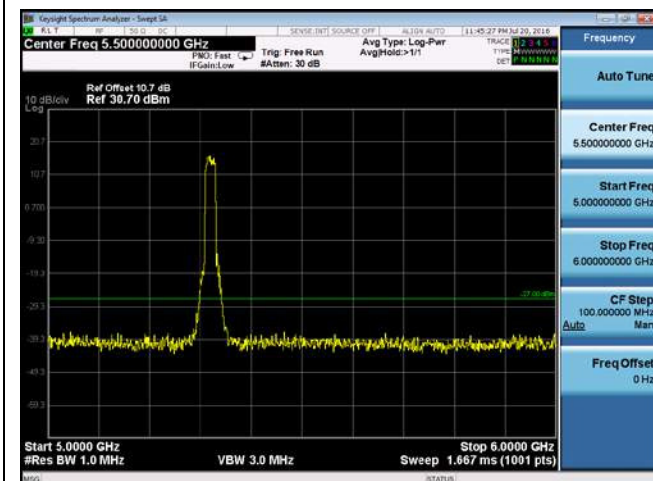
CUE-802.11n-20-5320M-chain 1(5GHz-6GHz)
