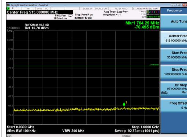
CUE-802.11a-5320M-chain 1(30MHz-1GHz)
