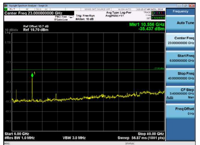
CUE-802.11a-5280M -chain2(6GHz-40GHz)
