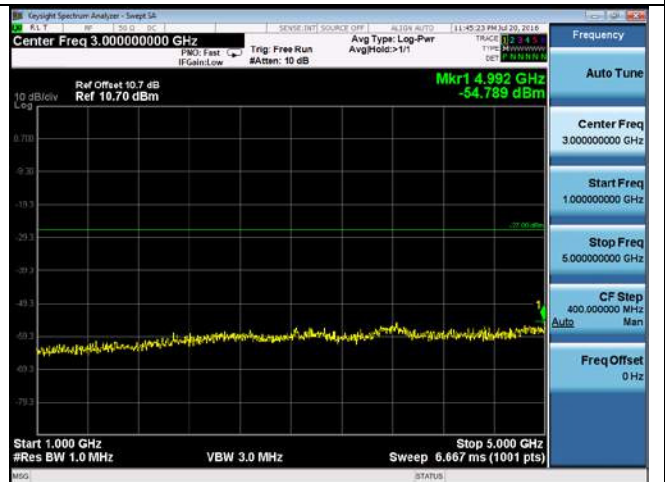
CUE-802.11n-20-5320M-chain 1(1GHz-5GHz)
