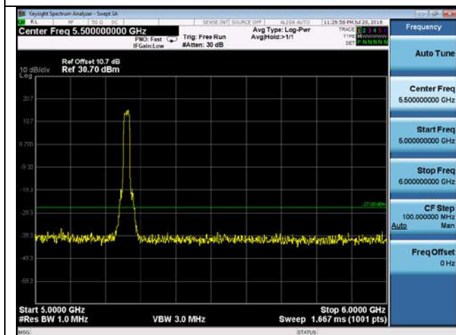
CUE-802.11a-5260M-chain1(5GHz-6GHz)
