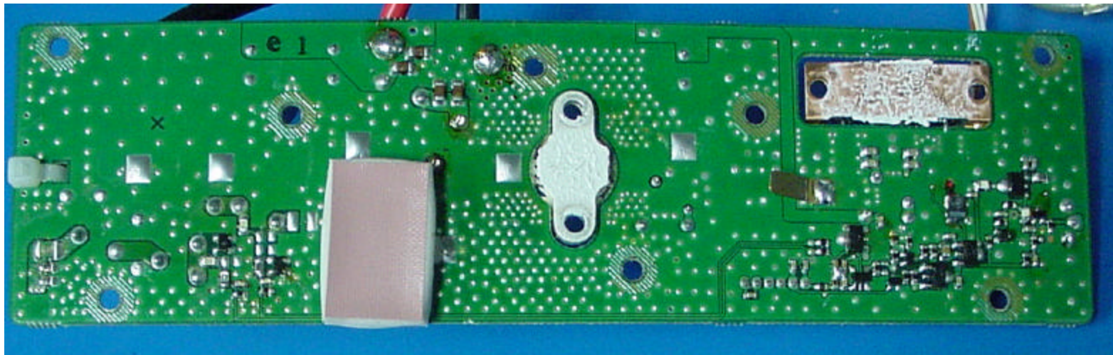
PA-Unit (UHF) PCB solder side
