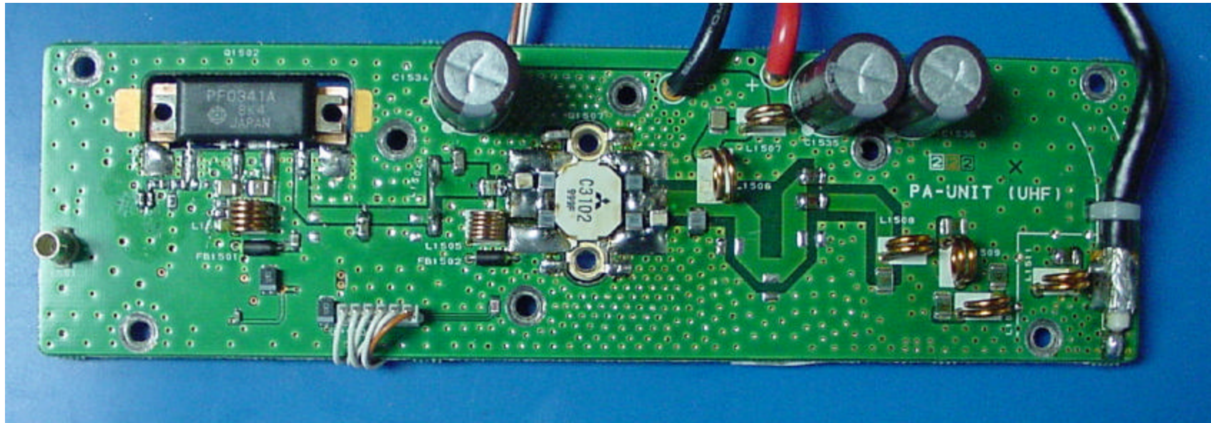
PA Unit (UHF) PCB component side
