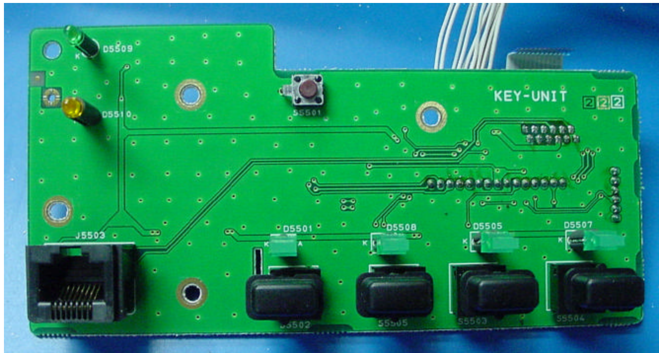
Key-Unit PCB front side
