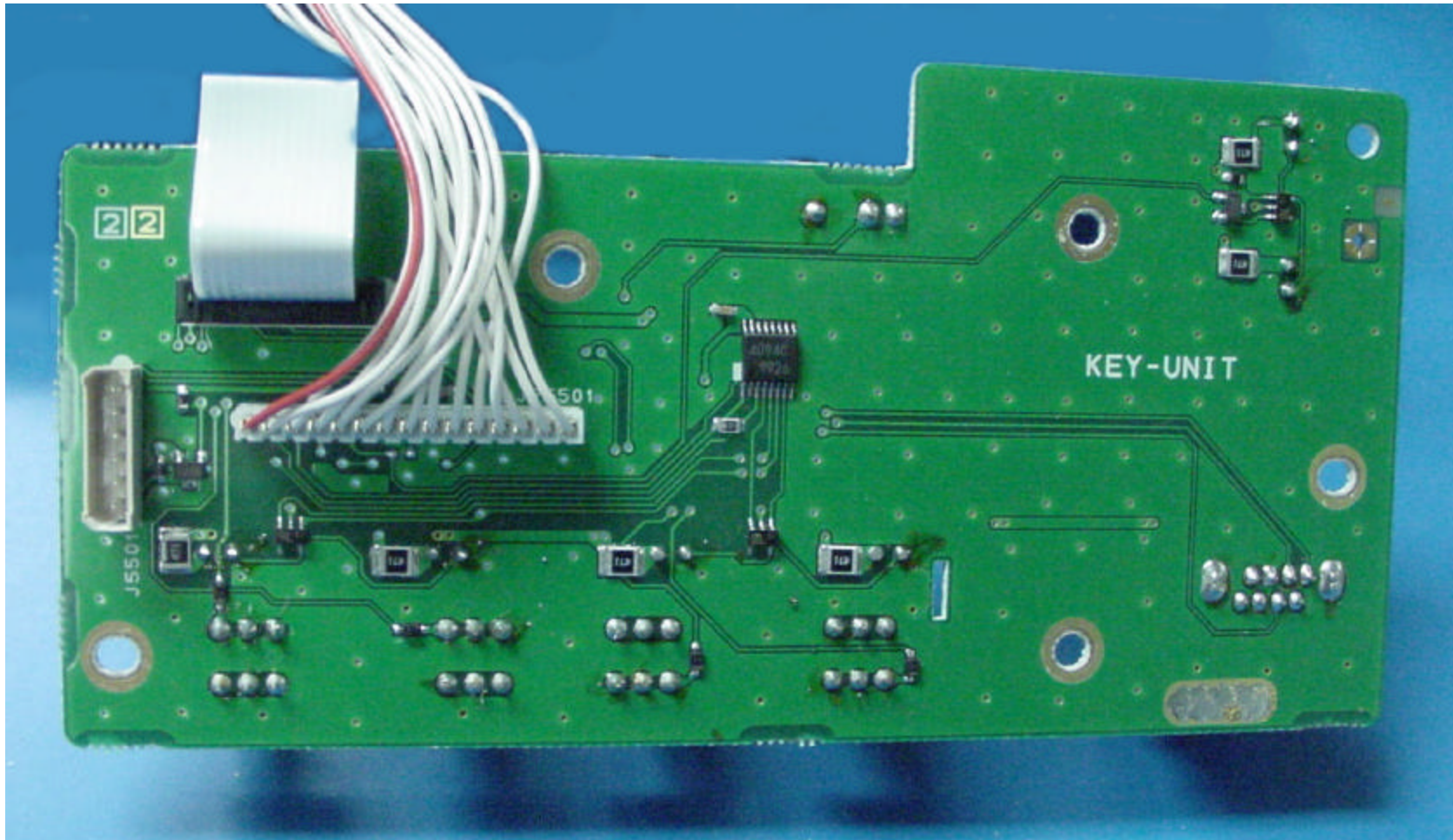
Key-Unit PCB back side
