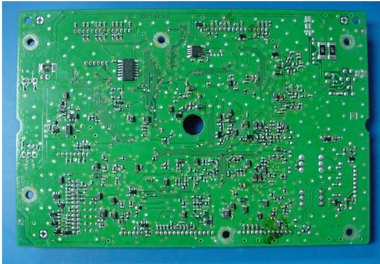
Control Unit PCB solder side
