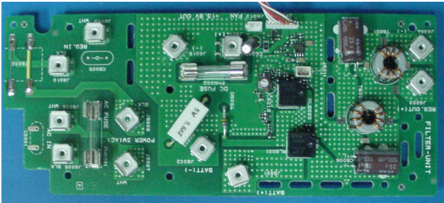
Filter Unit PCB top side
