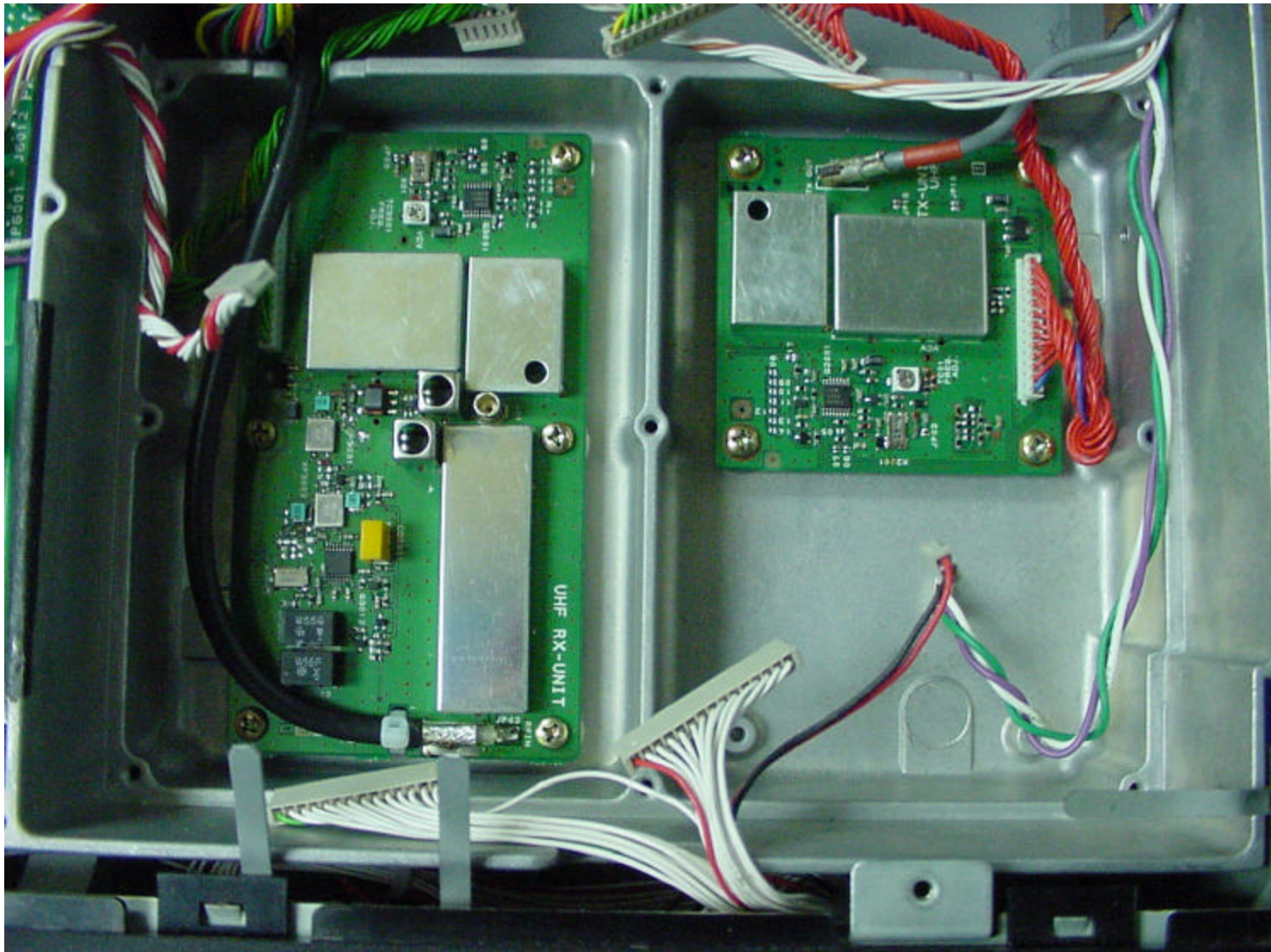
UHF PCB's in chassis
