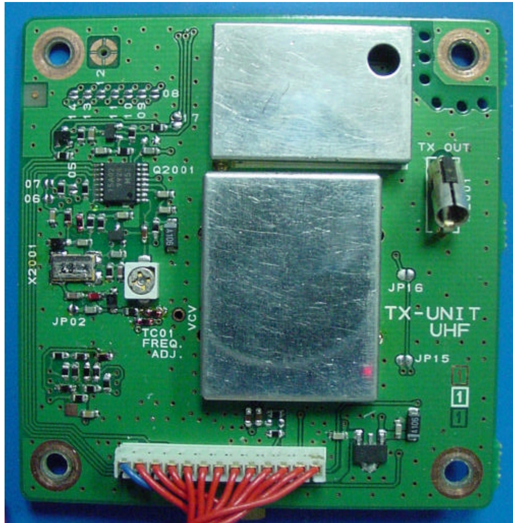
TX-Unit UHF PCBComponent Side
