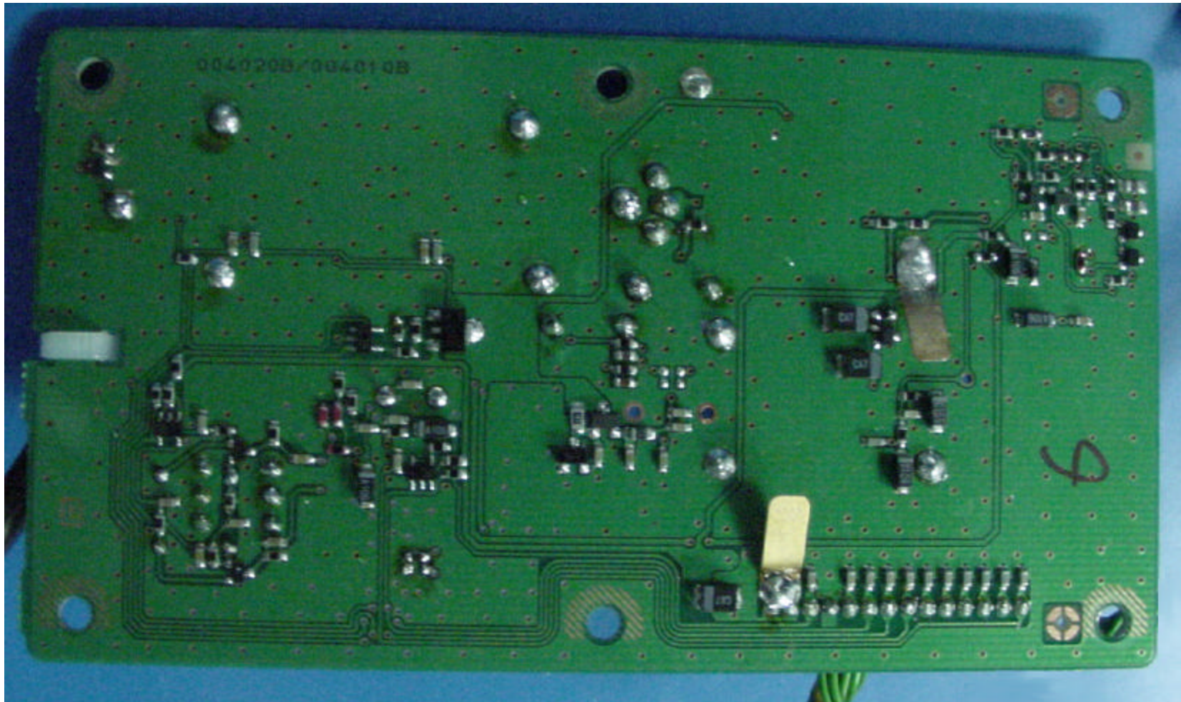
UHF RX-Unit PCB Solder Side
