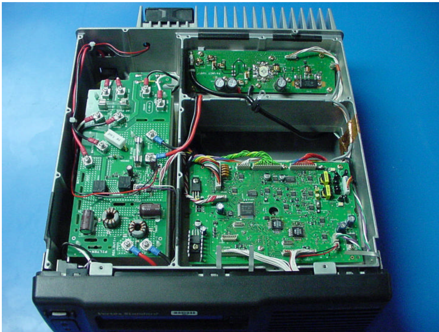
Shields removed from RF and Power compartments
