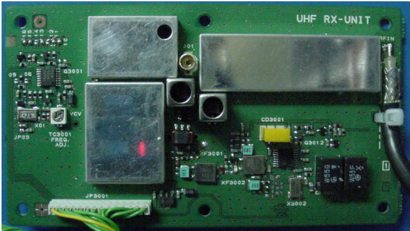
UHF RX-Unit PCB Component Side
