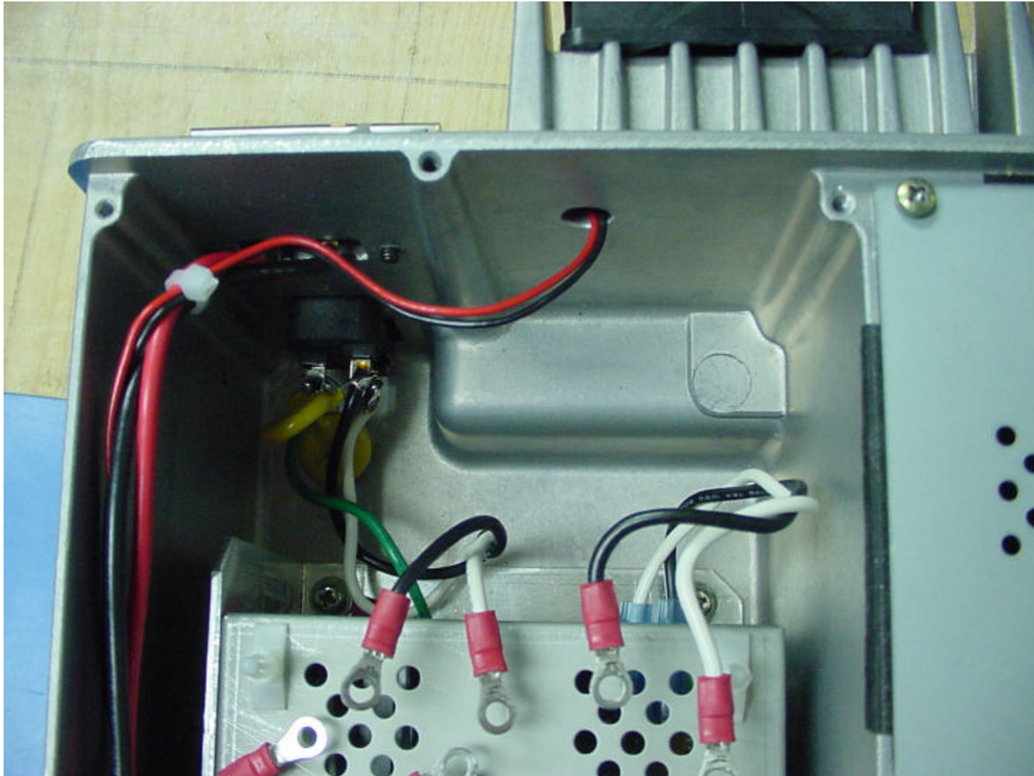
Rear corner connections at power input
