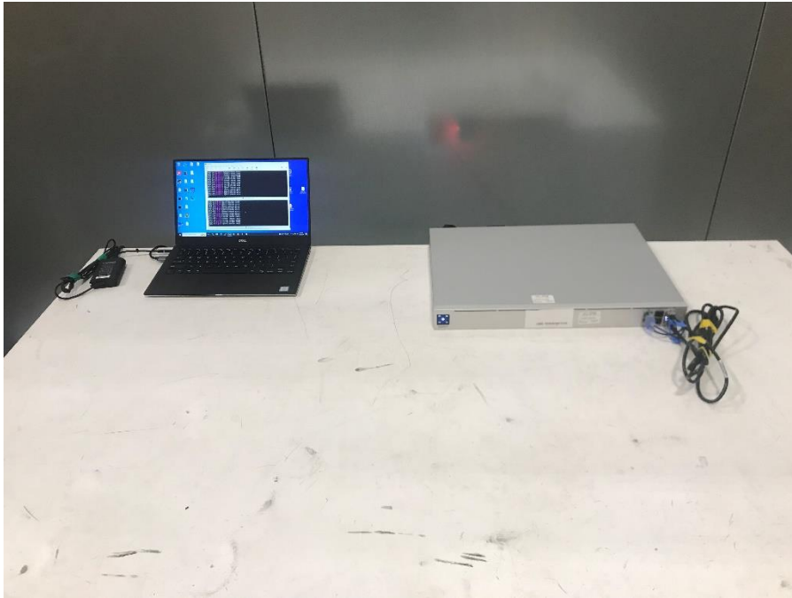
Photograph 5: View Test Set Up Front Conducted Emissions
