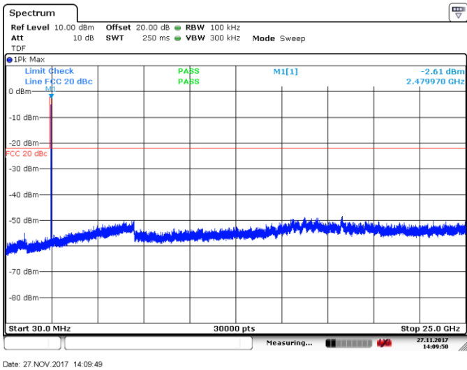
Figure 8.4-10: Conducted spurious emissions outside restricted band, High channel, OQPSK
