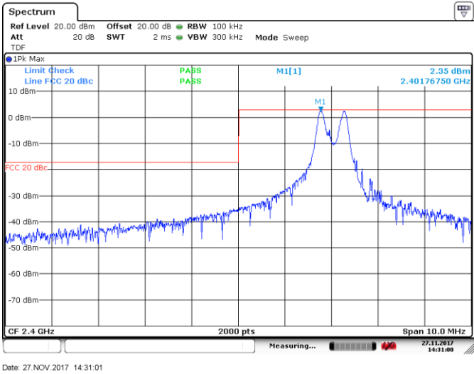
Figure 8.4-1: Conducted spurious emission at band edge outside restricted band, low channel, GFSK
