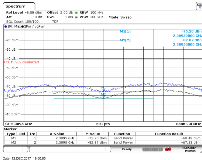
Figure 8.4-19: Conducted spurious emission at band edge of restricted band, low channel, OQPSK
