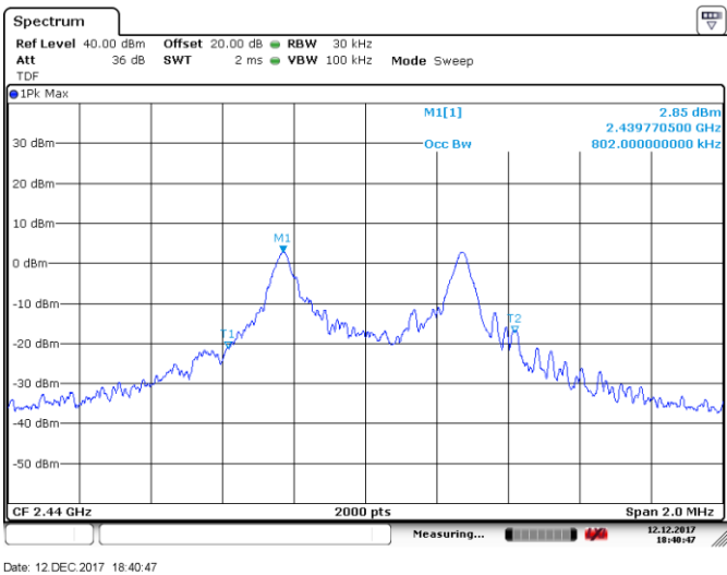
Figure 8.2-8: 99% bandwidth on mid channel, GFSK
