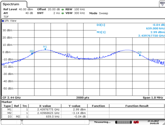
Figure 8.5-2: PSD plot on Mid channel, GFSK
