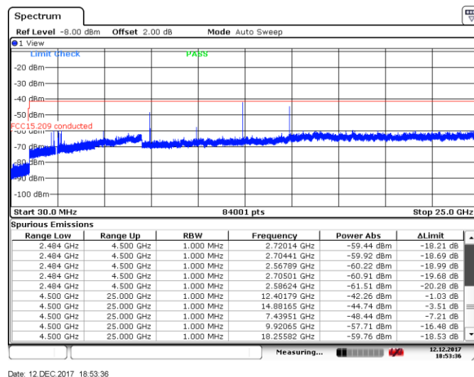
Figure 8.4-13: Conducted spurious emissions within restricted band, High channel, GFSK
