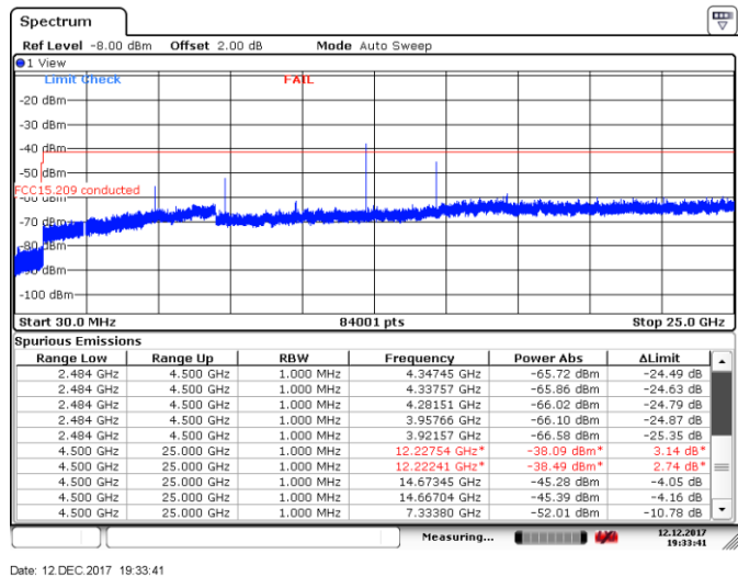
Figure 8.4-15: Conducted spurious emissions within restricted band, Mid channel, OQPSK
