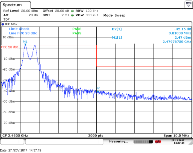
Figure 8.4-2: Conducted spurious emissions at band edge outside restricted band, High channel, GFSK
