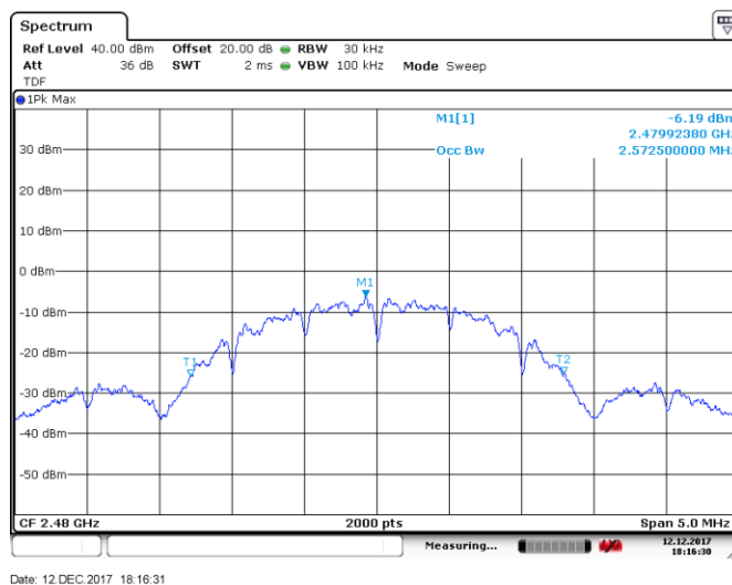
Figure 8.2-12: 99% bandwidth on high channel, OQPSK
