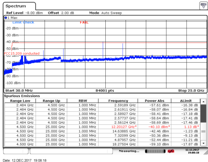
Figure 8.4-12: Conducted spurious emissions within restricted band, Mid channel, GFSK
