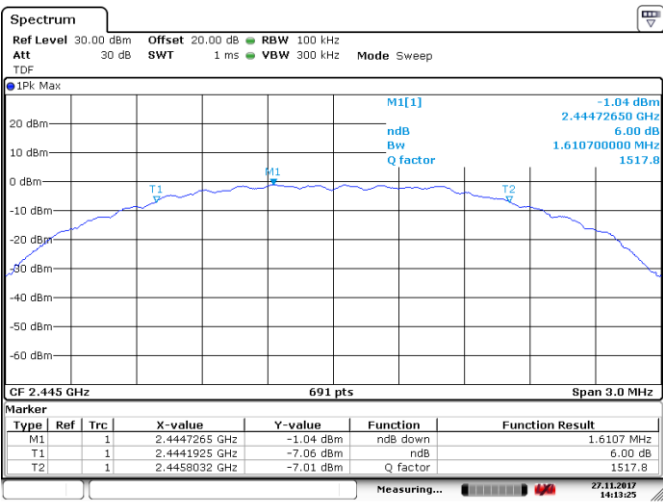
Figure 8.2-5: 6 dB bandwidth on mid channel, OQPSK
