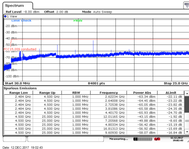
Figure 8.4-11: Conducted spurious emissions within restricted band, Low channel, GFSK
