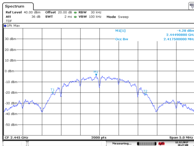
Figure 8.2-11: 99% bandwidth on mid channel, OQPSK
