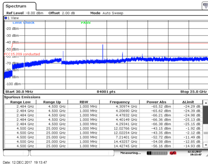
Figure 8.4-14: Conducted spurious emissions within restricted band, Low channel, OQPSK
