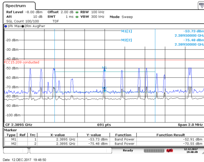
Figure 8.4-17: Conducted spurious emission at band edge of restricted band, low channel, GFSK
