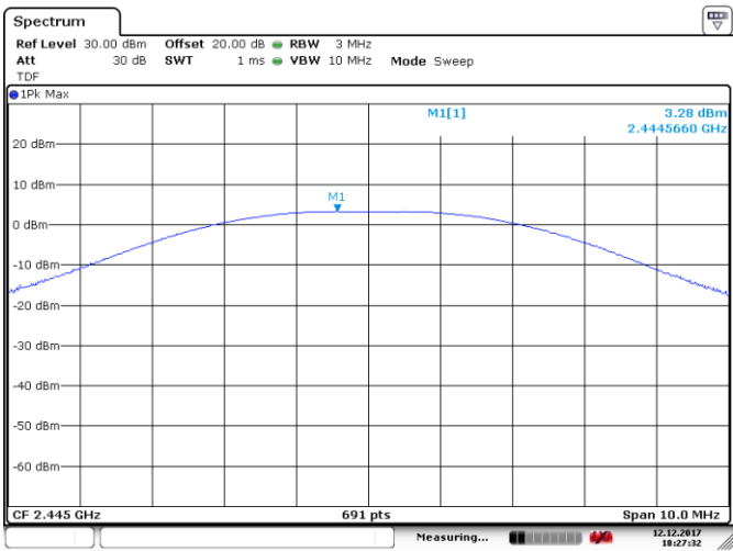
Figure 8.3-5: Output power on mid channel, OQPSK
