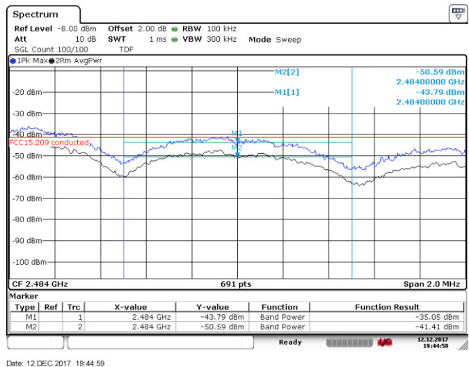
Figure 8.4-20: Conducted spurious emissions at band edge of restricted band, High channel, OQPSK
