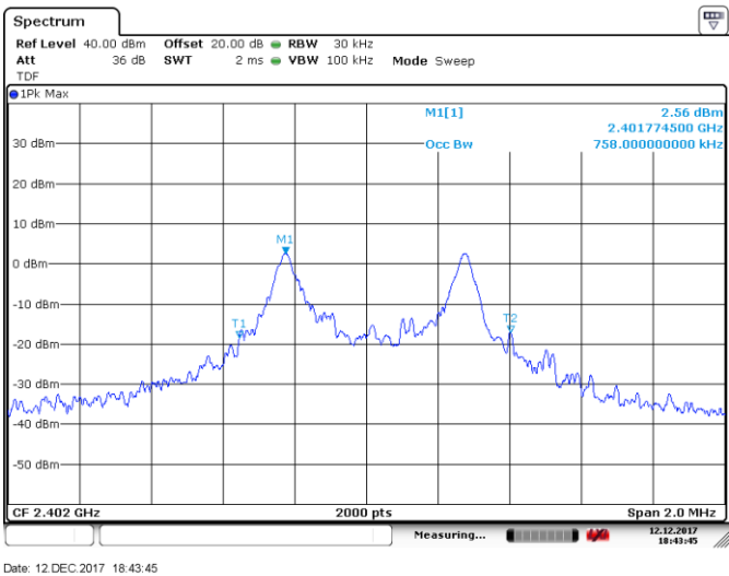
Figure 8.2-7: 99% bandwidth on low channel, GFSK
