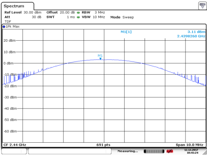
Figure 8.3-2: Output power on mid channel, GFSK
