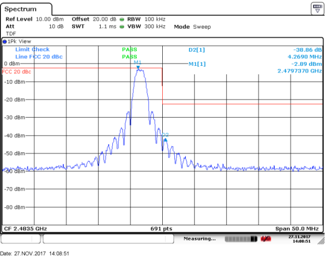
Figure 8.4-4: Conducted spurious emissions at band edge outside restricted band, High channel, OQPSK
