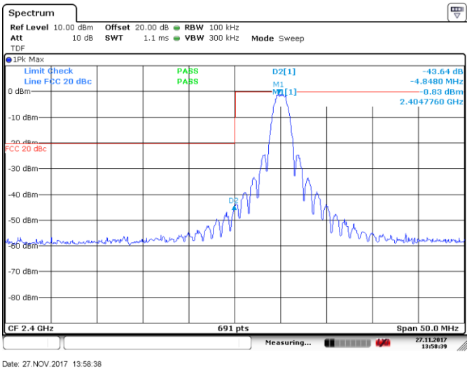
Figure 8.4-3: Conducted spurious emission at band edge outside restricted band, low channel, OQPSK
