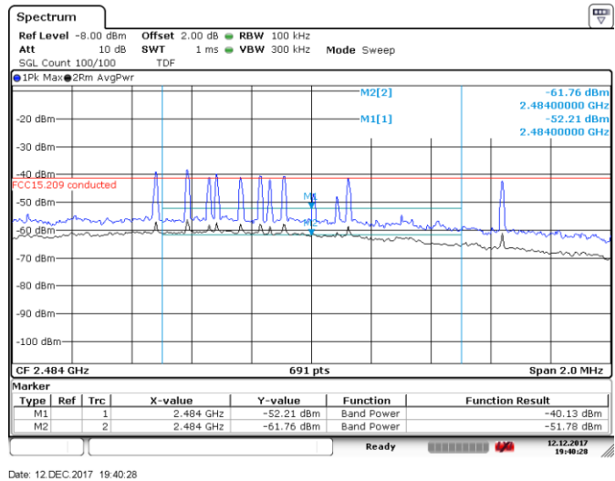
Figure 8.4-18: Conducted spurious emissions at band edge of restricted band, High channel, GFSK
