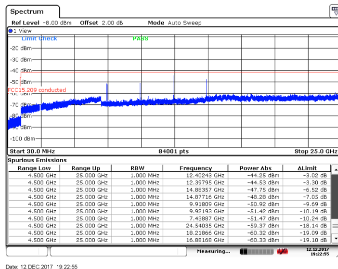
Figure 8.4-16: Conducted spurious emissions within restricted band, High channel, OQPSK
