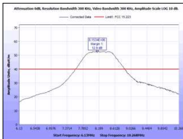
Plot 10. Fundamental Field Strength, NP20, 8.2 MHz, Fundamental Peak
