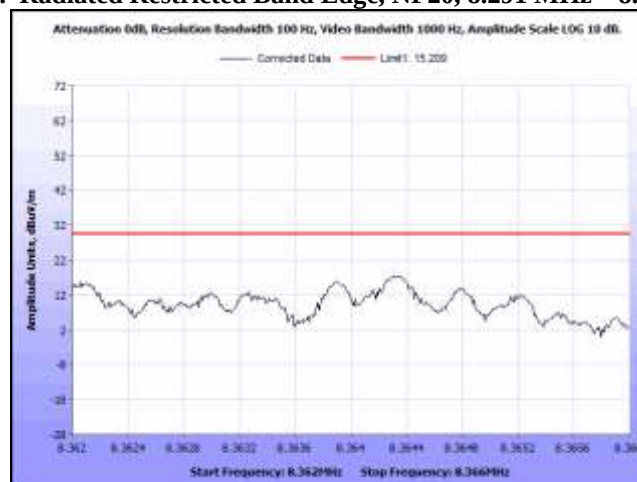
Plot 46. Radiated Restricted Band Edge, NP20, 8.362 MHz – 8.366 MHz
