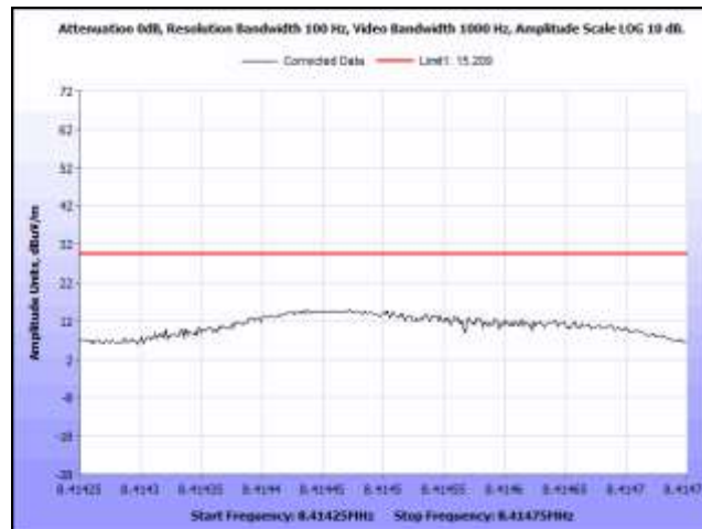
Plot 48. Radiated Restricted Band Edge, NP20, 8.41425 MHz – 8.41475 MHz
