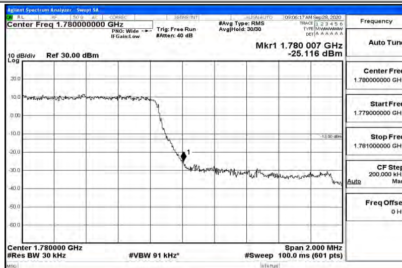
Band66-1.4MHz-16QAM-131979-6RB#0
