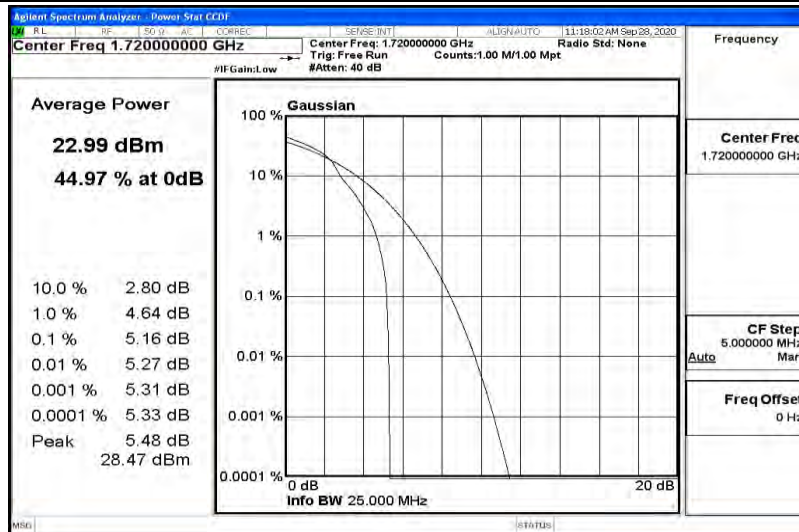
Band66-20MHz-16QAM-132072-100RB#0
