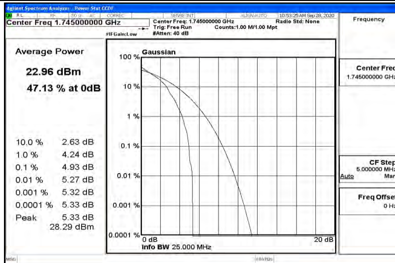
Band66-15MHz-QPSK-132322-75RB#0
