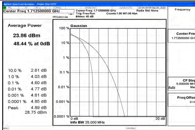
Band66-5MHz-QPSK-131997-25RB#0
