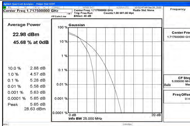
Band66-15MHz-QPSK-132047-75RB#0
