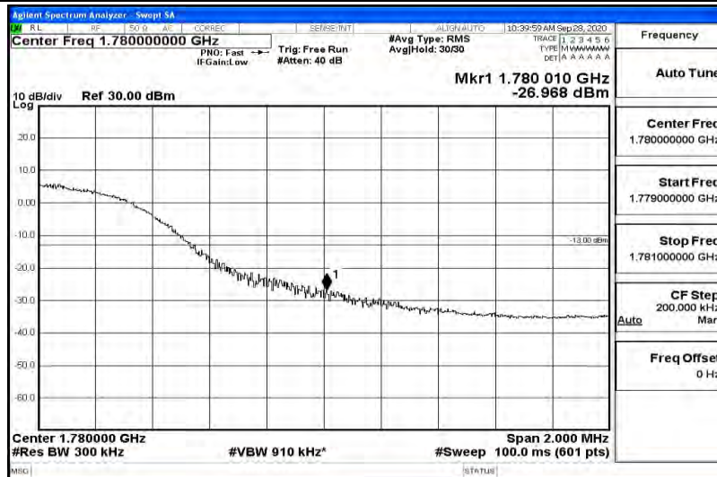
Band66-20MHz-QPSK-132072-100RB#0
