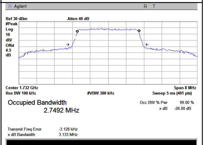
LTE Band IV - Middle CH 16QAM-3
