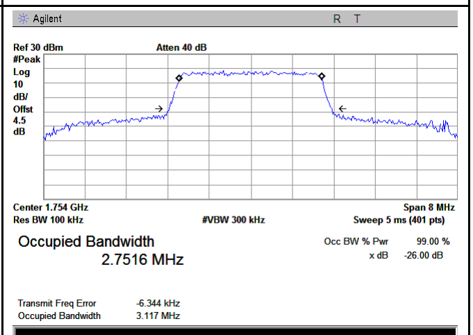
LTE Band IV - High CH 16QAM-3
