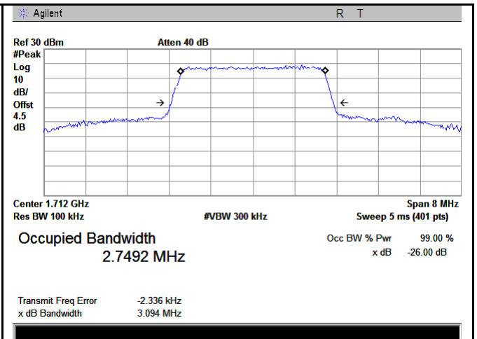
LTE Band IV - Low CH 16QAM-3
