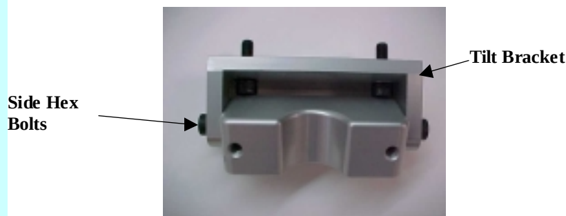
Figure 6-8 Tilt Bracket
