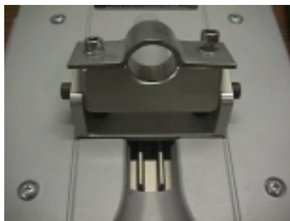
Figure 6-9 AB-Access Extender with Mounted Tilt Bracket
