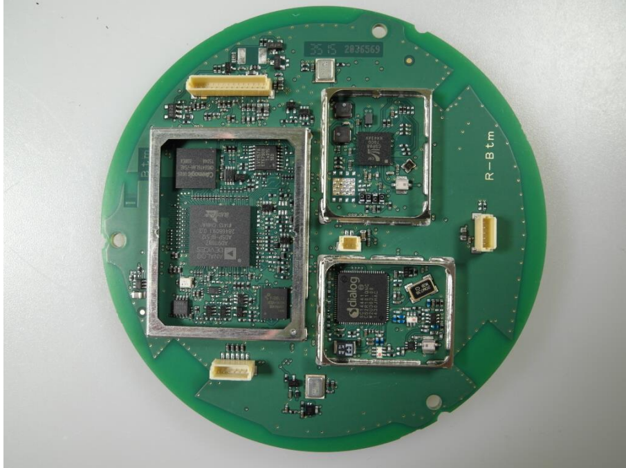
Photo 5: backside main layer without shielding
