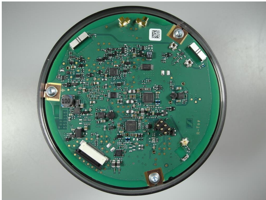
Photo 2: main layer with RF ports and antennas
