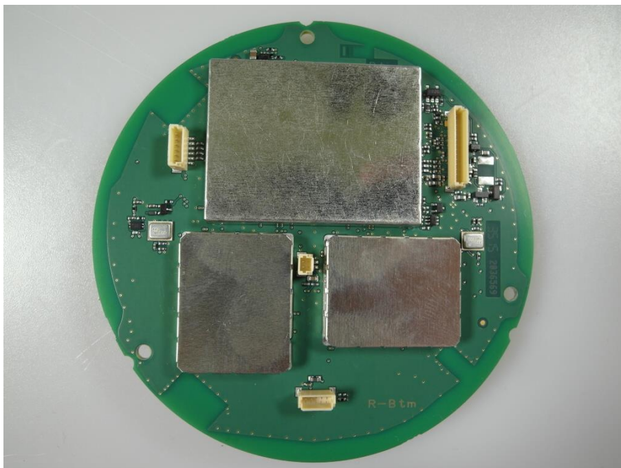
Photo 4: backside of the main layer
