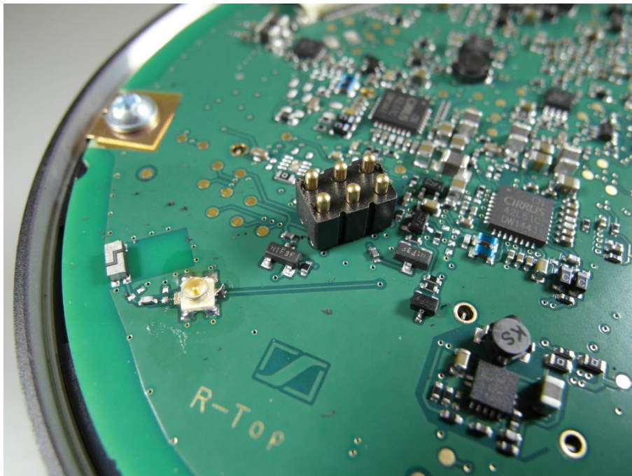
Photo 3: RF port and antenna for BT technology
