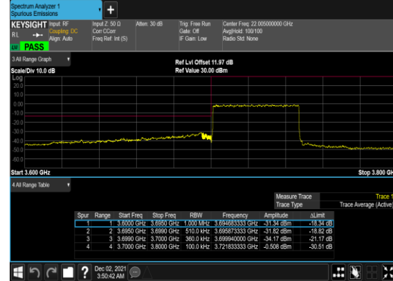
B41_N77(50M)_DFT-s- OFDM_QPSK_Outer_Full_Low_CH
