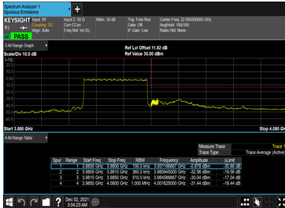
B41_N77(50M)_DFT-s- OFDM_BPSK_Outer_Full_High_CH
