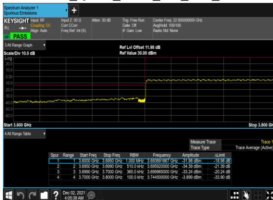
B41_N77(100M)_DFT-s- OFDM_QPSK_Outer_Full_Low_CH
