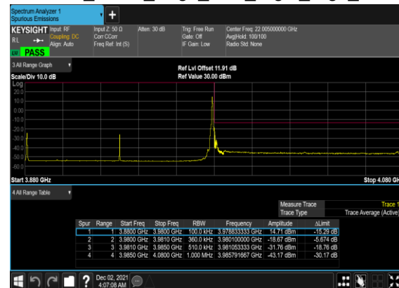
B41_N77(100M)_DFT-s- OFDM_BPSK_Edge_1RB_Right_High_CH
