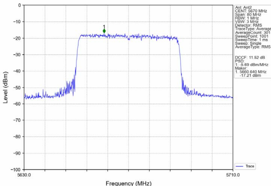
802.11ax(HEW40)_HCH_5670MHz_RU484_Left_Ant2_NTNV
