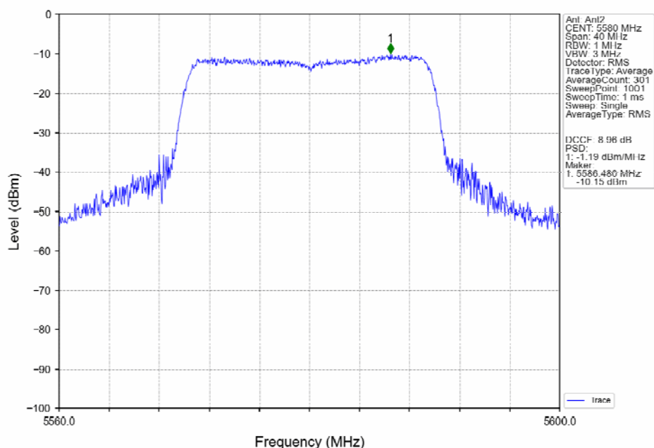
802.11ax(HEW20)_MCH_5580MHz_RU242_Left_Ant2_NTNV
