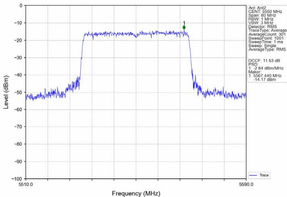
802.11ax(HEW40)_MCH_5550MHz_RU484_Left_MIMO_NTNV
