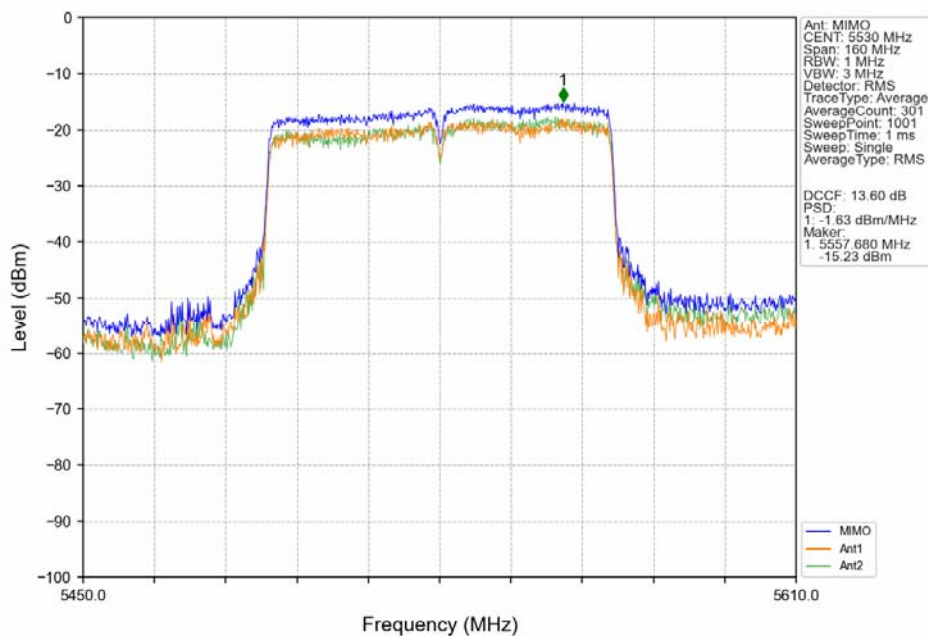
802.11ac(VHT80)_LCH_5530MHz_MIMO_NTNV
