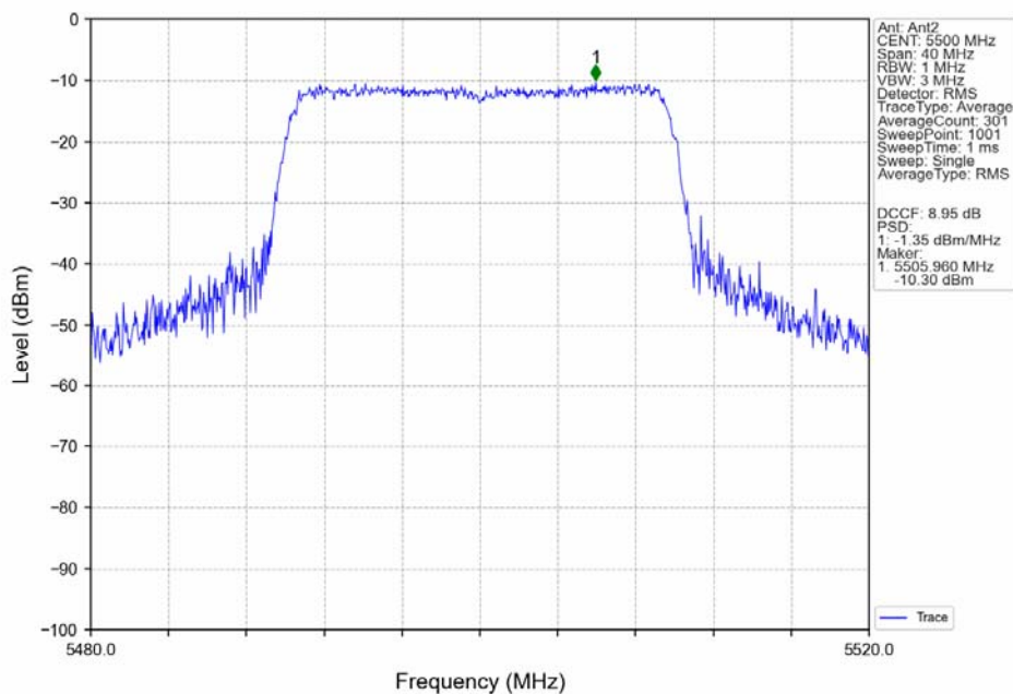
802.11ax(HEW20)_LCH_5500MHz_RU242_Left_MIMO_NTNV
