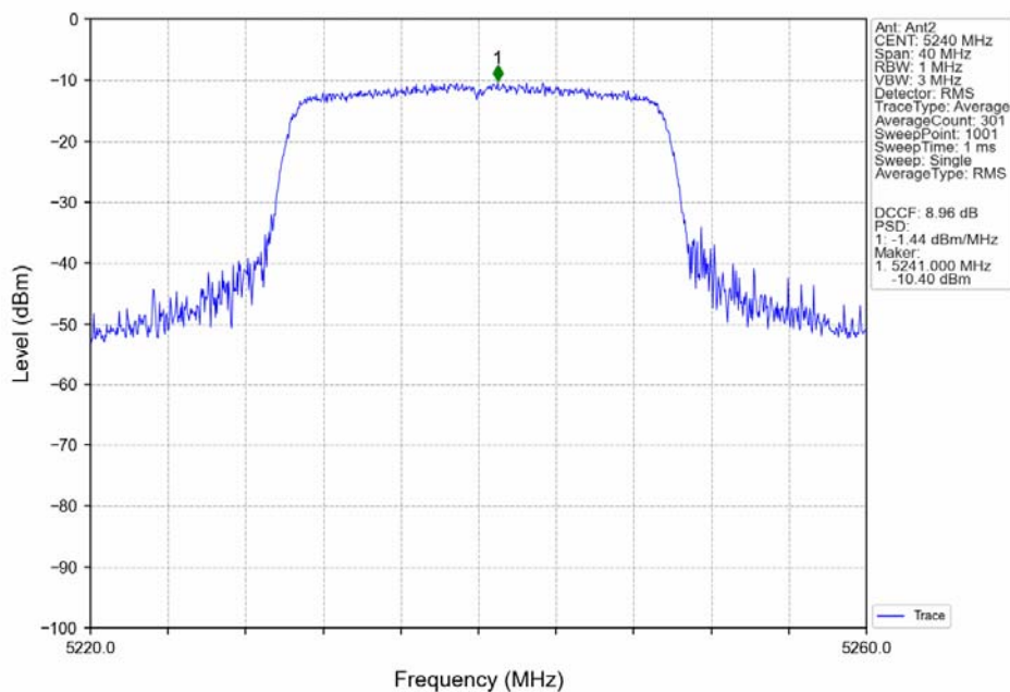
802.11ax(HEW20)_HCH_5240MHz_RU242_Left_MIMO_NTNV
