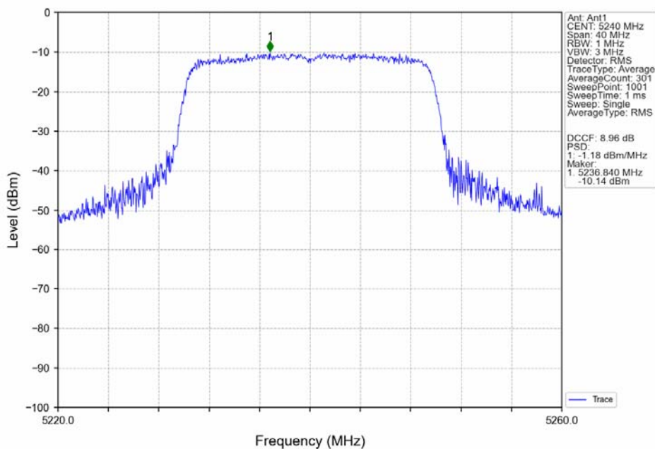
802.11ax(HEW20)_HCH_5240MHz_RU242_Left_Ant1_NTNV
