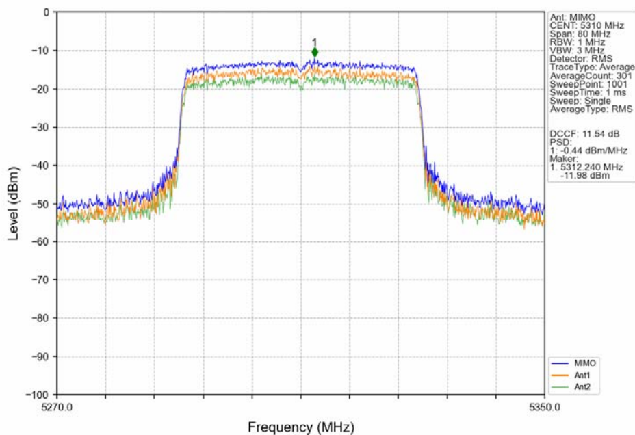
802.11ax(HEW40)_HCH_5310MHz_RU484_Left_MIMO_NTNV
