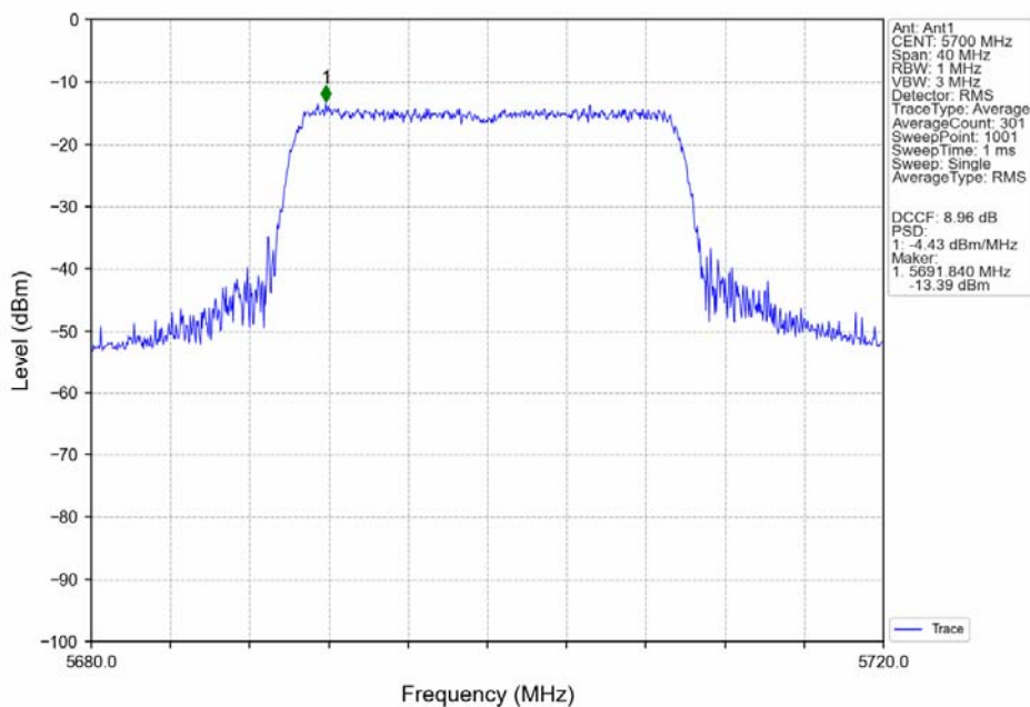
802.11ax(HEW20)_HCH_5700MHz_RU242_Left_Ant1_NTNV
