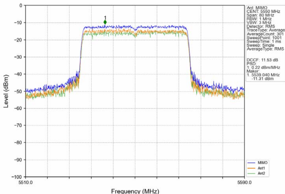
802.11ax(HEW40)_MCH_5550MHz_RU484_Left_MIMO_NTNV
