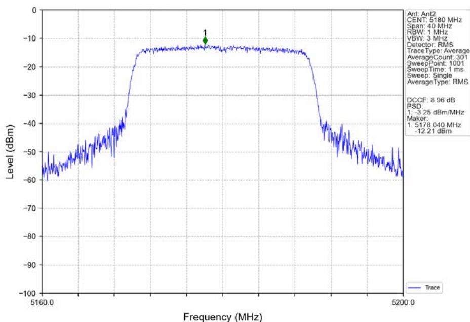
802.11ax(HEW20)_LCH_5180MHz_RU242_Left_MIMO_NTNV
