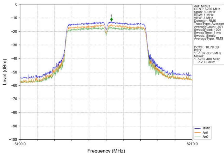
802.11n(HT40)_HCH_5230MHz_MIMO_NTNV
