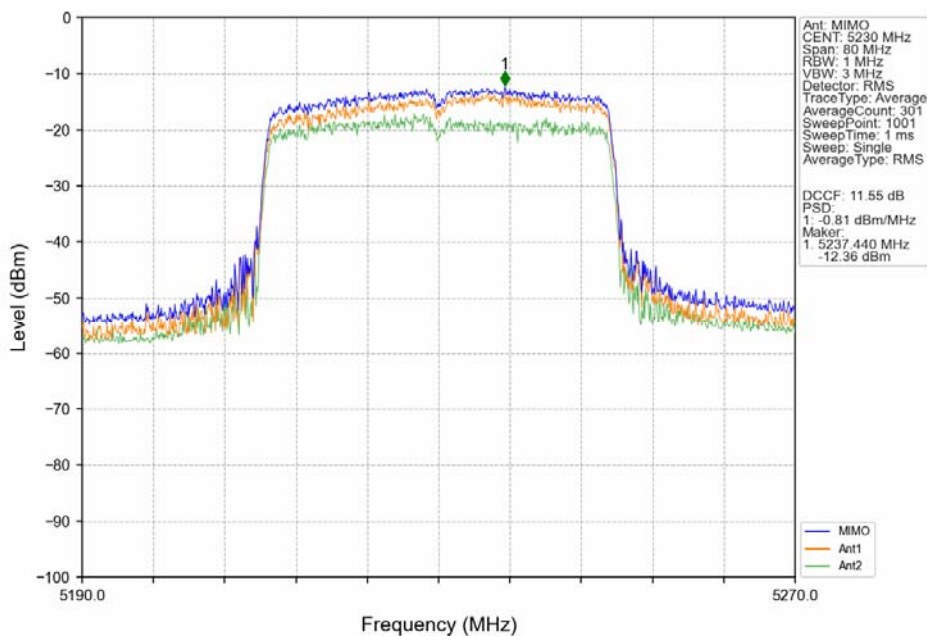
802.11ax(HEW40)_HCH_5230MHz_RU484_Left_MIMO_NTNV
