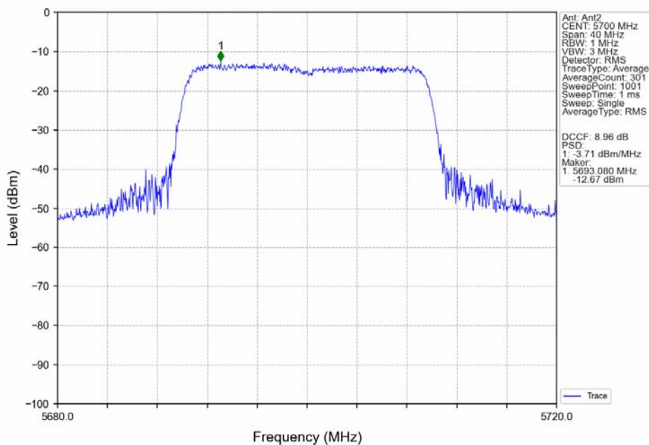
802.11ax(HEW20)_HCH_5700MHz_RU242_Left_MIMO_NTNV
