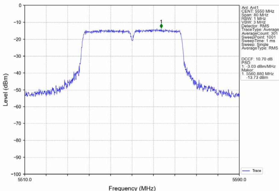
802.11n(HT40)_MCH_5550MHz_Ant1_NTNV
