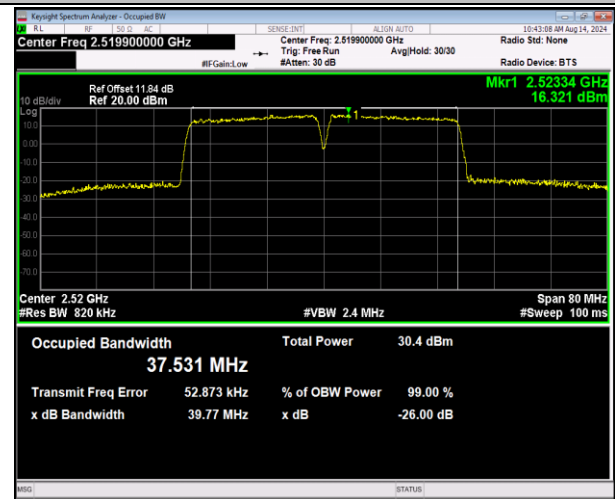
7-7-20MHz-20MHz-QPSK-QPSK-20850-21048-100RB#0-100RB#0-PASS
