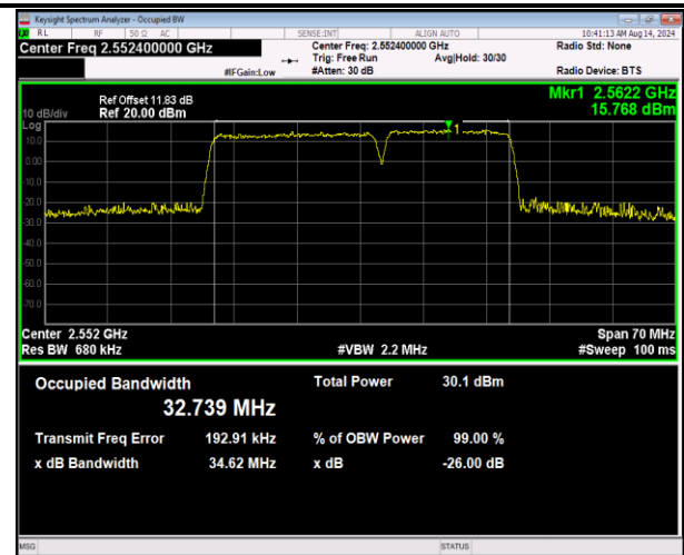
7-7-20MHz-15MHz-16QAM-16QAM-21201-21372-100RB#0-75RB#0-PASS
