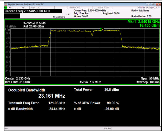
7-7-15MHz-10MHz-QPSK-QPSK-21051-21171-75RB#0-50RB#0-PASS
