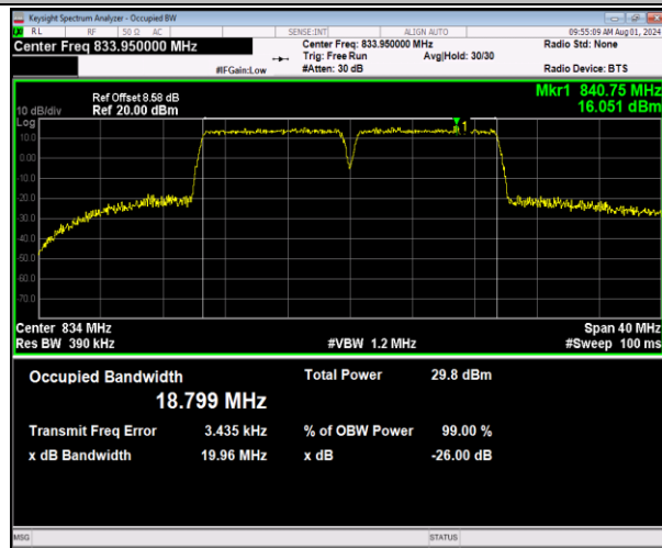
5-5-10MHz-10MHz-64QAM-64QAM-20450-20549-50RB#0-5 0-50RB#0-PASS
