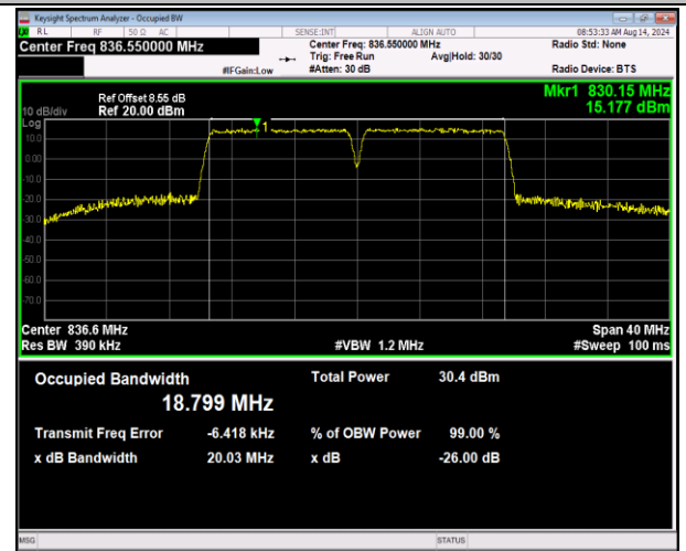
5-5-10MHz-10MHz-QPSK-QPSK-20476-20575-50RB#0-5 50RB#0-PASS
