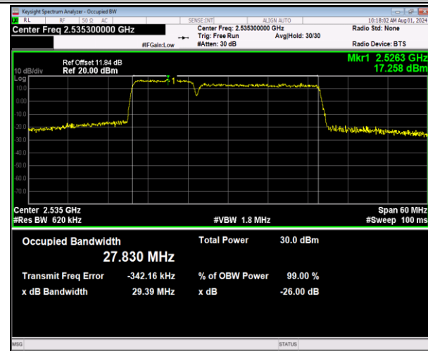
7-7-10MHz-20MHz-64QAM-64QAM-21006-21150-50RB# 0-100RB#0-PASS
