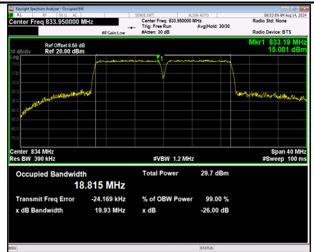
5-5-10MHz-10MHz-16QAM-16QAM-20450-20549-50RB#0-5 #0-50RB#0-PASS
