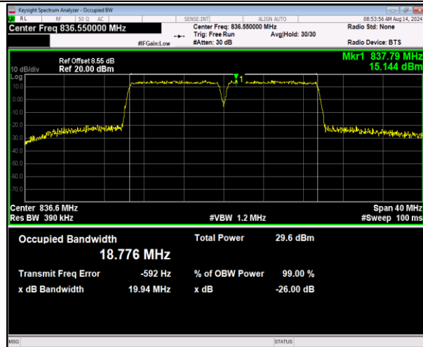
5-5-10MHz-10MHz-16QAM-16QAM-20476-20575-50RB#0-5 0-50RB#0-PASS
