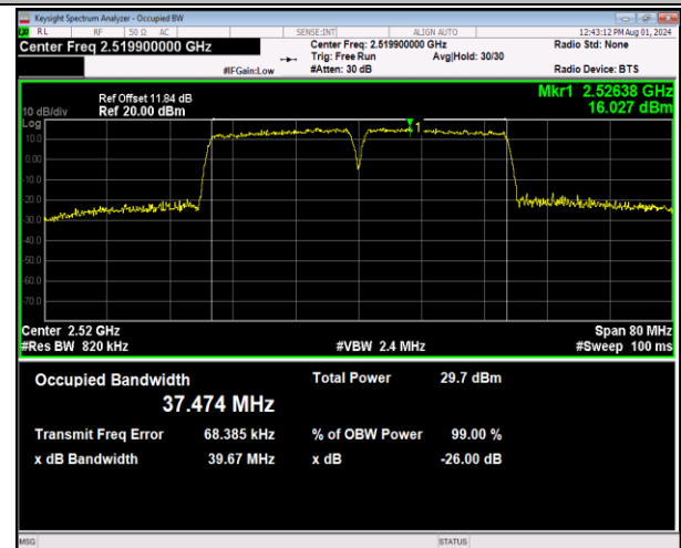
7-7-20MHz-20MHz-64QAM-64QAM-20850-21048-100RB#0-100RB#0-PASS
