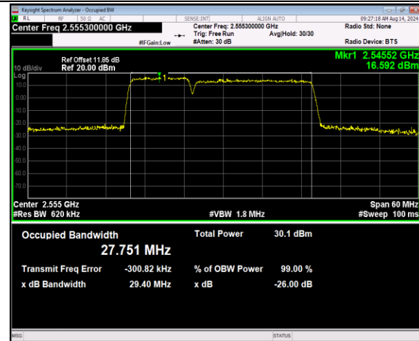
7-7-10MHz-20MHz-16QAM-16QAM-21206-21350-50RB# 0-100RB#0-PASS
