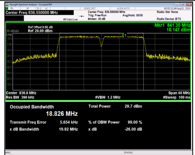
5-5-10MHz-10MHz-64QAM-64QAM-20476-20575-50RB#0-5 #0-50RB#0-PASS
