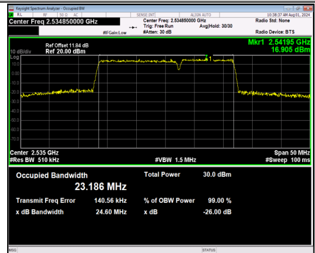
7-7-15MHz-10MHz-64QAM-64QAM-21051-21171-75RB#0-50RB#0-PASS
