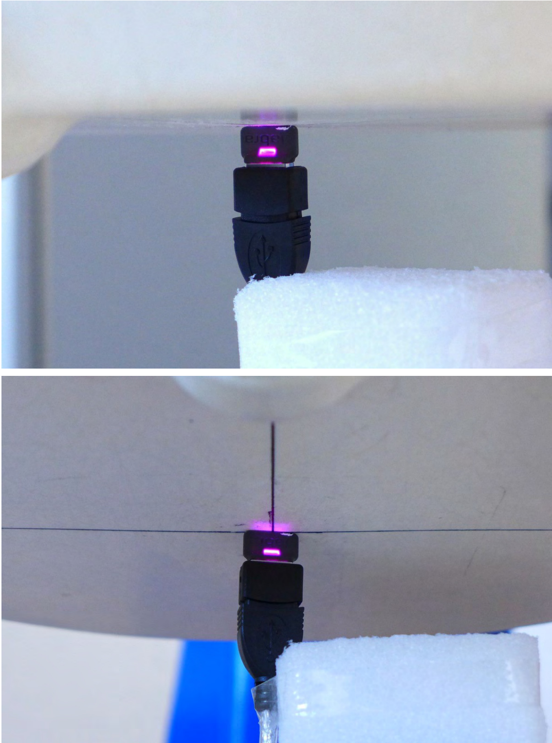
Pic. 7: Test position 5 – top side, 0mm distance to phantom.
