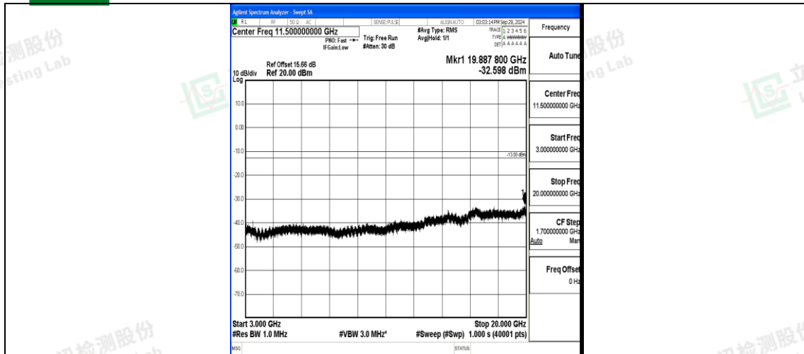
Band4_15MHz_QPSK_20175_1RB#0_3000~20000_3000~20000
