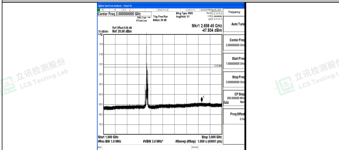
Band4_15MHz_QPSK_20175_1RB#0_1000~3000_1000~3000
