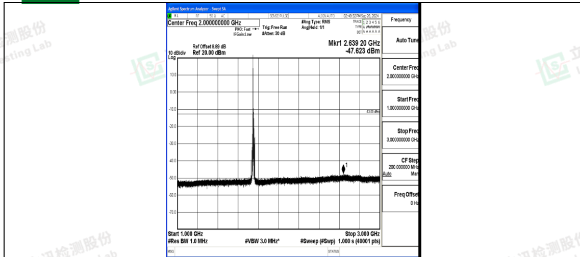
Band4_10MHz_16QAM_20350_1RB#0_1000~3000_1000~3000
