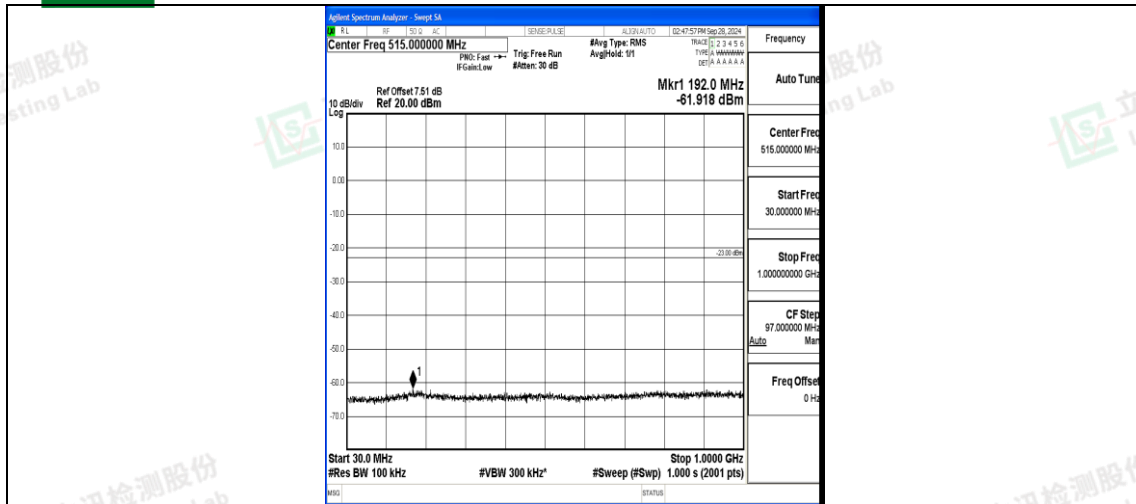
Band4_10MHz_QPSK_20350_1RB#0_30~1000_30~1000
