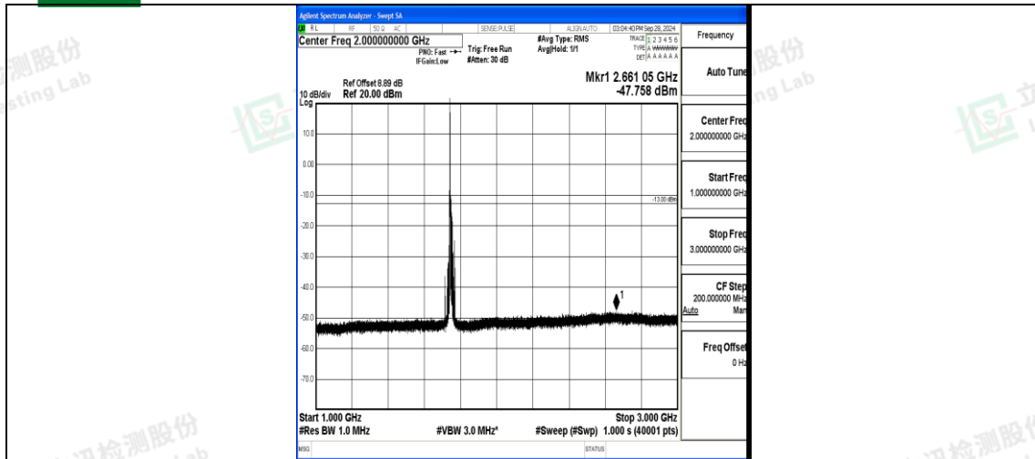
Band4_15MHz_16QAM_20325_1RB#0_1000~3000_1000~3000
