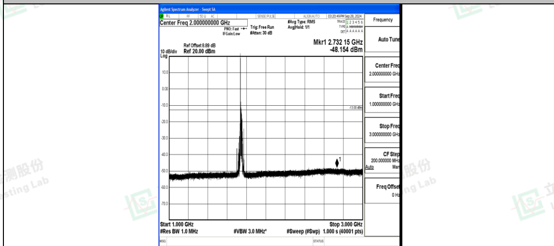
Band4_20MHz_16QAM_20300_1RB#0_1000~3000_1000~3000
