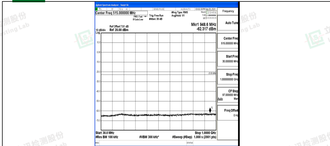
Band4_15MHz_16QAM_20025_1RB#0_30~1000_30~1000
