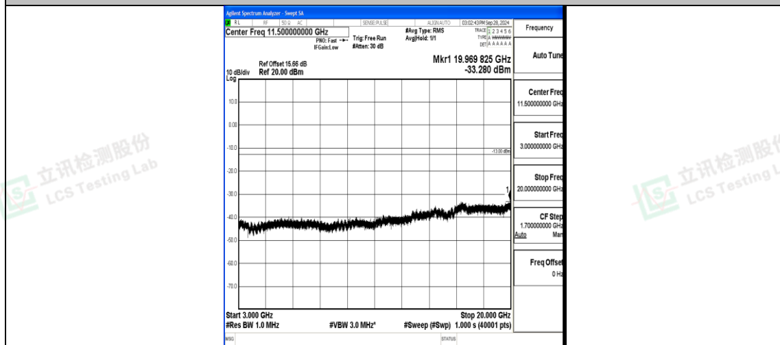
Band4_15MHz_16QAM_20025_1RB#0_3000~20000_3000~20000
