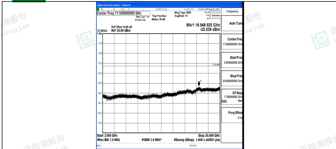
Band4_15MHz_QPSK_20025_1RB#0_3000~20000_3000~20000
