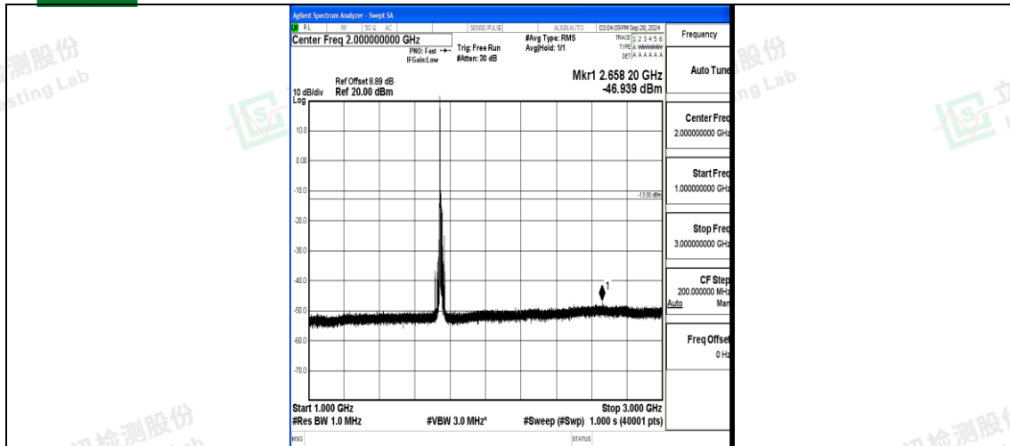
Band4_15MHz_QPSK_20325_1RB#0_1000~3000_1000~3000
