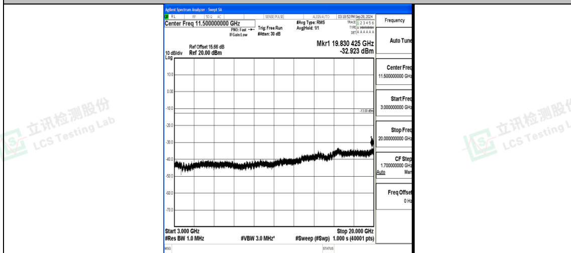
Band4_20MHz_16QAM_20050_1RB#0_3000~20000_3000~20000
