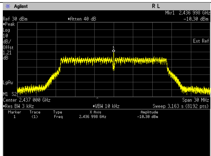
Maximum Power Spectral Density. 802.11g Frequency 2437 MHz
