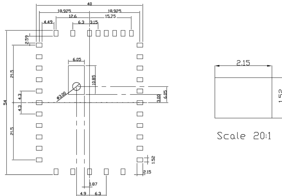
Figure 4: Recommend Footprint
