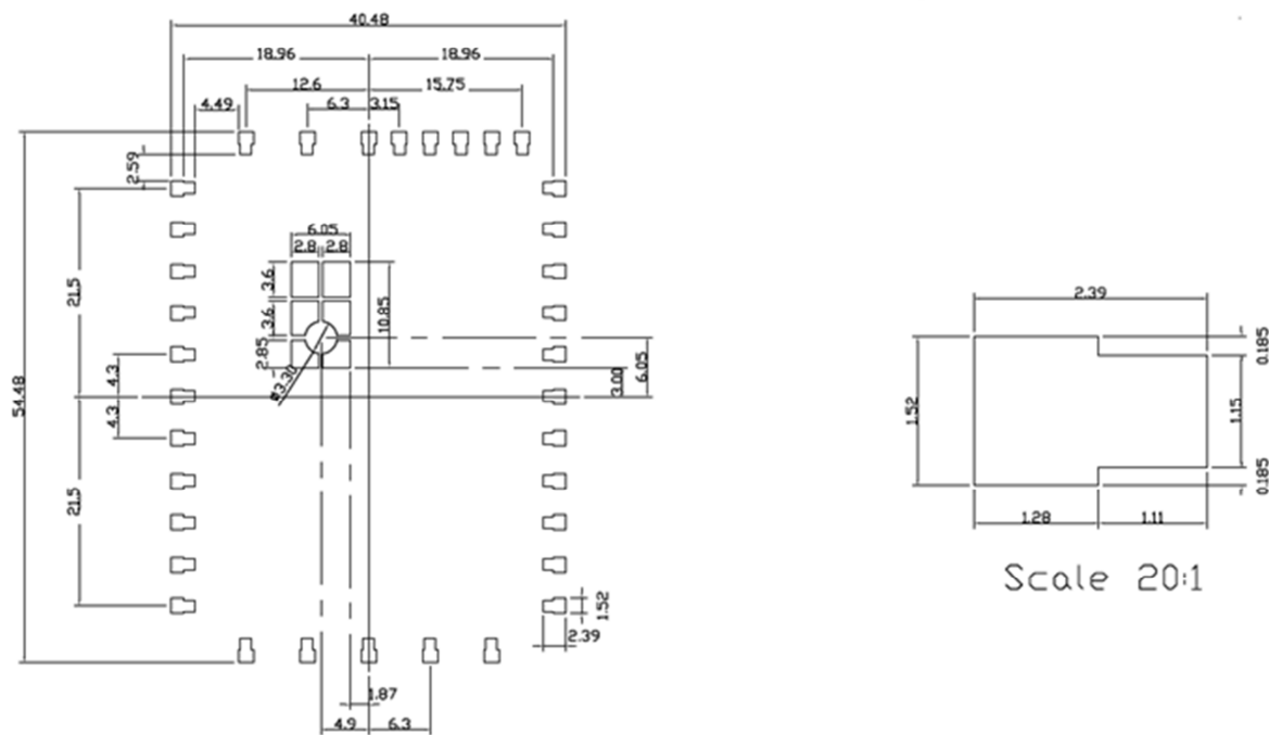
Figure 5: Recommend Stencil
