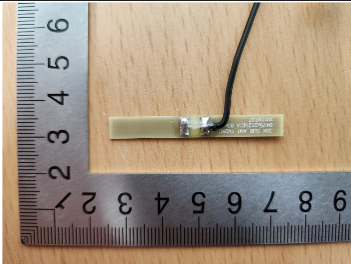
MESH Antenna 2 (LEFT)
