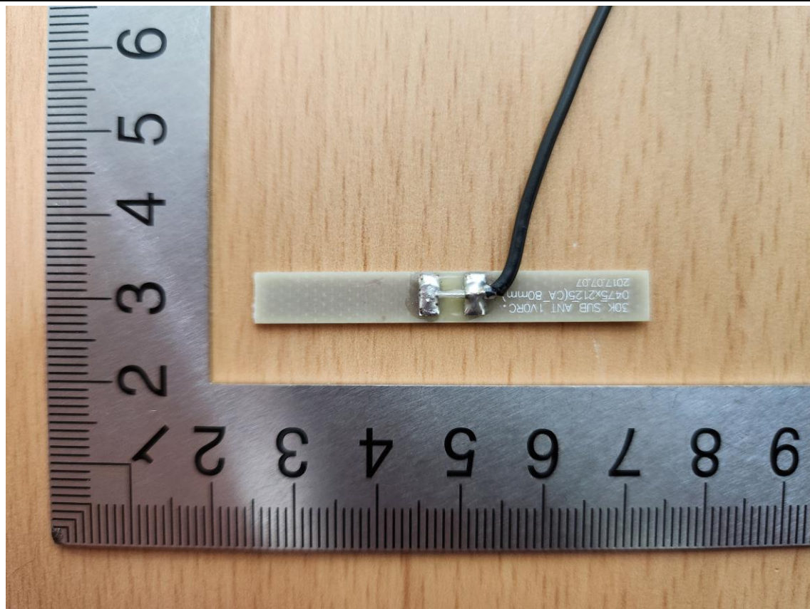
MESH Antenna 1 (RIGHT)
