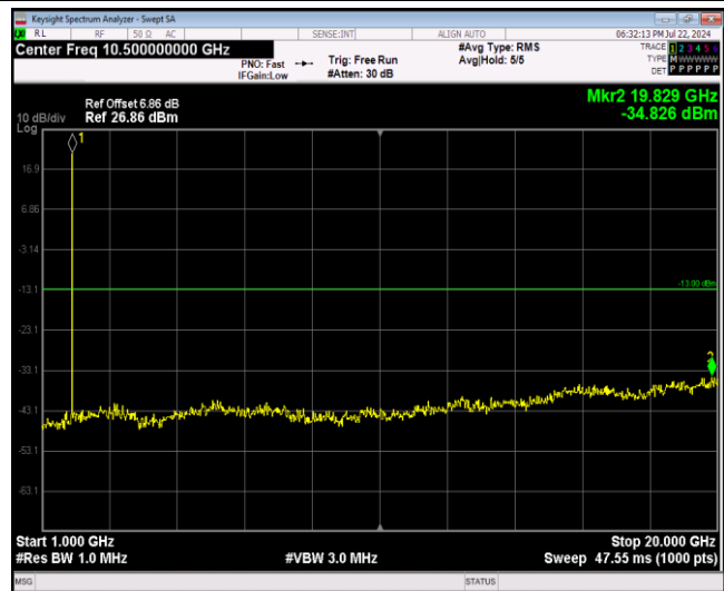
Band2-1.4MHz-64QAM-18900-1RB#0-Range2:1000~20 000MHz
