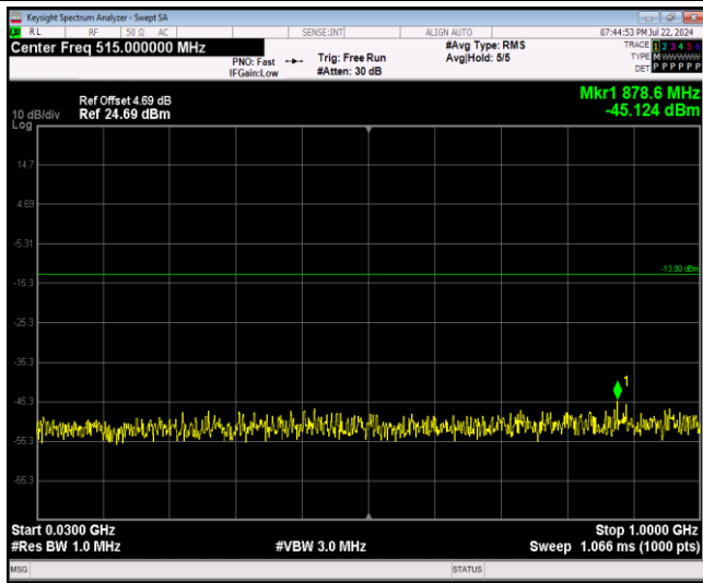
Band4-20MHz-64QAM-20175-1RB#0-Range1:30~1000MHz
