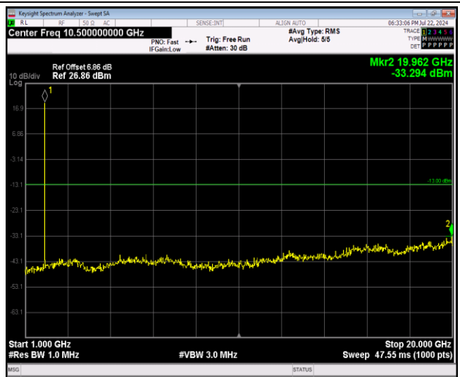
Band2-1.4MHz-64QAM-19193-1RB#0-Range2:1000~20000MHz
