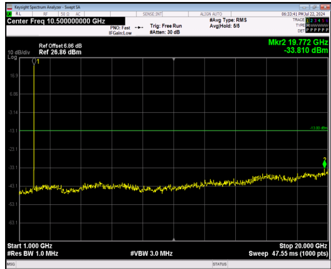
Band2-1.4MHz-64QAM-18607-1RB#0-Range2:1000~20 000MHz
