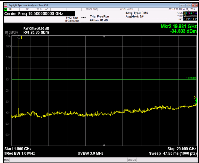
Band4-1.4MHz-64QAM-19957-1RB#0-Range2:1000~20000MHz
