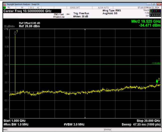
Band4-1.4MHz-64QAM-20393-1RB#0-Range2:1000~20 000MHz
