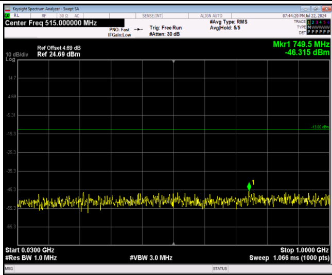
Band4-20MHz-QPSK-20300-1RB#0-Range1:30~100 OMHz
