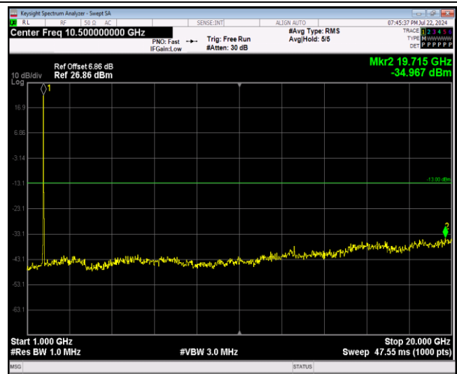
Band4-20MHz-64QAM-20050-1RB#0-Range2:1000~20000MHz
