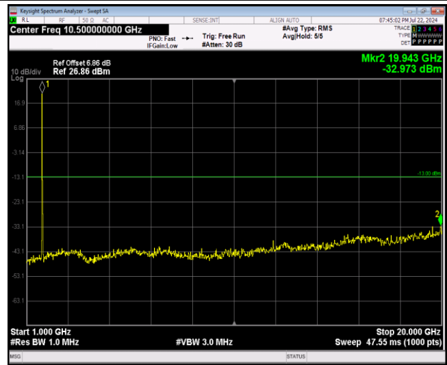
Band4-20MHz-64QAM-20175-1RB#0-Range2:1000~20000MHz
