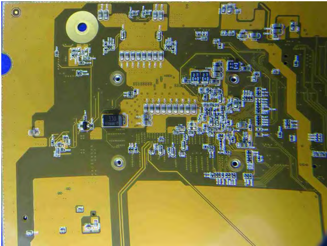
(42) EUT Photo
