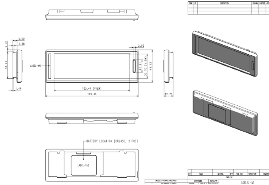
Figure 3 Mechanical Dimension
