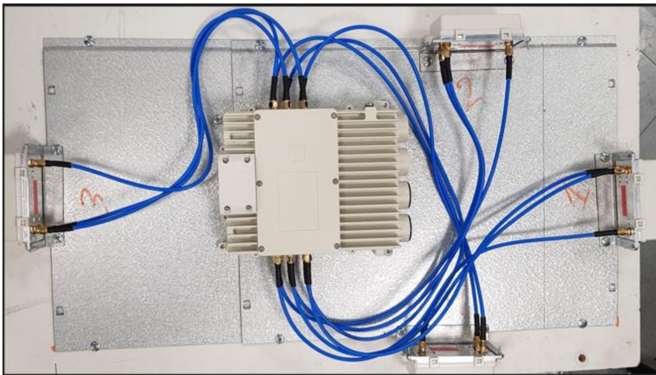
Photograph No.1 MH-N880-CCP-PoE front view
