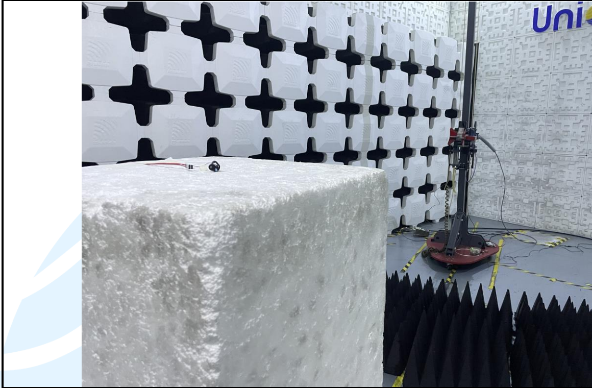
Radiated emission Test Setup (Above 1 GHz) _ Left Ear
