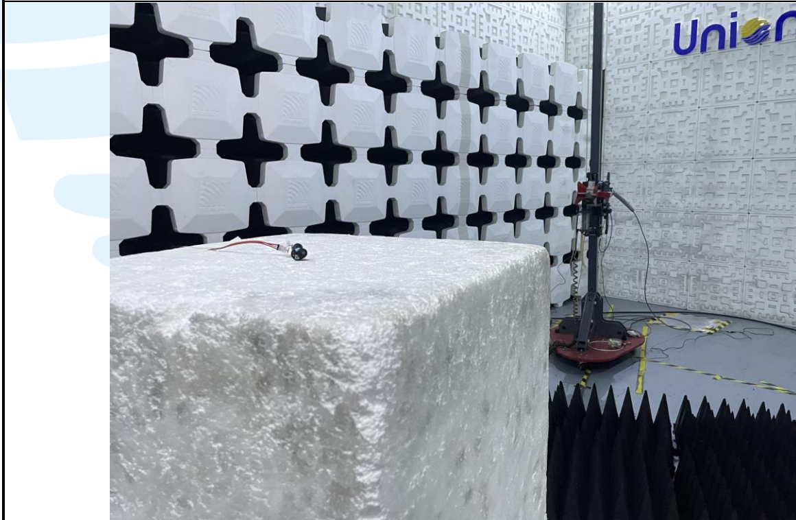
Radiated emission Test Setup (Above 1 GHz) _ Right Ear
