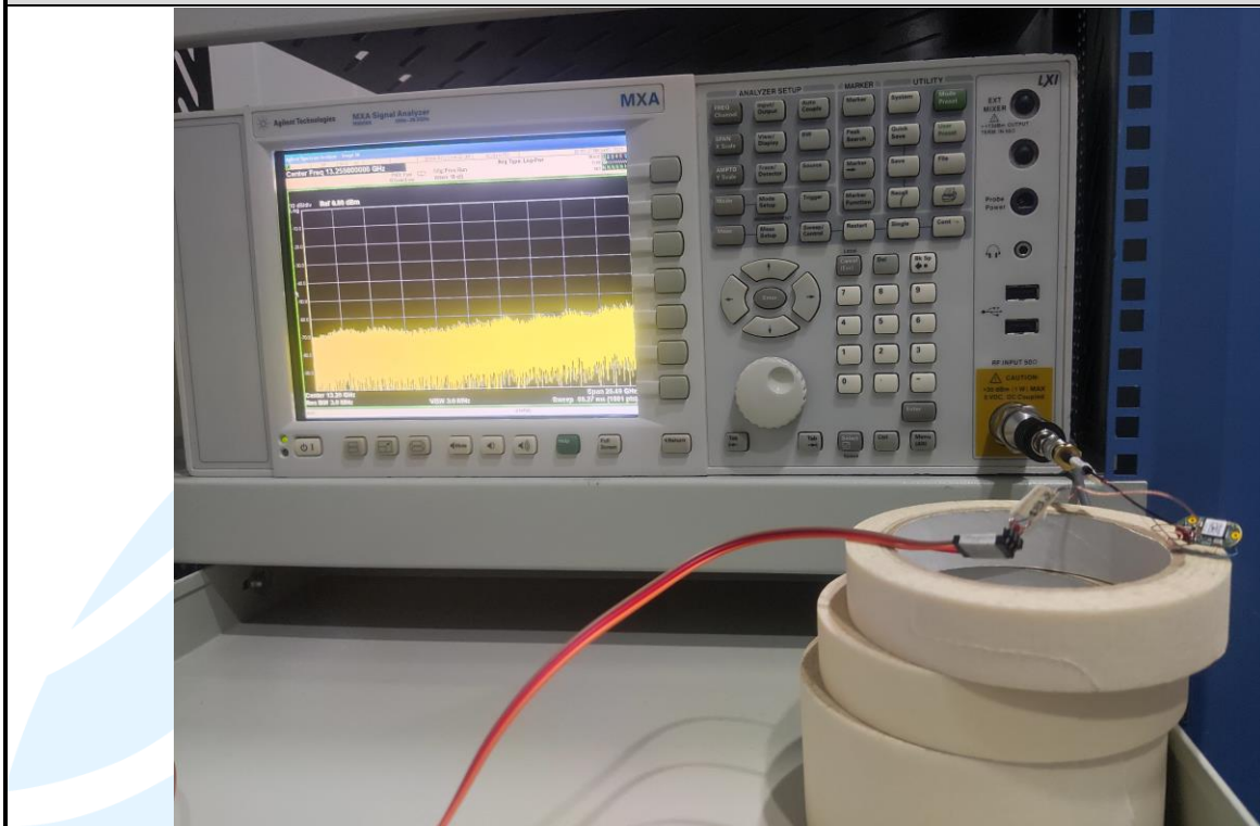
RF Conducted Test Setup_ Left Ear
