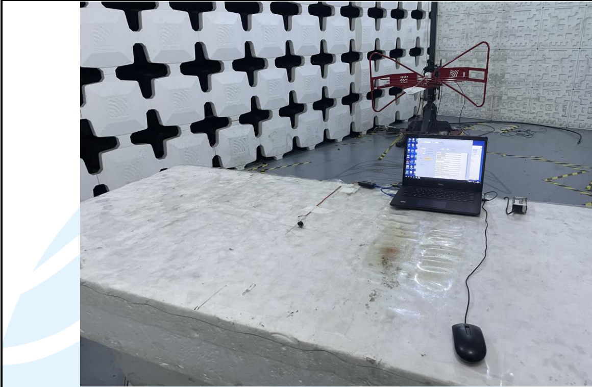
Radiated emission Test Setup (30 MHz~1 GHz)_ Left Ear
