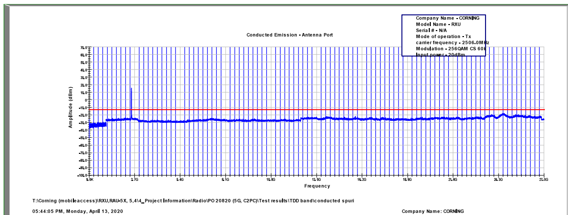
Figure 567: Spurious Emissions at Antenna Terminal 256QAM, 2506.0MHz, B.W. 20MHz, Sub Carrier 60kHz
