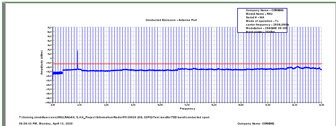
Figure 564: Spurious Emissions at Antenna Terminal 256QAM, 2506.0MHz, B.W. 20MHz, Sub Carrier 30kHz
