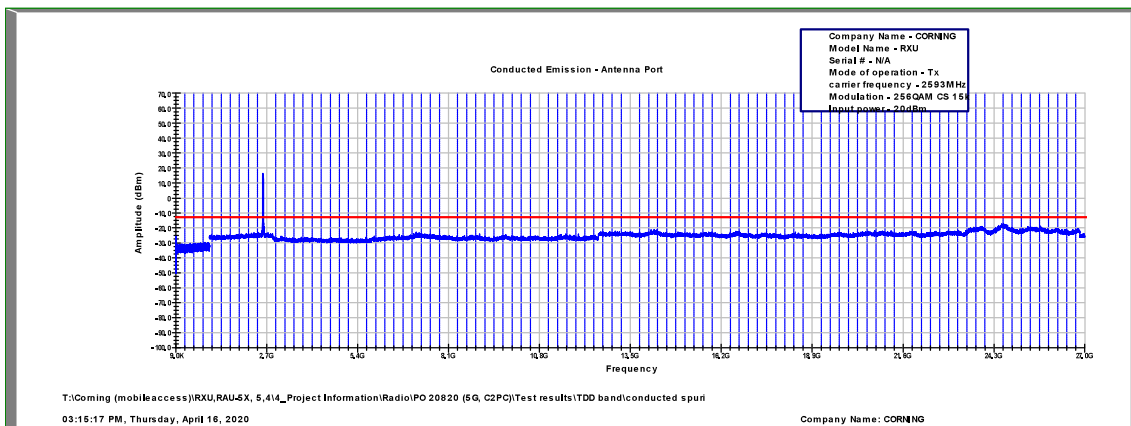
Figure 562: Spurious Emissions at Antenna Terminal 256QAM, 2593.0MHz, B.W. 20MHz, Sub Carrier 15kHz
