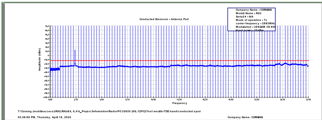
Figure 577: Spurious Emissions at Antenna Terminal 256QAM, 2593.0MHz, B.W. 40MHz, Sub Carrier 60kHz
