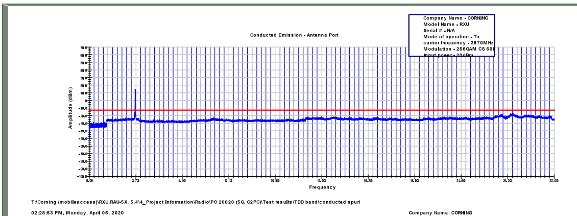
Figure 578: Spurious Emissions at Antenna Terminal 256QAM, 2670.0MHz, B.W. 40MHz, Sub Carrier 60kHz
