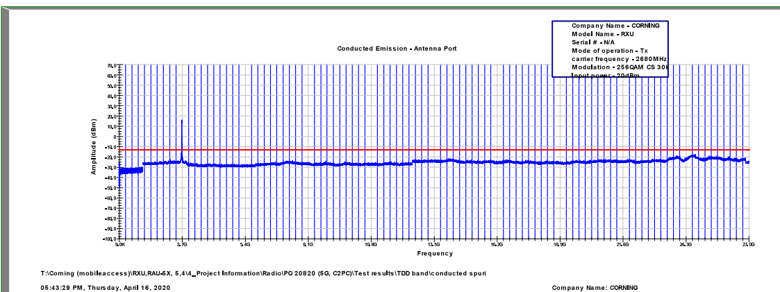
Figure 566: Spurious Emissions at Antenna Terminal 256QAM, 2680.0MHz, B.W. 20MHz, Sub Carrier 30kHz
