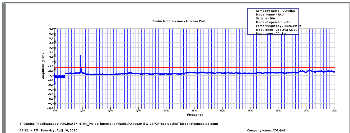
Figure 579: Spurious Emissions at Antenna Terminal 256QAM, 2526.0MHz, B.W. 60MHz, Sub Carrier 30kHz
