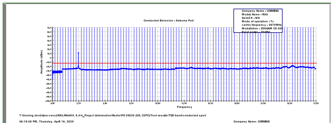
Figure 575: Spurious Emissions at Antenna Terminal 256QAM, 2670.0MHz, B.W. 40MHz, Sub Carrier 30kHz
