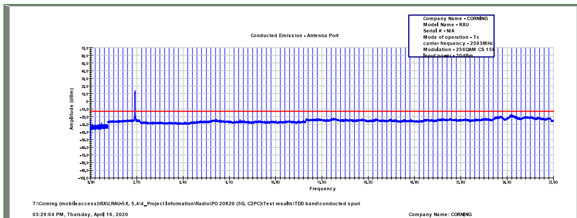
Figure 571: Spurious Emissions at Antenna Terminal 256QAM, 2593.0MHz, B.W. 40MHz, Sub Carrier 15kHz
