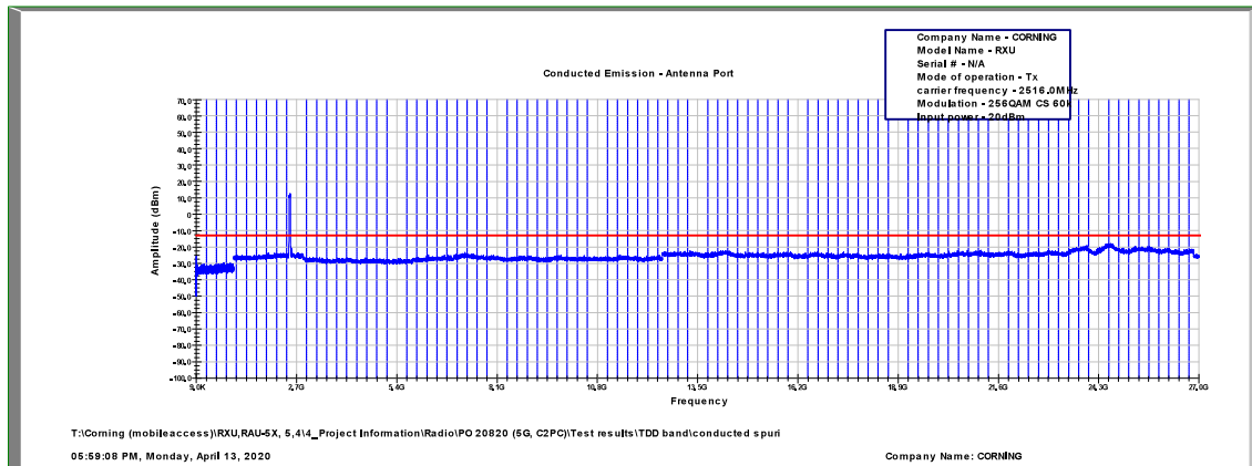
Figure 576: Spurious Emissions at Antenna Terminal 256QAM, 2516.0MHz, B.W. 40MHz, Sub Carrier 60kHz
