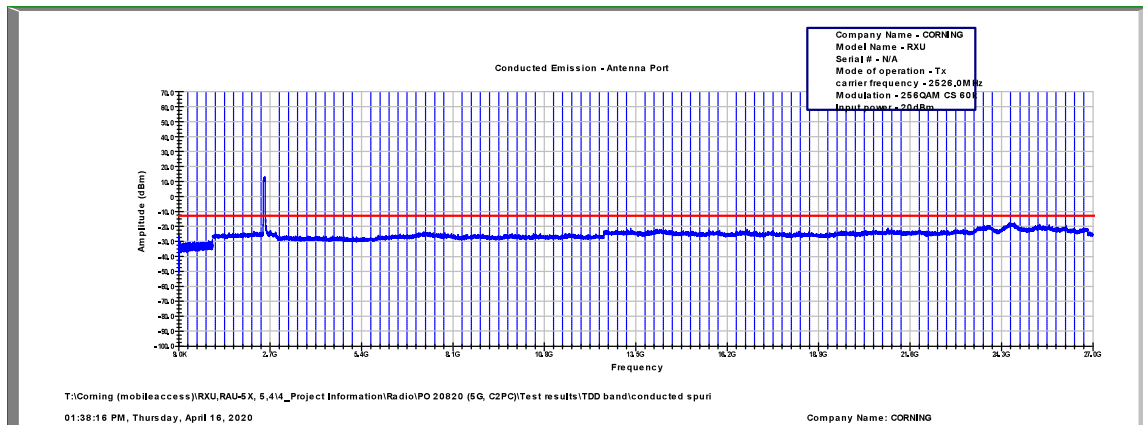
Figure 582: Spurious Emissions at Antenna Terminal 256QAM, 2526.0MHz, B.W. 60MHz, Sub Carrier 60kHz
