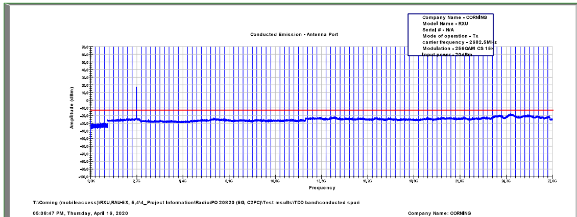
Figure 554: Spurious Emissions at Antenna Terminal 256QAM, 2682.5MHz, B.W. 15MHz, Sub Carrier 15kHz
