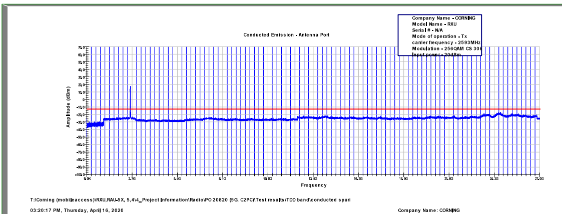
Figure 565: Spurious Emissions at Antenna Terminal 256QAM, 2593.0MHz, B.W. 20MHz, Sub Carrier 30kHz
