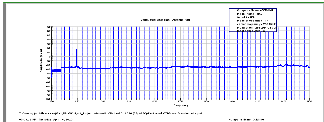
Figure 556: Spurious Emissions at Antenna Terminal 256QAM, 2593.0MHz, B.W. 15MHz, Sub Carrier 30kHz
