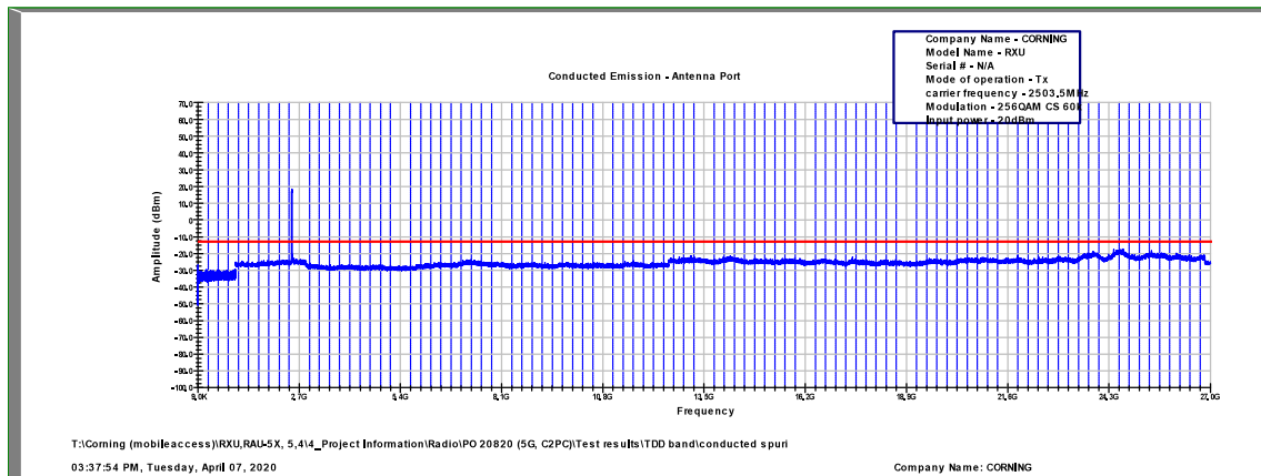
Figure 558: Spurious Emissions at Antenna Terminal 256QAM, 2503.5MHz, B.W. 15MHz, Sub Carrier 60kHz
