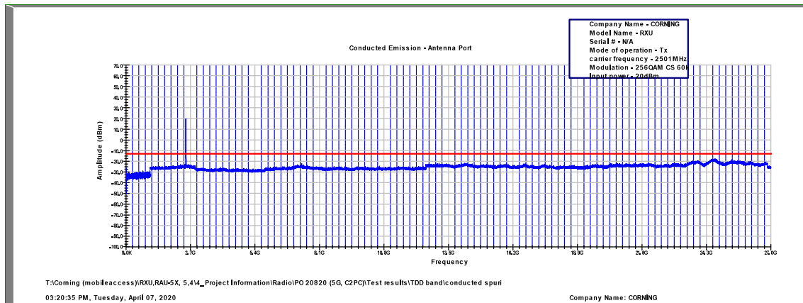
Figure 549: Spurious Emissions at Antenna Terminal 256QAM, 2501.0MHz, B.W. 10MHz, Sub Carrier 60kHz
