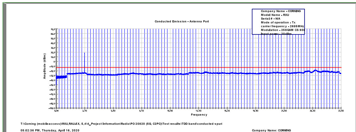
Figure 551: Spurious Emissions at Antenna Terminal 256QAM, 2685.0MHz, B.W. 10MHz, Sub Carrier 60kHz
