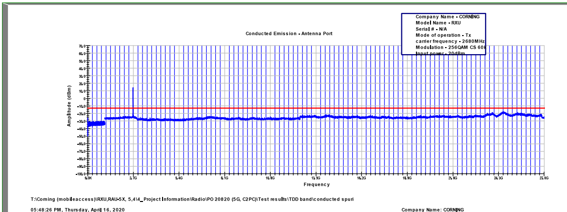
Figure 569: Spurious Emissions at Antenna Terminal 256QAM, 2680.0MHz, B.W. 20MHz, Sub Carrier 60kHz
