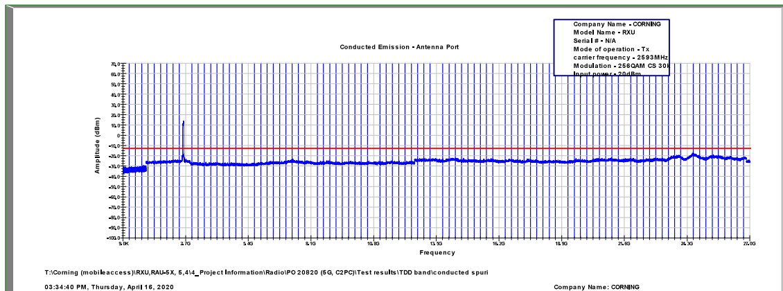
Figure 574: Spurious Emissions at Antenna Terminal 256QAM, 2593.0MHz, B.W. 40MHz, Sub Carrier 30kHz
