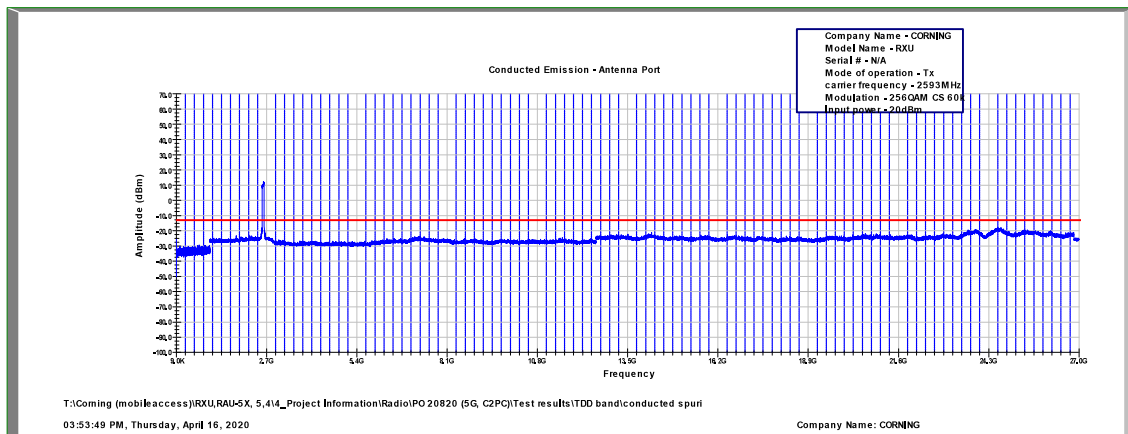
Figure 583: Spurious Emissions at Antenna Terminal 256QAM, 2593.0MHz, B.W. 60MHz, Sub Carrier 60kHz
