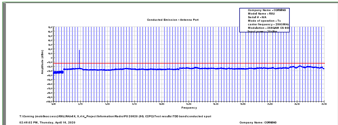
Figure 550: Spurious Emissions at Antenna Terminal 256QAM, 2593.0MHz, B.W. 10MHz, Sub Carrier 60kHz
