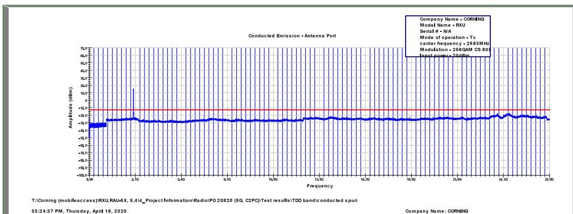
Figure 568: Spurious Emissions at Antenna Terminal 256QAM, 2593.0MHz, B.W. 20MHz, Sub Carrier 60kHz
