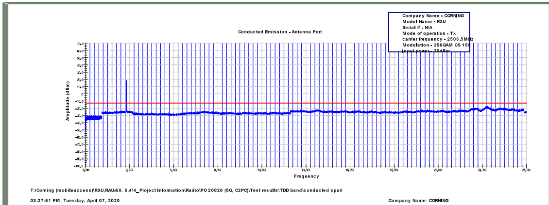
Figure 552: Spurious Emissions at Antenna Terminal 256QAM, 2503.5MHz, B.W. 15MHz, Sub Carrier 15kHz
