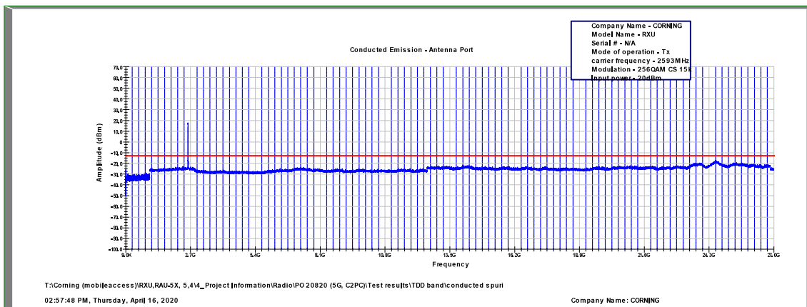
Figure 553: Spurious Emissions at Antenna Terminal 256QAM, 2593.0MHz, B.W. 15MHz, Sub Carrier 15kHz
