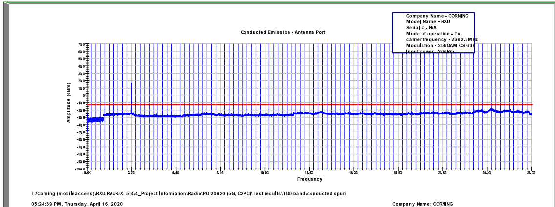
Figure 560: Spurious Emissions at Antenna Terminal 256QAM, 2682.5MHz, B.W. 15MHz, Sub Carrier 60kHz
