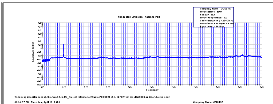
Figure 581: Spurious Emissions at Antenna Terminal 256QAM, 2660.0MHz, B.W. 60MHz, Sub Carrier 30kHz
