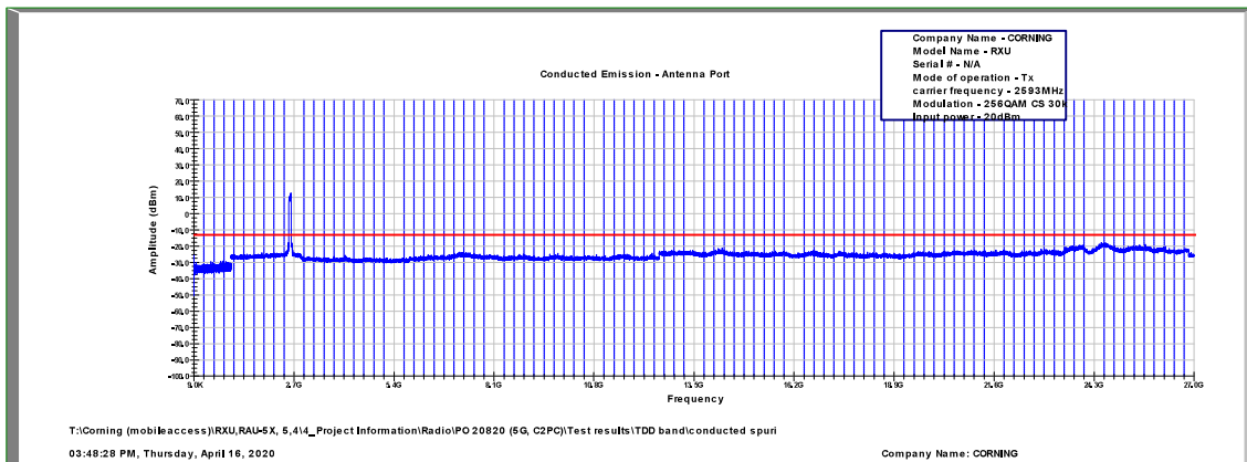
Figure 580: Spurious Emissions at Antenna Terminal 256QAM, 2593.0MHz, B.W. 60MHz, Sub Carrier 30kHz
