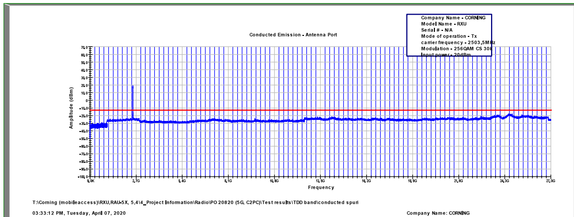
Figure 555: Spurious Emissions at Antenna Terminal 256QAM, 2503.5MHz, B.W. 15MHz, Sub Carrier 30kHz
