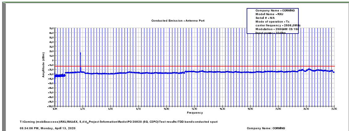
Figure 561: Spurious Emissions at Antenna Terminal 256QAM, 2506.0MHz, B.W. 20MHz, Sub Carrier 15kHz
