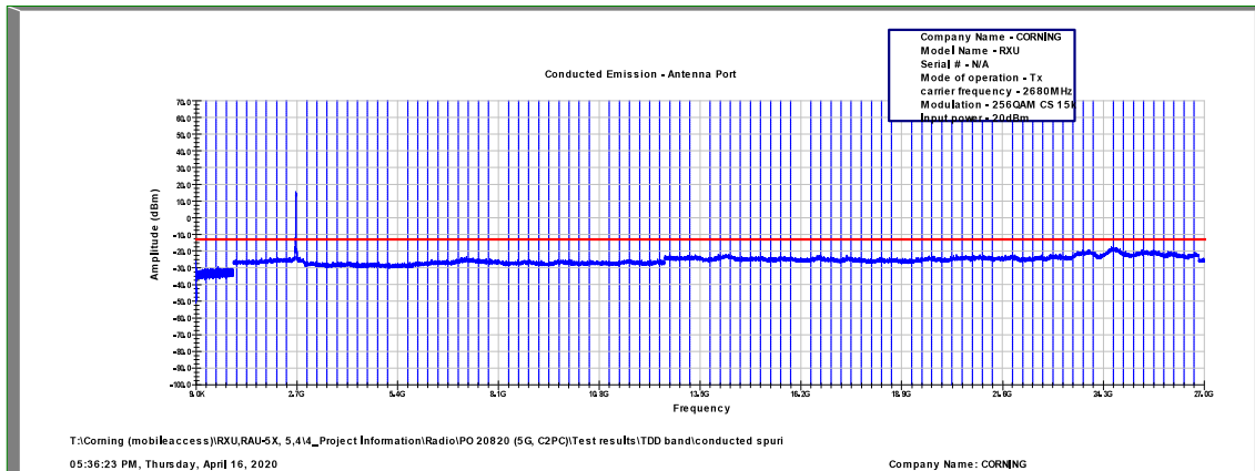
Figure 563: Spurious Emissions at Antenna Terminal 256QAM, 2680.0MHz, B.W. 20MHz, Sub Carrier 15kHz
