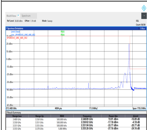
1-N78-3450-3550--30-100-H-5-CP-QPSK-Edge_1RB_Right-1@272-Ant1-1---see graph
