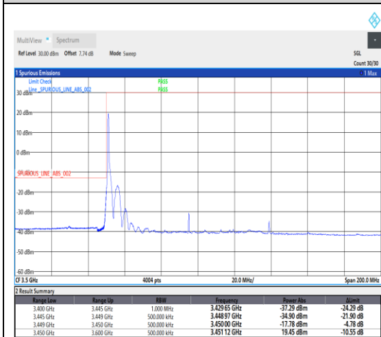
1-N78-3450-3550--30-90-L-4-CP-QPSK-Edge_1RB_Left-1@0-Ant1-1---see graph
