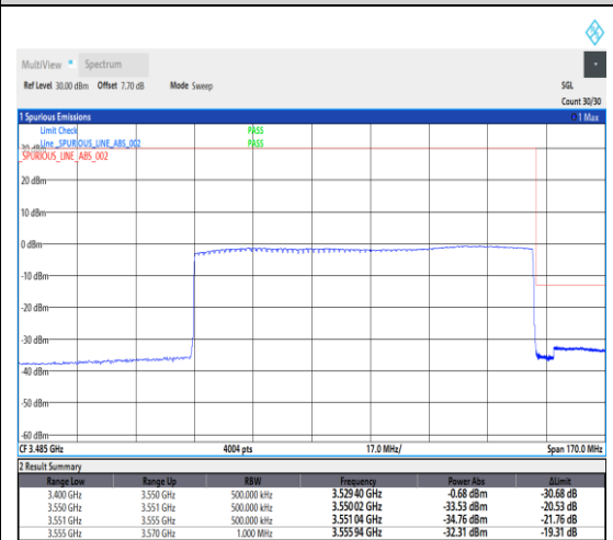
1-N78-3450-3550--30-100-H-6-CP-QPSK-Out_Full-273@0-Ant1-1---see graph
