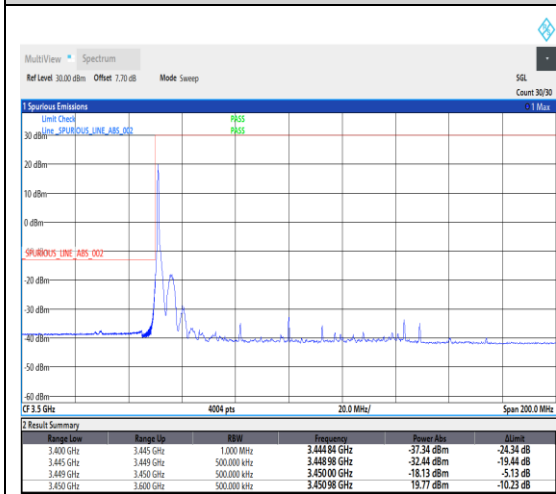
1-N78-3450-3550--30-100-L-1-DFT-PI2BPSK-Edge_1RB_Left-1@0-Ant1-1---see graph
