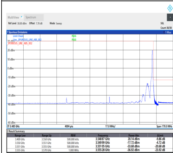
1-N78-3450-3550--30-90-H-5-CP-QPSK-Edge_1RB_Right-1@244-Ant1-1---see graph
