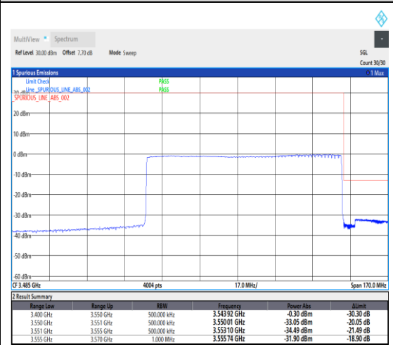
1-N78-3450-3550--30-90-H-6-CP-QPSK-Outer_Full-245@0-Ant1-1---see graph
