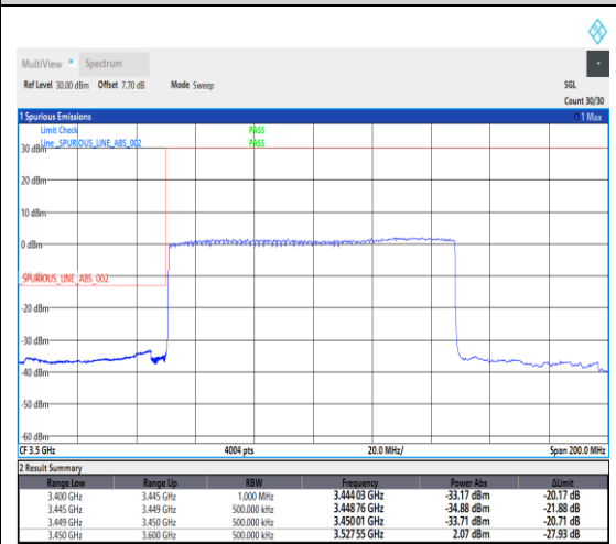
1-N78-3450-3550--30-100-L-3-DFT-PI2BPSK-Outer_Full-270@0-Ant1-1---see graph
