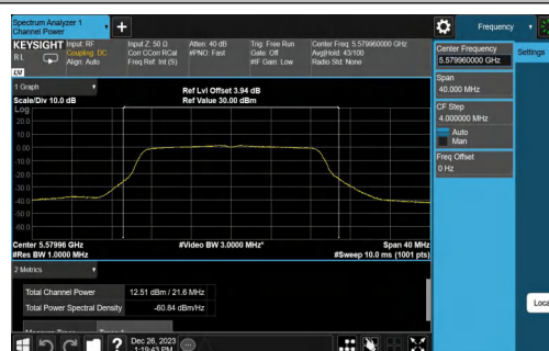
11AC20MIMO-Ant1-5580-TPC_L-PASS
