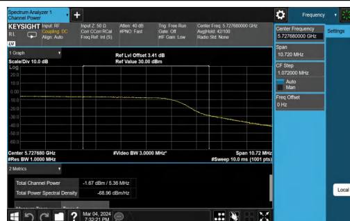
11AC20MIMO-Ant1-5745-PASS
