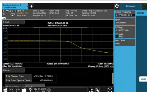
11AC20MIMO-Ant0-5745-PASS
