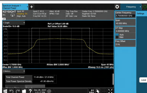
11AC20MIMO-Ant0-5700-TPC_L-PASS
