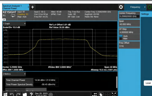
11AC20SISO-Ant0-5260-TPC_L-PASS
