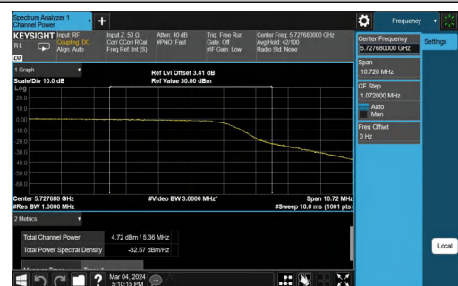
11AC20MIMO-Ant1-5720_UNII-3-TPC_L-PASS
