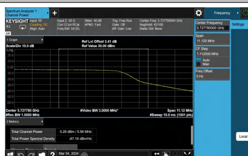
11AC20SISO-Ant1-5745-PASS
