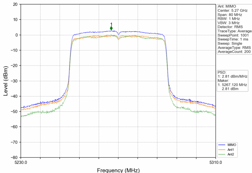
802.11ax(HEW40)_LCH_5270MHz_RU484_Left_MIMO_NTNV
