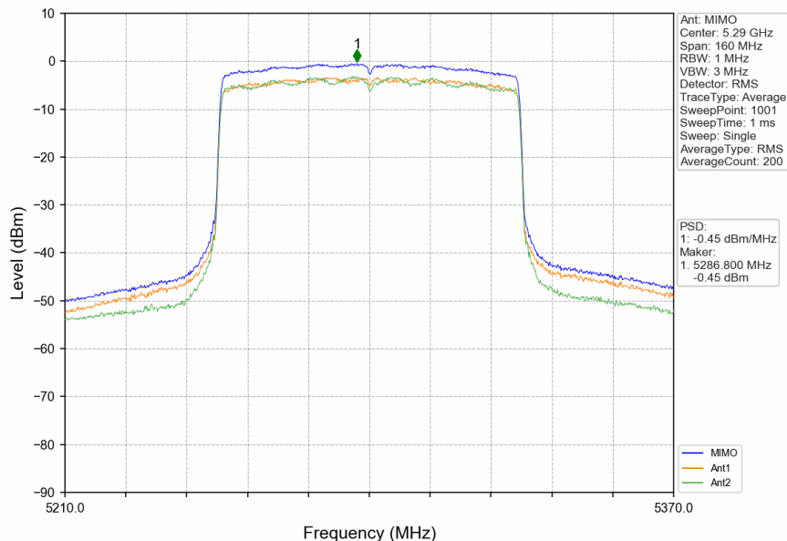
802.11ax(HEW80)_MCH_5290MHz_RU996_Left_MIMO_NTNV
