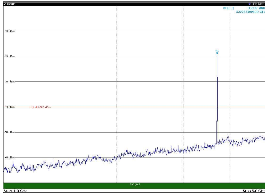
Channel: TOP, Modulation: 64QAM, BW=20MHz, Range: 1GHz - 5GHz, Polarization: Horizontal
