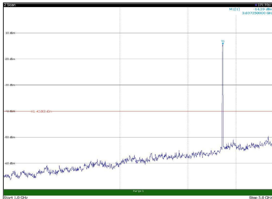
Channel: TOP, Modulation: 64QAM, BW=20MHz, Range: 1GHz - 5GHz, Polarization: Vertical
