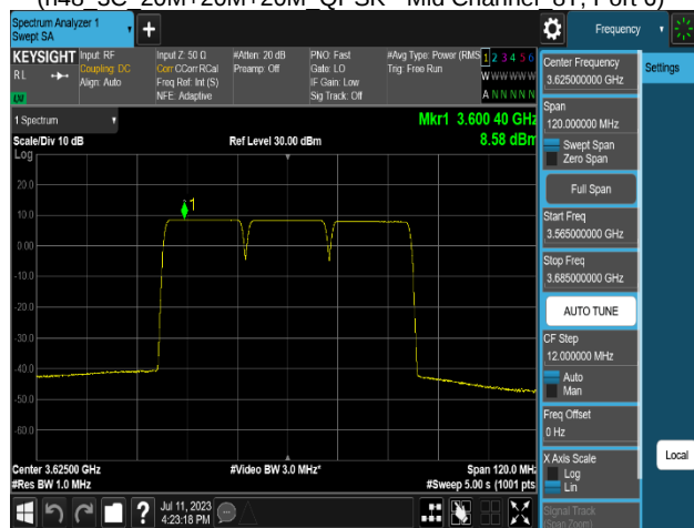
Plot 8-20. Power Spectral Density Plot (n48_3C_20M+20M+20M_QPSK - Mid Channel_8T, Port 8)
