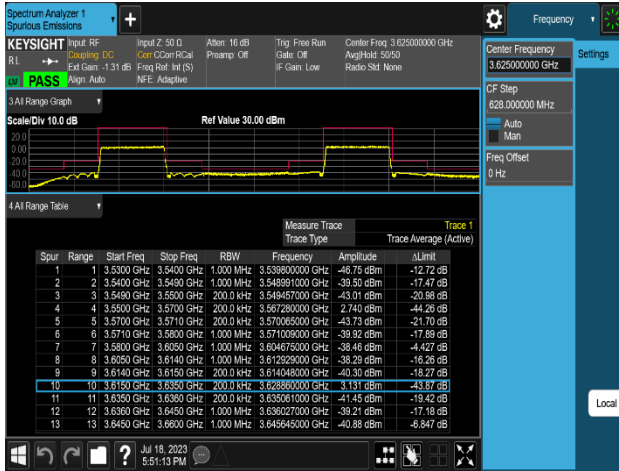
Plot 8-47. Channel Edge Emission Plot (n48_3C_20M+20M+20M_QPSK – Non-Contiguous_8T, Port 5)
