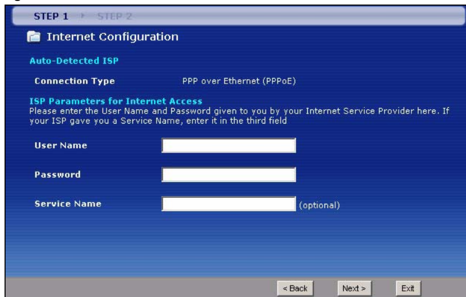
Figure 19 Auto-Detection: PPPoE
