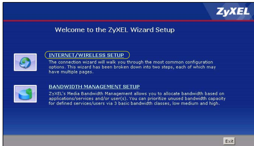
Figure 16 Wizard: Welcome
