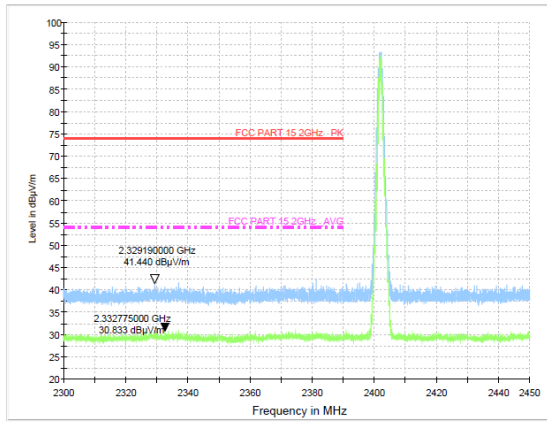
Test Mode: \pi/4 DQPSK-Low Hopping-off
