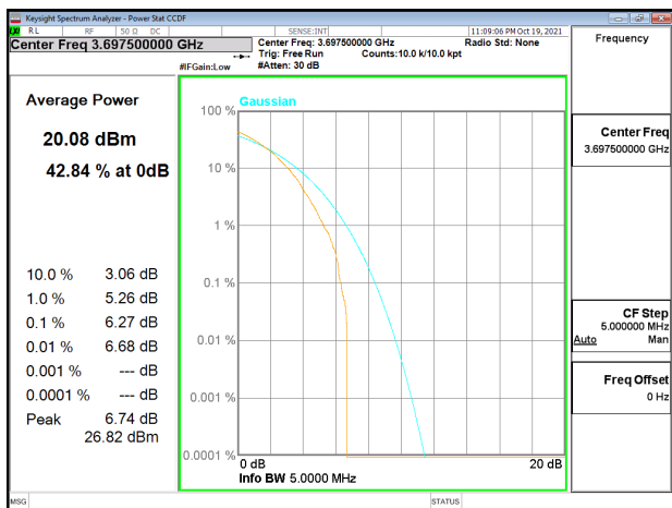
Band48_5MHz_64QAM_RB25_0_CH56715
