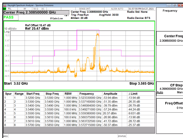
Emission Mask_Band48_10MHz_QPSK_RB1_49_CH55290
