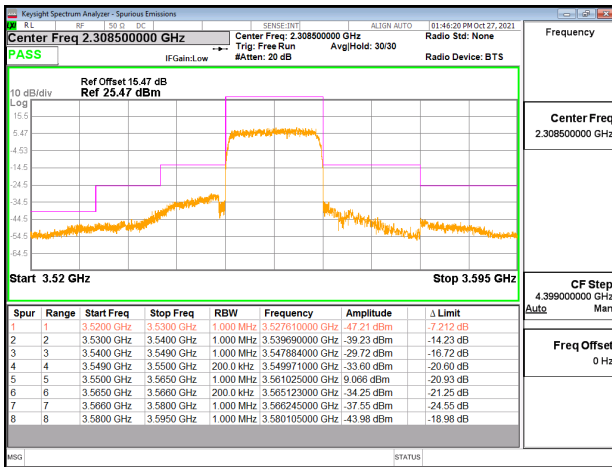
Emission Mask_Band48_15MHz_QPSK_RB75_0_CH55315
