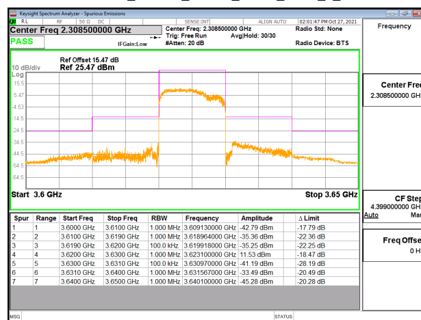
Emission Mask_Band48_10MHz_QPSK_RB50_0_CH55990
