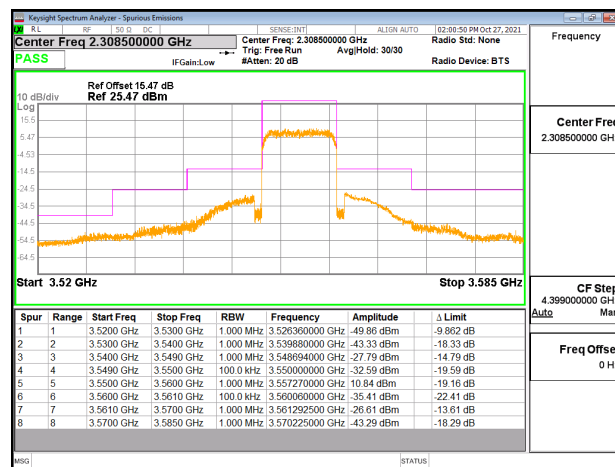
Emission Mask_Band48_10MHz_QPSK_RB50_0_CH55290
