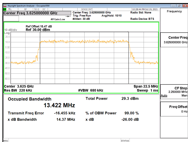
Band48_15MHz_QPSK_RB75_0_CH55990
