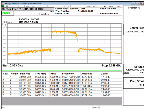
Emission Mask_Band48_15MHz_QPSK_RB75_0_CH55990
