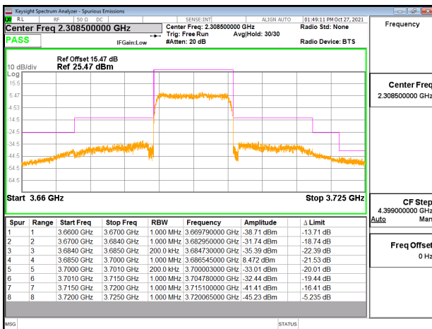
Emission Mask_Band48_15MHz_QPSK_RB75_0_CH56665
