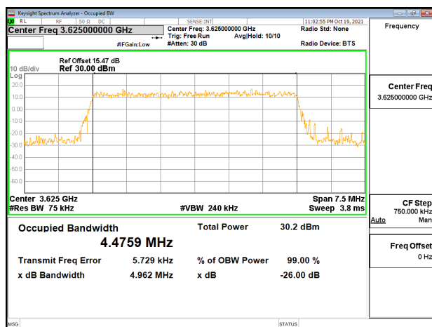
Band48_5MHz_QPSK_RB25_0_CH55990
