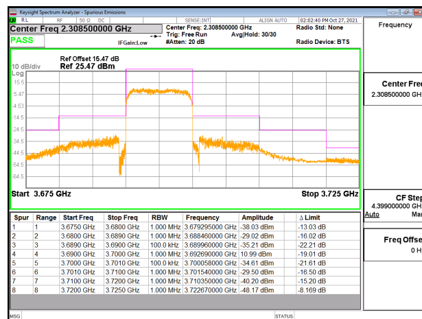
Emission Mask_Band48_10MHz_QPSK_RB50_0_CH56690
