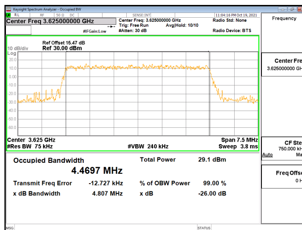
Band48_5MHz_16QAM_RB25_0_CH55990
